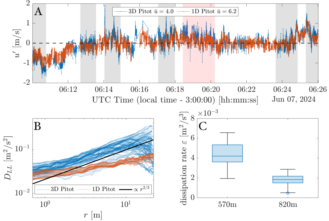
Figure 7. A: Velocity fluctuation measured with 1D (100 Hz, 8-point averaging effectively 12.5 Hz) and 3D pitot tubes (50 Hz) in a region of \approx 820 m altitude show overall agreement. Sections with continuous measurements are marked with shading. B: The second order longitudinal structure function only reveals r^{2/3} -scaling in the inertial sub-range for the measurements with 3D pitot tube. C: From the structure function the dissipation rate \varepsilon was determined for the shaded red region shown in panel A (820 m) and another region at lower altitude (570 m).
