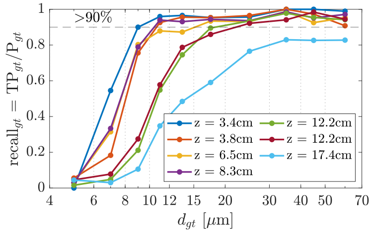
Figure 8. Recall measured with the CloudTarget as a function of the theoretical ground truth particle diameter d_{gt} . The recall is determined within the center cross section of 18.4 \times 18.4 mm. A CloudTarget photomask was recorded with HoloTrack at different z -distances from the imaging plane. The holograms were automatically processed. Recall is a measure for detection efficiency and indicates how many of the actual particles were correctly found by the system. For z \lesssim 8.5 cm particles of 10\text{ }\mu\text{m} diameter or larger are reliably detected. The results are binned by ground truth diameter d_{gt} , the diameter of the printed disks on the photomask which might vary slightly from the measured diameter d_m .
