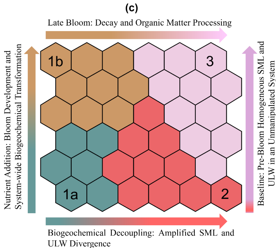
605 Figure 8: Distribution and visualisation of SML and ULW nutrient samples on the self-organising map (SOM). (a) Acronyms of individual samples are denoted by sampling month (M, May; J, June) and water layers (S, SML; U, ULW). Numbers correspond to the sampling day of the respective month. i.e. SM18 represents the SML sample on May 18, and UM18 represents the ULW sample on the same date. (b) Hierarchical clustering of the trained SOM nodes, mapped to a dendrogram. Each node on the dendrogram represent the hexagonal cells in the SOM map, i.e. 1 corresponds to neuron 1 in cluster 1. Neuron clustering or counting proceeds from bottom to top and from left to right on the SOM map in panel (a). Different colors and corresponding numbers delineate clusters. (c) Clusters from panel (a) are shown again, illustrating temporal and seasonal variability in SML and ULW nutrient samples. This panel complements panel (a) by presenting the same SOM cluster classification with text labels for easier interpretation, highlighting the temporal progression of the mesocosm experiment and how clusters change across different bloom phases based on nutrient fluctuations and levels over the time of the mesocosm. 610
