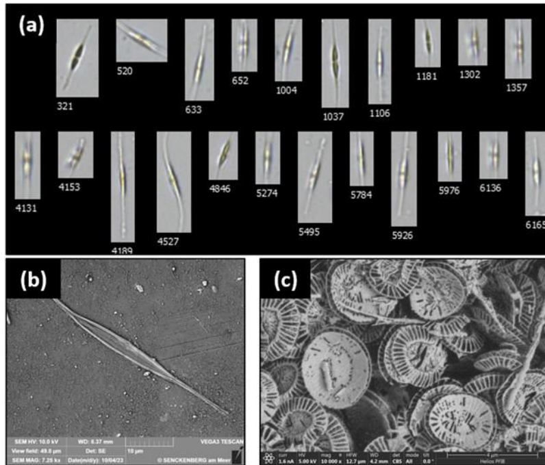
Figure R1. Bloom-forming species observed during the mesocosm experiment. (a) FlowCam images of Cylindrotheca closterium (numbers indicate image identifiers). (b) SEM image of C. closterium . (c) SEM image of coccoliths belonging to Emiliana huxleyi .
