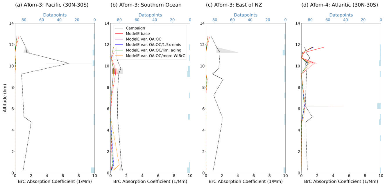
00 Figure 11. Vertical profiles of median BrC absorption (BrC-Abs) at 365 nm, measured by flight campaigns (black) and simulated by ModelE's base case of BrC representation (red), variable OA-to-OC ratio case (purple), 1.5 times BB OA emissions case (blue), limited aging case (green), and larger fraction of WBrC case (orange). Analysis is over remote regions, and data is in units of \text{Mm}^{-1} . Consistent with Fig. 7, a CO and BC scaling factor (Eqs. 1-2) have been applied to model data, campaign and specific region of analysis is indicated on the top left of each plot, the midpoint of altitude bins is plotted, dashed lines interpolate over altitudes with no data, shaded areas show 05 the IQR of BrC-Abs in each altitude bin, blue bars show the number of datapoints averaged in each bin, and horizontal blue dashed-lines separate the lower-, mid-, and upper-troposphere. Data is not filtered for BB number fraction.
