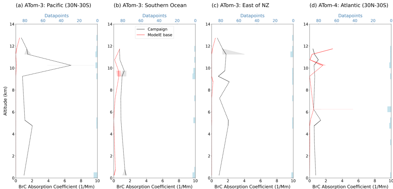
30 Figure 7. Vertical profiles of median BrC absorption (BrC-Abs) at 365 nm, measured by flight campaigns (black) and simulated by (red), in remote regions, reported in units of \text{Mm}^{-1} . Consistent with Fig. 6, a CO and BC scaling factor (Eqs. 1-2) have been applied to model data, campaign and specific region of analysis is indicated on the top left of each plot, the midpoint of each altitude bin is plotted, dashed lines interpolate over altitudes with no data, shaded areas show the IQR of BrC-Abs in each altitude bin, blue bars show the number of 35 datapoints grouped in each bin, and horizontal blue dashed-lines separate the lower-, mid-, and upper-troposphere. Data is not filtered for BB number fraction.
