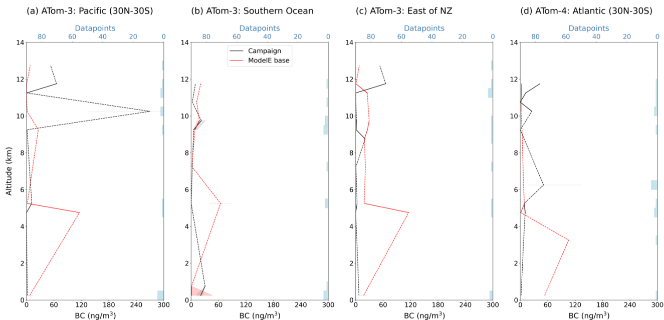
50 Figure 4. Vertical profiles of median BC mass concentration, measured by flight campaigns (black) and simulated by ModelE’s base case of BrC representation (red), in remote regions, reported in units of \text{ng m}^{-3} . Consistent with Fig. 3, a CO scaling factor (Eq. 1) has been applied to model data, the midpoint of altitude bins is plotted, campaign and specific region of analysis is indicated on the top left of each plot, dashed lines interpolate over altitudes with no data, shaded areas show the IQR of BC in each altitude bin, blue bars show the number of datapoints grouped in each bin, and horizontal blue dashed-lines separate the lower-, mid-, and upper-troposphere. Unlike Fig. 3, there is no BB number fraction filter applied, as data is already limited.
