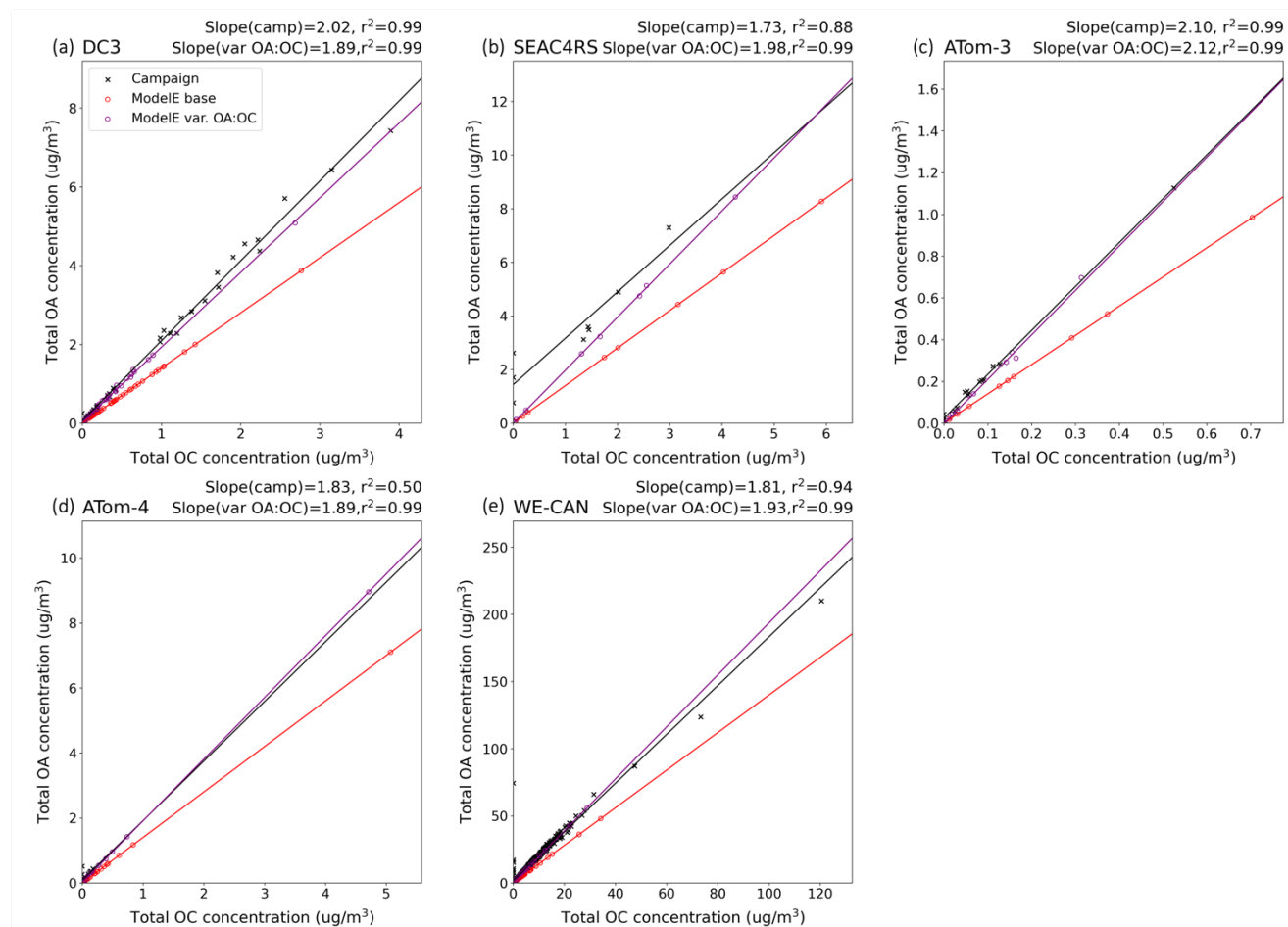
25 Figure 9. Total OA concentration plotted against OC concentration, both in units of \mu\text{g m}^{-3} , as measured by flight campaigns (black x's), simulated by the base case of ModelE OA representation (red o's), and simulated by the revised ModelE case with variable OA-to-OC
