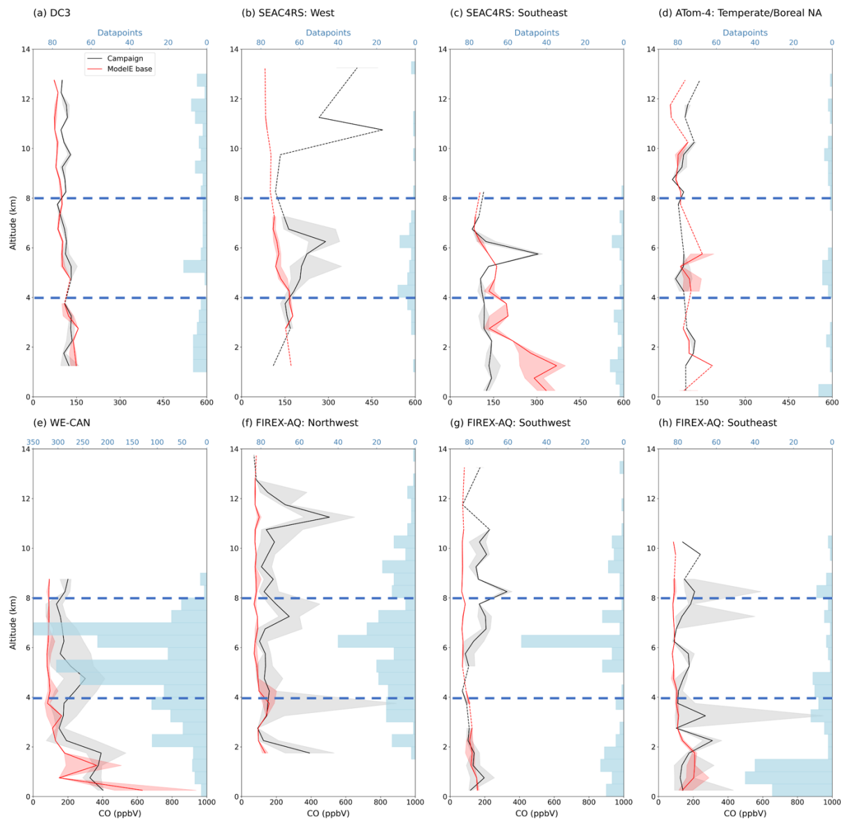
Figure A2. Vertical profiles of median carbon monoxide (CO) concentration measured by flight campaigns (black) and simulated by ModelE's base case of BrC representation (red), over land/near sources, reported in units of ppbV. Campaign and specific region of analysis is indicated on the top left of each plot, data is plotted at the midpoint of each altitude bin, dashed lines interpolate over altitudes with no data, shaded areas show the interquartile range (IQR) of data in each altitude bin, blue bars show the number of datapoints grouped in each bin, and horizontal blue dashed-lines separate the lower-, mid-, and upper-troposphere. Data is filtered for BB number fraction (when relevant).
