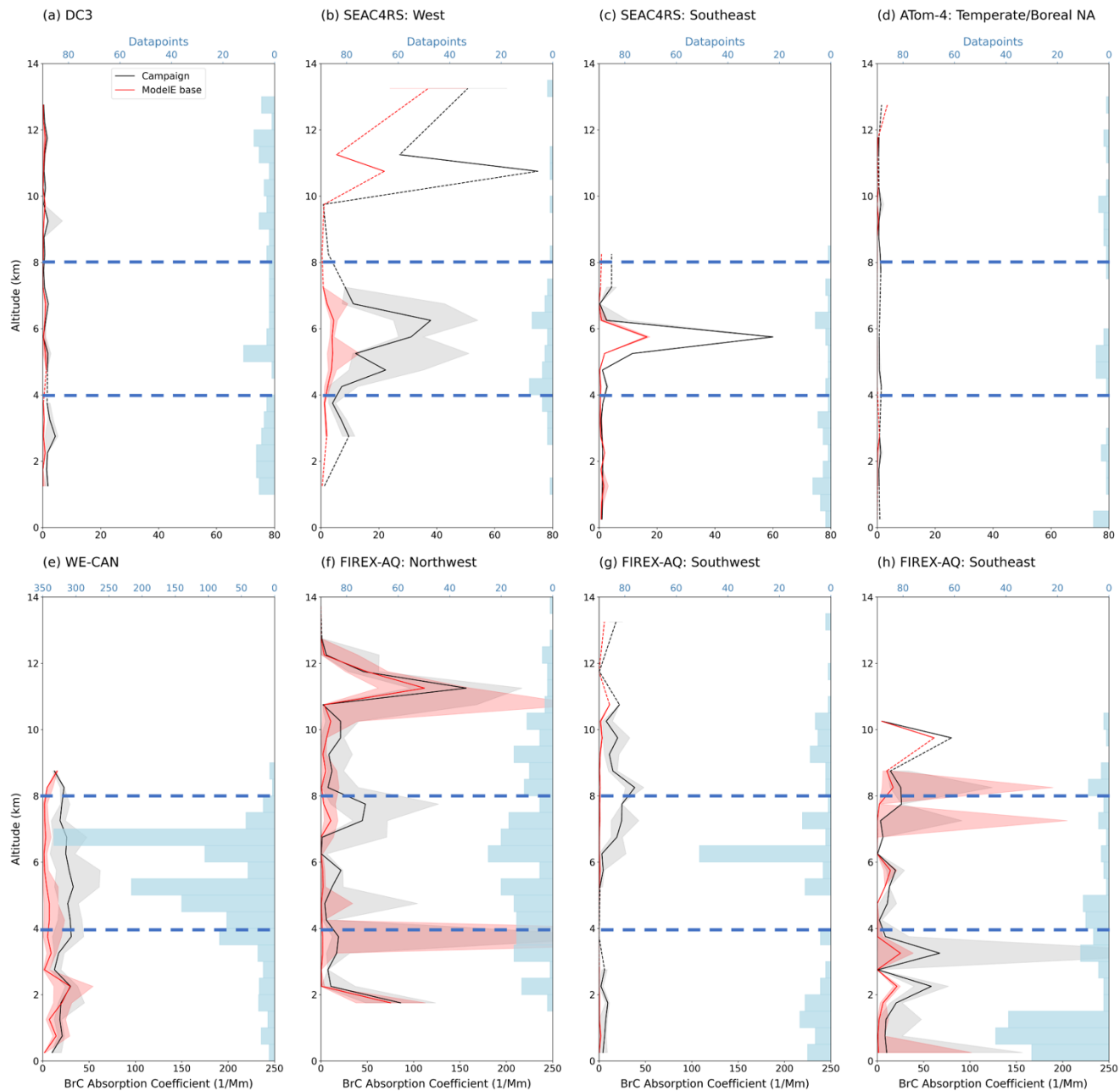
Figure 6. Vertical profiles of median BrC absorption (BrC-Abs) at 365 nm, measured by flight campaigns (black) and simulated by ModelE's base case of BrC representation (red), over land/near sources, reported in units of \text{Mm}^{-1} . Model absorption has been multiplied by a CO and BC scaling factor (Eqs. 1-2). Consistent with Figs. 3 and 4, campaign and specific region of analysis is indicated on the top left of each plot, the midpoint of altitude bins in plotted, dashed lines interpolate over altitudes with no data, shaded areas show the IQR of
