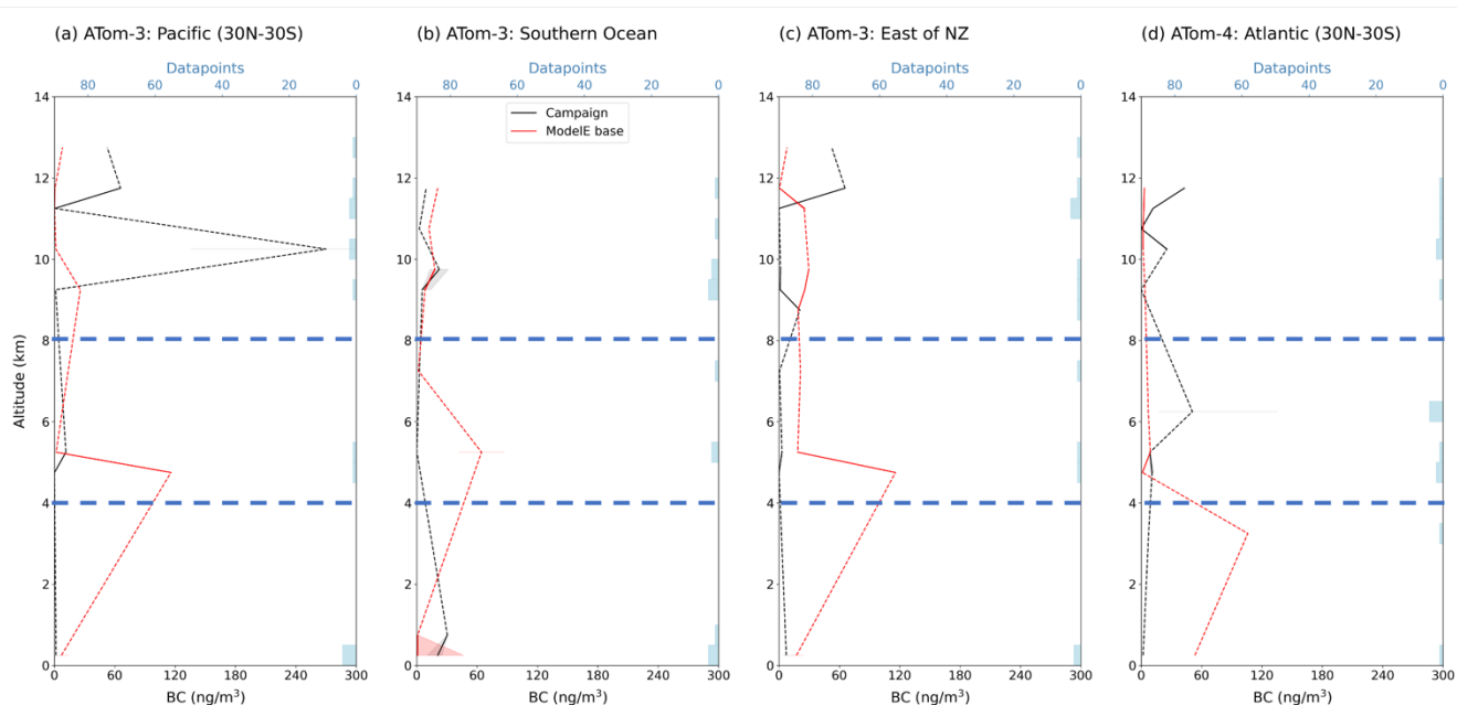
Figure 4. Vertical profiles of median BC mass concentration, measured by flight campaigns (black) and simulated by ModelE’s base case of BrC representation (red), in remote regions, reported in units of \text{ng m}^{-3} . Consistent with Fig. 3, a CO scaling factor (Eq. 1) has been applied to model data, the midpoint of altitude bins is plotted, campaign and specific region of analysis is indicated on the top left of each plot, dashed lines interpolate over altitudes with no data, shaded areas show the IQR of BC in each altitude bin, blue bars show the number of datapoints grouped in each bin, and horizontal blue dashed-lines separate the lower-, mid-, and upper-troposphere. Unlike Fig. 3, there is no BB number fraction filter applied, as data is already limited. 50
