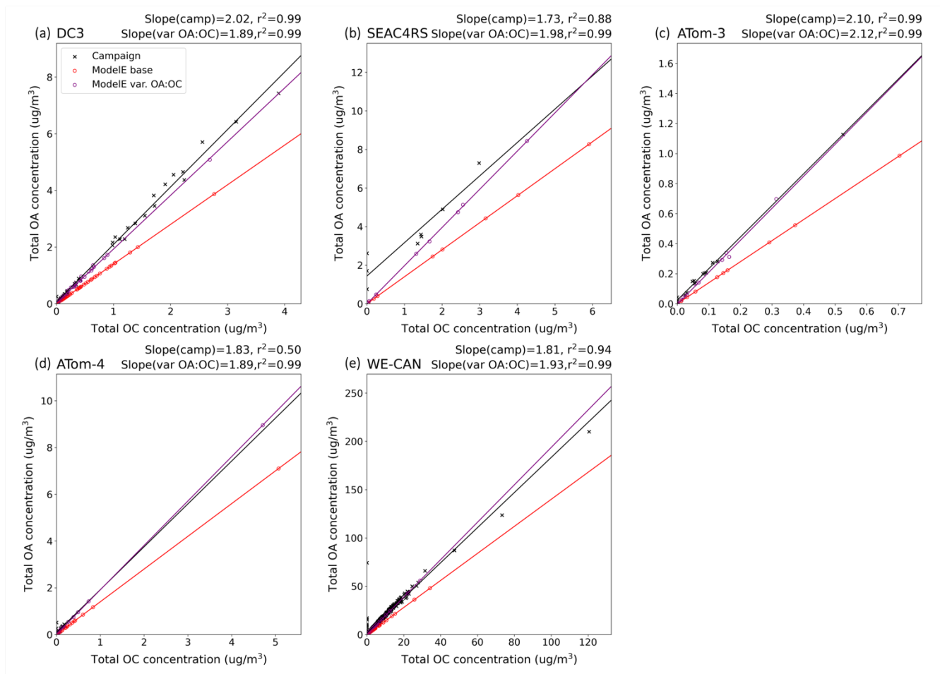
20 Figure 9. Total OA concentration plotted against OC concentration, both in units of \mu\text{g m}^{-3} , as measured by flight campaigns (black x's), simulated by the base case of ModelE OA representation (red o's), and simulated by the revised ModelE case with variable OA-to-OC ratios (purple o's). For each campaign that provided both OC and OA measurements (labelled on the top-left of each plot), data has been filtered to remove points outside of the regions used for vertical profile analysis and points outside of the IQR (for comparison with vertical profiles). Linear regression lines for campaign data and all model simulations are included. The slope and r^2 of campaign and revised-case regressions are displayed on the top-right of each plot for comparison—these slopes are indicative of average OA-to-OC ratios. The slope and r^2 of the model base case is not provided because the value (1.4) is constant across all campaign periods and regions.
