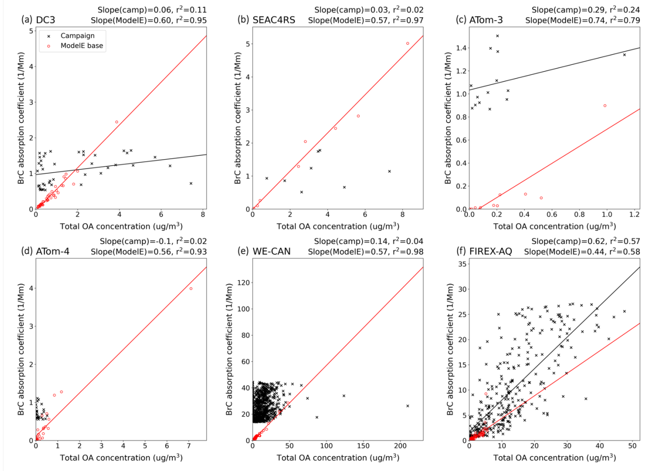
Figure 8. BrC absorption coefficient, in units of \text{Mm}^{-1} , plotted against total OA concentration, in units of \mu\text{g m}^{-3} , as measured by flight campaigns (black 'x's) and simulated by ModelE (red 'o's). For each campaign (labelled on the top-left of each plot), data has been filtered to remove points outside of the regions used for vertical profile analysis and points outside the IQR (for consistent comparison with vertical profiles). The slope and r^2 of linear regressions for measured and simulated data are displayed on the top-right of each plot. Regression lines are plotted for all campaigns except SEAC 4 RS, ATom-4, and WE-CAN (as the r^2 is too low).
