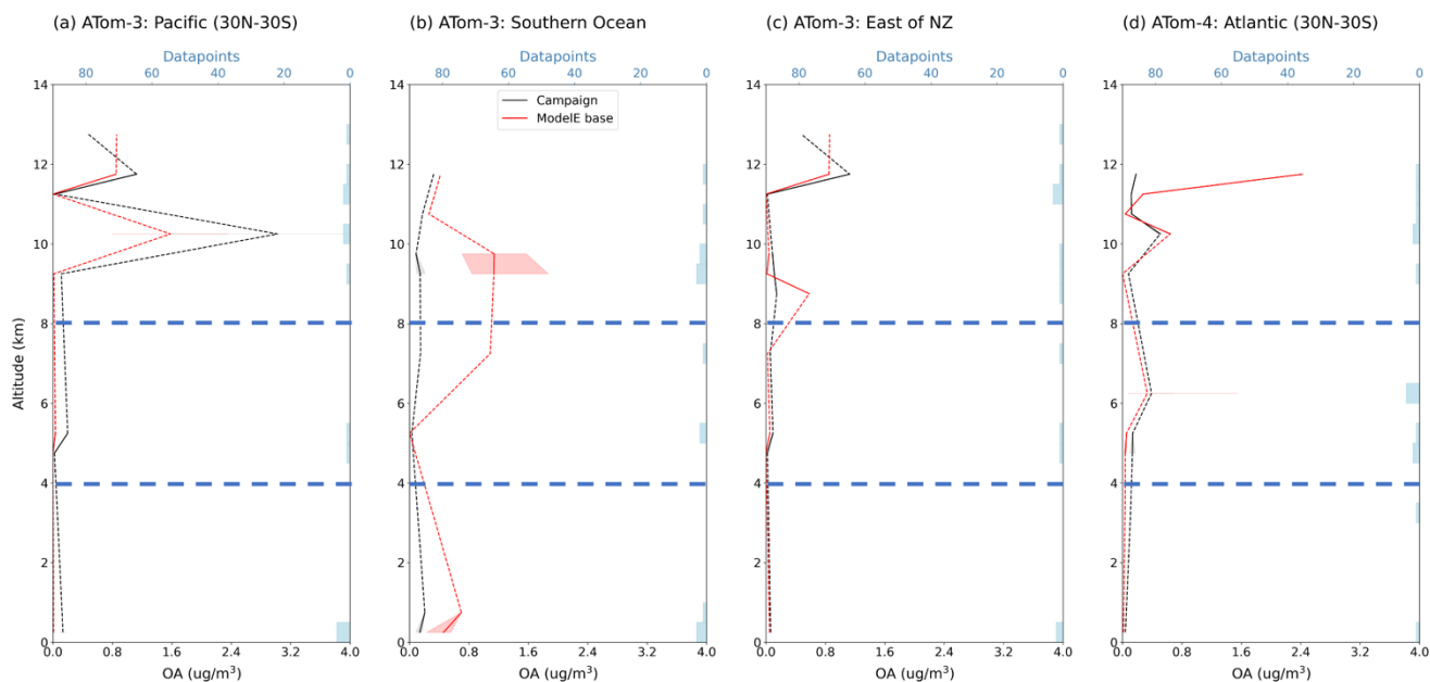
Figure A5. Vertical profiles of median, total organic aerosol (OA) concentration measured by flight campaigns (black) and simulated by ModelE’s base case of BrC representation (red), over remote regions, reported in units of \mu\text{g m}^{-3} . Consistent with Fig. A3, a CO and BC scaling factor (Eqs. 1-2) have been applied to model data, campaign and specific region of analysis is indicated on the top left of each plot, the midpoint of altitude bins is plotted, dashed lines interpolate over altitudes with no data, shaded areas show the IQR of data in each altitude bin, blue bars show the number of datapoints grouped in each bin, and horizontal blue dashed-lines separate the lower-, mid-, and upper-troposphere. Data is not filtered for BB number fraction.
