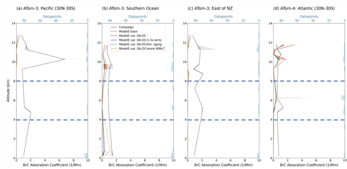
85 Figure 11. Vertical profiles of median BrC absorption (BrC-Abs) at 365 nm, measured by flight campaigns (black) and simulated by ModelE's base case of BrC representation (red), variable OA-to-OC ratio case (purple), 1.5 times BB OA emissions case (blue), limited aging case (green), and larger fraction of WBrC case (orange). Analysis is over remote regions, and data is in units of \text{Mm}^{-1} . Consistent with Fig. 7, a CO and BC scaling factor (Eqs. 1-2) have been applied to model data, campaign and specific region of analysis is indicated on the top left of each plot, the midpoint of altitude bins is plotted, dashed lines interpolate over altitudes with no data, shaded areas show the IQR of BrC-Abs in each altitude bin, blue bars show the number of datapoints averaged in each bin, and horizontal blue dashed-lines 90 separate the lower-, mid-, and upper-troposphere. Data is not filtered for BB number fraction.
