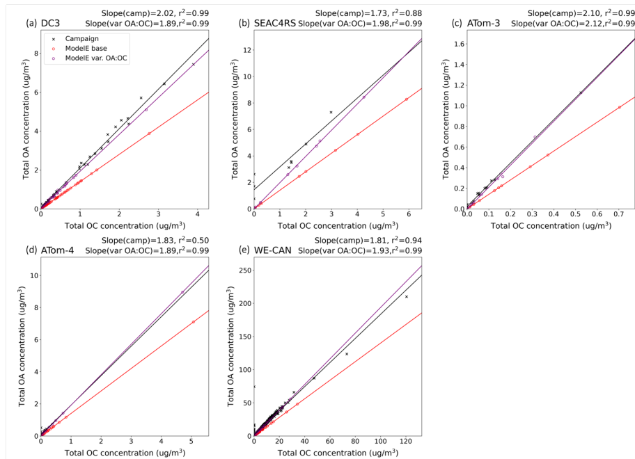
Figure 9. Total OA concentration plotted against OC concentration, both in units of \mu\text{g m}^{-3} , as measured by flight campaigns (black 'x's), simulated by the base case of ModelE OA representation (red 'o's), and simulated by the revised ModelE case with variable OA-to-OC ratios (purple 'o's').
