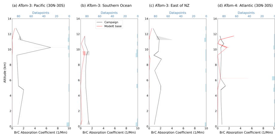
40 Figure 7. Vertical profiles of median BrC absorption (BrC-Abs) at 365 nm, measured by flight campaigns (black) and simulated by (red), in remote regions, reported in units of Mm^{-1} . Consistent with Fig. 6, a CO and BC scaling factor (Eqs. 1-2) have been applied to model data, campaign and specific region of analysis is indicated on the top left of each plot, the midpoint of each altitude bin is plotted, dashed lines interpolate over altitudes with no data, shaded areas show the IQR of BrC-Abs in each altitude bin, blue bars show the number of datapoints grouped in each bin, and horizontal blue dashed-lines separate the lower-, mid-, and upper-troposphere. Data is not filtered for BB number fraction.
