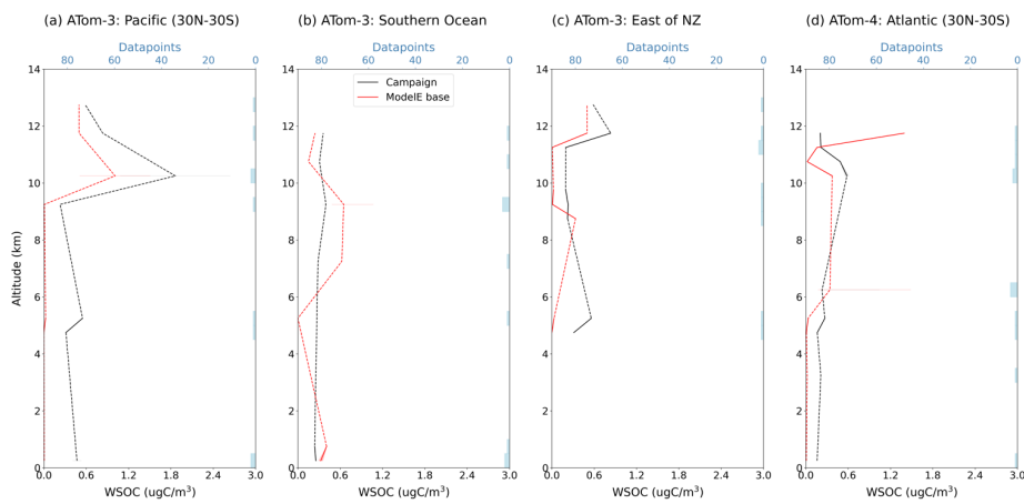
Figure A7. Vertical profiles of median water-soluble organic carbon (WSOC) concentration measured by flight campaigns (black) and simulated by ModelIE's base case of BrC representation (red), over remote regions, reported in units of \mu\text{gC m}^{-3} . Consistent with Figs. A4, a CO and BC scaling factor (Eqs. 1-2) have been applied to model data, campaign and specific region of analysis is indicated on the top left of each plot, the midpoint of altitude bins is plotted, dashed lines interpolate over altitudes with no data, shaded areas show the IQR of data in each altitude bin, blue bars show the number of datapoints grouped in each bin, and horizontal blue dashed-lines separate the lower-, mid-, and upper-troposphere. Data is not filtered for BB number fraction.
