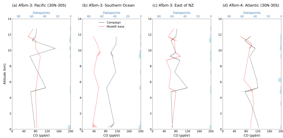
Figure A3. Vertical profiles of median carbon monoxide (CO) concentration measured by flight campaigns (black) and simulated by ModelE's base case of BrC representation (red), over remote regions, reported in units of ppbV. Consistent with Fig. A1, campaign and specific region of analysis is indicated on the top left of each plot, the midpoint of altitude bins is plotted, dashed lines interpolate over altitudes with no data, shaded areas show IQR of data in each altitude bin, blue bars show the number of datapoints grouped in each bin, and horizontal blue dashed-lines separate the lower-, mid-, and upper-troposphere. Data is not filtered for BB number fraction.
