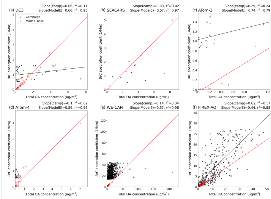
Figure 8. BrC absorption coefficient, in units of \text{Mm}^{-1} , plotted against total OA concentration, in units of \mu\text{g m}^{-3} , as measured by flight campaigns (black x's) and simulated by ModelE (red o's). For each campaign (labelled on the top-left of each plot), data has been filtered to remove points outside of the regions used for vertical profile analysis and points outside the IQR (for consistent comparison with vertical profiles). The slope and r^2 of linear regressions for measured and simulated data are displayed on the top-right of each plot. Regression lines are plotted for all campaigns except SEAC 4 RS, ATom-4, and WE-CAN (as the r^2 is too low).
