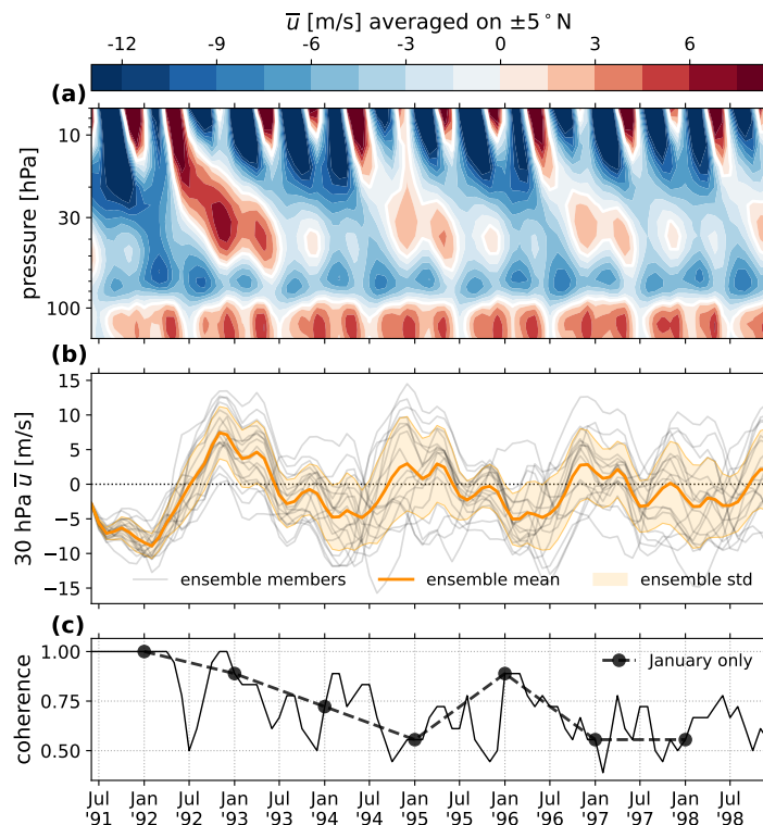
Figure 2. The QBO shown as \bar{u} averaged over [5^{\circ}\text{S}, 5^{\circ}\text{N}] for the CF ensemble mean. (a) time–pressure plane centered on the lower stratosphere. (b) zonal wind time series at 30 hPa. The ensemble mean and standard deviation in \bar{u} is shown as a bold orange line and light orange shading, respectively. Individual ensemble members are shown as faint gray lines, and the zero-line is dotted. (c) the ensemble coherence, defined as the fraction of ensemble members in agreement with the sign of the ensemble mean in panel (b). A bold dashed line with points displays the coherence evaluated only at each January.
