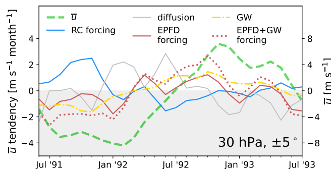
Figure 3. The TEM momentum balance of the QBO for the first two years of the CF ensemble mean, averaged over [5^\circ\text{S}, 5^\circ\text{N}] at 30 hPa. Shown are the contributions to \partial\bar{u}/\partial t in [\text{m s}^{-1} \text{ month}^{-1}] from the EPFD (red solid), gravity waves (gold dotted), the combined EPFD and gravity waves (red dotted), the residual circulation (blue solid), and diffusion (thin gray solid) as functions of latitude at 3 hPa (top panels) and 30 hPa (bottom panels). Also shown is \bar{u} itself (thick green dashed) in [\text{m s}^{-1}] , values read on the left vertical axis. The negative tendency or wind speed domain is shaded in light gray.
