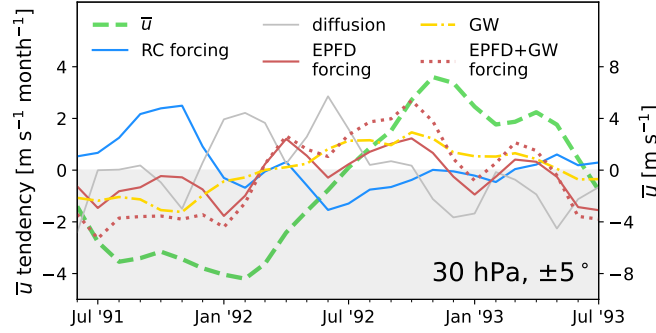
Figure 3. The TEM momentum balance of the QBO for the first two years of the CF ensemble mean, averaged over [5^{\circ}\text{S}, 5^{\circ}\text{N}] at 30 hPa. Shown are the contributions to \partial\bar{u}/\partial t in [\text{m s}^{-1} \text{ month}^{-1}] from the EPFD (red solid), gravity waves (gold dotted), the combined EPFD and gravity waves (red dotted), the residual circulation (blue solid), and diffusion (thin gray solid) as functions of latitude at 3 hPa (top panels) and 30 hPa (bottom panels). Also shown is \bar{u} itself (thick green dashed) in [\text{m s}^{-1}] , values read on the left vertical axis. The negative tendency or wind speed domain is shaded in light gray.
