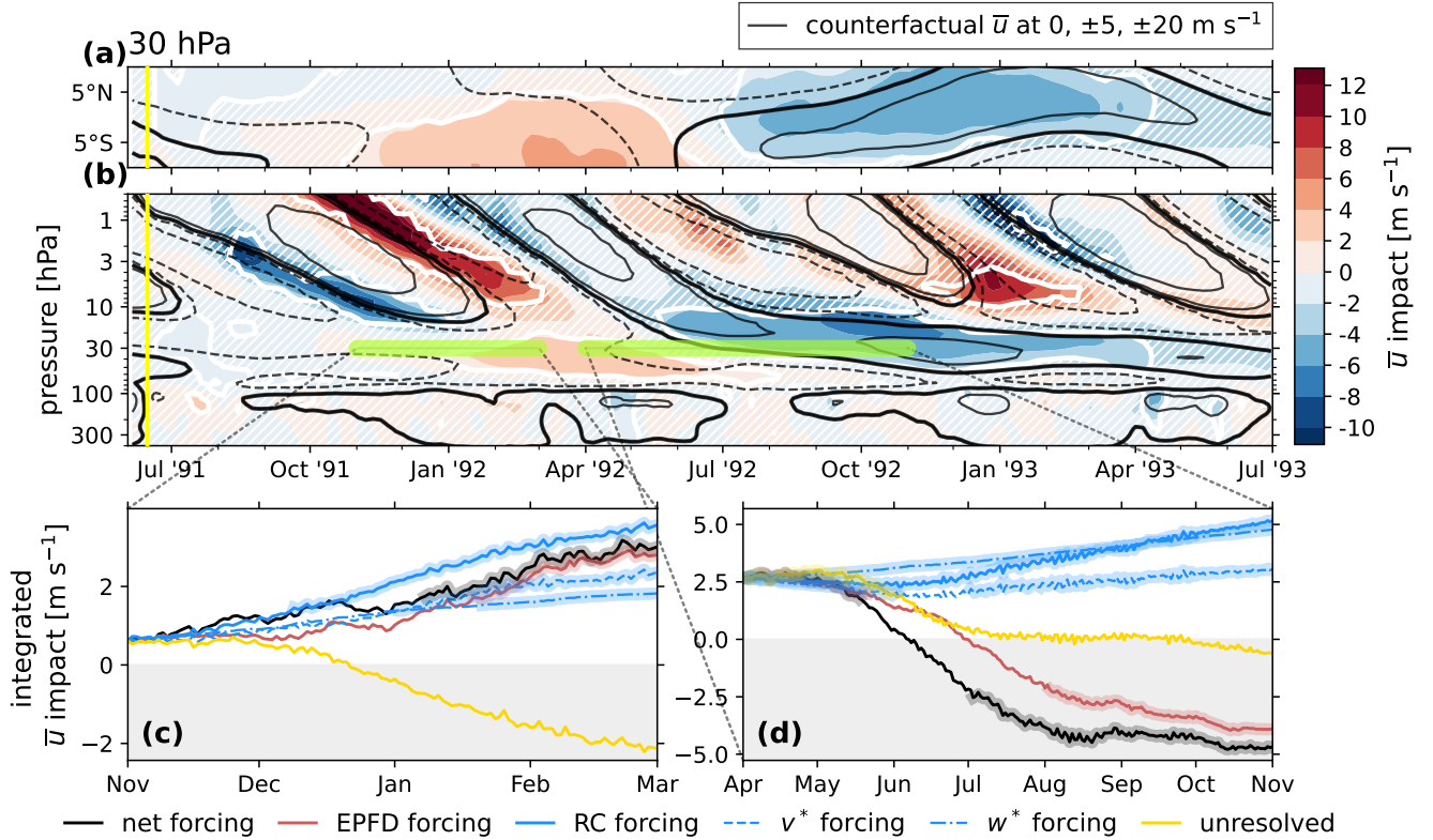
Figure 11. The same as Fig. 6, with the following modifications: panels (a), (c), and (d) are shown for the 30 hPa level. In panels (b), (c), and (d), the latitude band average is taken over 5°S–5°N. The CF \bar{u} contours in panels (a) and (b) are drawn at 0, \pm 5 , and \pm 20 \text{ m s}^{-1} .
