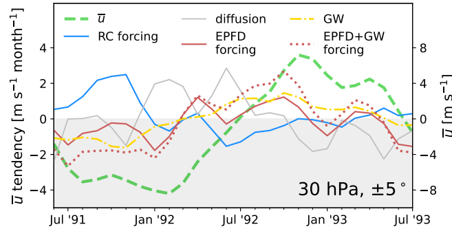
Figure 3. The TEM momentum balance of the QBO for the first two years of the CF ensemble mean, averaged over [5^\circ\text{S}, 5^\circ\text{N}] at 30 hPa. Shown are the contributions to \partial\bar{u}/\partial t in [\text{m s}^{-1} \text{ month}^{-1}] from the EPFD (red solid), gravity waves (gold dotted), the combined EPFD and gravity waves (red dotted), the residual circulation (blue solid), and diffusion (thin gray solid) as functions of latitude at 3 hPa (top panels) and 30 hPa (bottom panels). Also shown is \bar{u} itself (thick green dashed) in [\text{m s}^{-1}] , values read on the left vertical axis. The negative tendency or wind speed domain is shaded in light gray.
