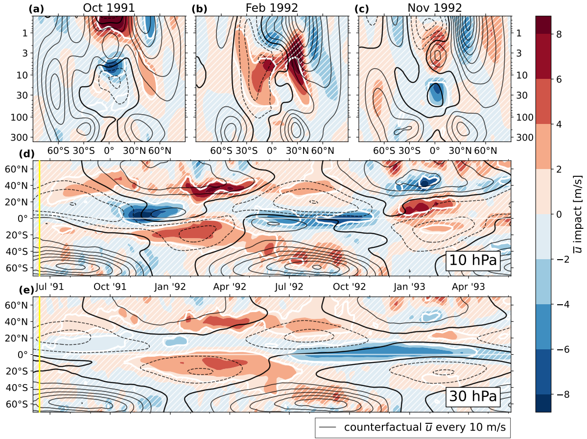
Figure 4. The ensemble-mean \Delta\bar{u} as filled contours (colorscale), with the CF ensemble-mean \bar{u} overplotted as black contours, drawn every 10 \text{ m s}^{-1} , with negative contours dashed and the zero-line in bold. A bold white contour is drawn at 95% significance, with the \Delta\bar{u} p -value computed as in Sect. 3.1. Regions of insignificance are filled with white hatching. The upper three panels show the latitude-pressure plane for time averages over (a) October 1991, (b) February 1992, and (c) November 1992. The lower two panels show the time-latitude plane for pressure levels at (d) 10 hPa, and (e) 30 hPa. In panels (d) and (e), a vertical yellow line shows the time of eruption, and a faint white line is drawn on the equator.
