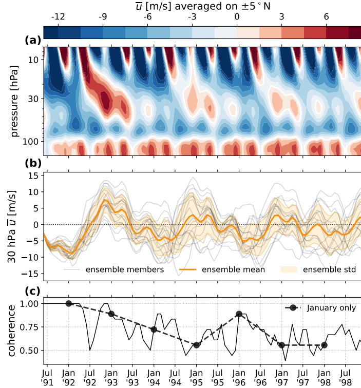
Figure 2. The QBO shown as \bar{u} averaged over [5^{\circ}\text{S}, 5^{\circ}\text{N}] for the CF ensemble mean. (a) time–pressure plane centered on the lower stratosphere. (b) zonal wind time series at 30 hPa. The ensemble mean and standard deviation in \bar{u} is shown as a bold orange line and light orange shading, respectively. Individual ensemble members are shown as faint gray lines, and the zero-line is dotted. (c) the ensemble coherence, defined as the fraction of ensemble members in agreement with the sign of the ensemble mean in panel (b). A bold dashed line with points displays the coherence evaluated only at each January.
