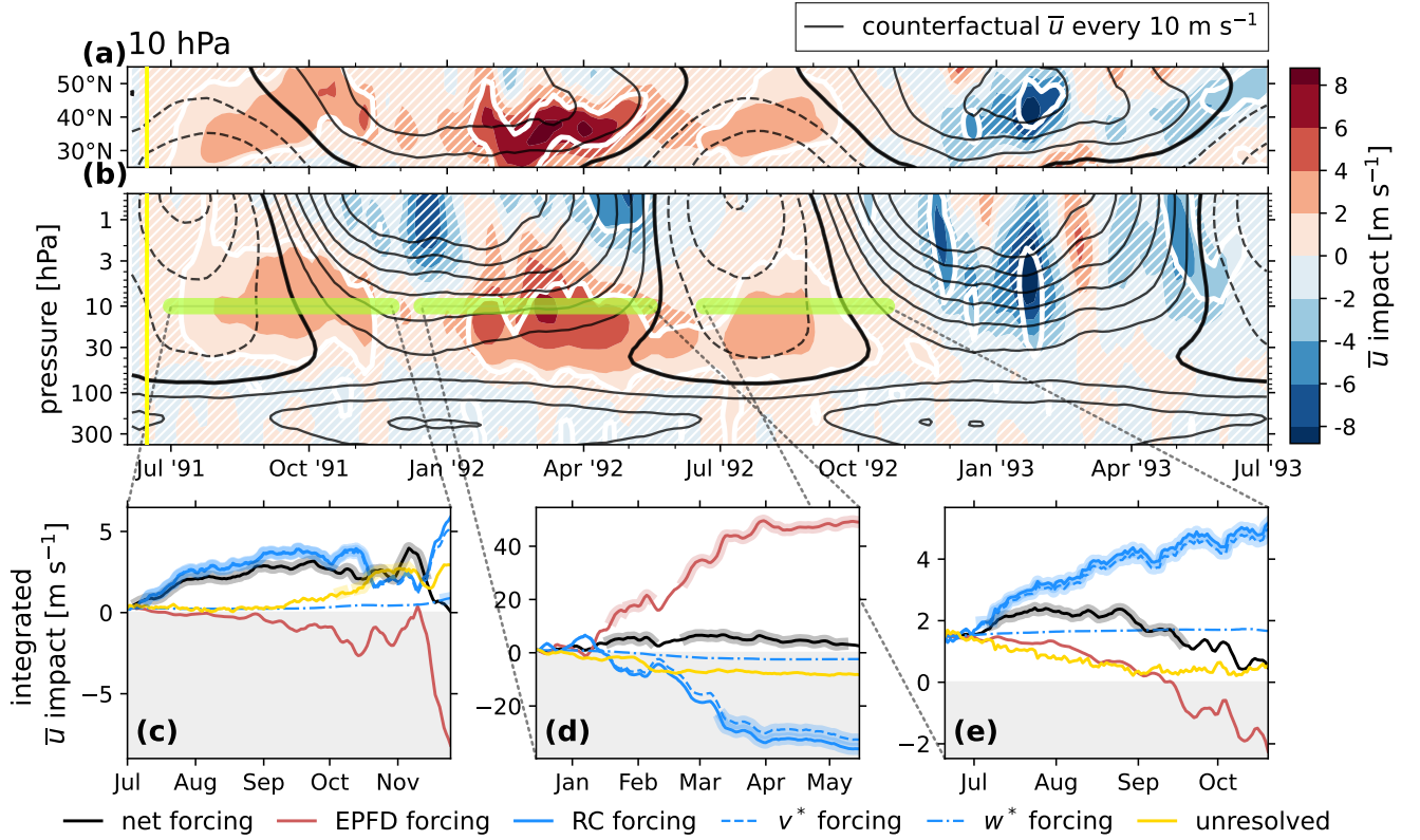
Figure 6. Vertical structure of the midlatitude zonal-wind impacts, and the TEM balance impact at 10 hPa. Panels (a) and (b) show the ensemble-mean \Delta \bar{u} as filled contours (colorscale), with the CF ensemble mean \bar{u} overplotted as black contours, drawn every 10 \text{ m s}^{-1} , with negative contours dashed and the zero-line in bold. A bold white contour is drawn at 95% significance, with the \Delta \bar{u} p -value computed as in Sect. 3.1. Regions of insignificance are filled with white hatching. (a) shows the latitude band from 25^\circ\text{N} to 55^\circ\text{N} at 10 hPa, reproduced from Fig. 4(b). (b) shows the meridional mean over 30\text{--}50^\circ\text{N} , from 400 to 0.5 hPa, for two years following the eruption (which is indicated with a vertical yellow line). In panels (c)–(e), curves show the integrated forcing impact by the EPFD (red solid), by w^* advection (dash-dotted blue), by v^* advection and the associated Coriolis force (dashed blue), and by \bar{X} = \bar{X}_{\text{GW}} + \bar{X}_d (yellow solid). Also shown is the cumulative residual velocity forcing (blue solid), and the total forcing (black solid). The curves are backed by a thick shading of a matching color where they are statistically significant. Each term has units of \text{m s}^{-1} after time integration. The total forcing curve (black solid) matches the data on the colorscale in the corresponding highlighted region of panel (b). These data are computed according to Appendix A. The negative domain is shaded.
