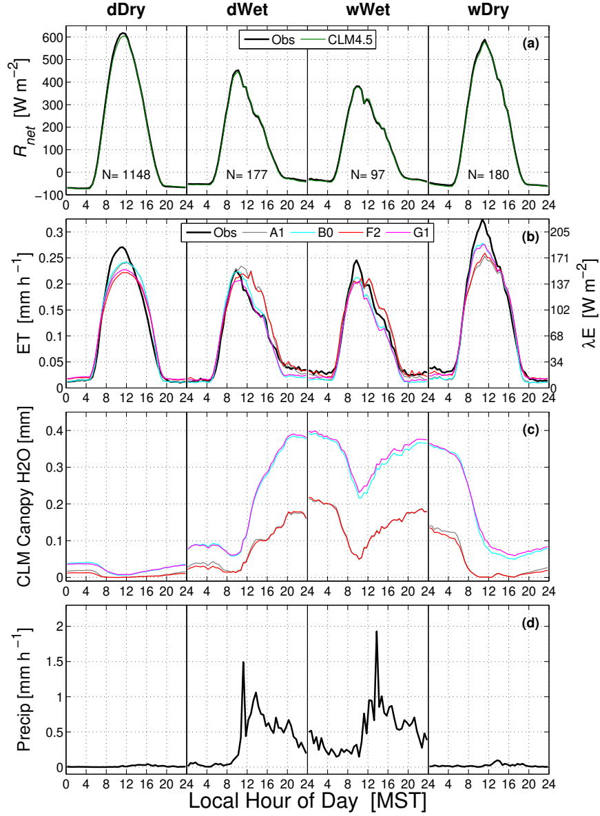
Figure 8. The warm-season mean composite diel cycle for dDry, dWet, wWet, and wDry conditions of (a) observed and CLM4.5 net radiation R_{net} , (b) observed and CLM4.5 evapotranspiration ET, (c) CLM4.5 canopy water content, and (d) precipitation. In (b) and (c) the CLM4.5 A1, B0, F2, and G1 cases are shown (see legend in panel (b) as well as Sect. 2.3 for case details). These results are from years 1999–2003 and 2006–2014 and use the same periods as Burns et al. (2018). The number of days (N) used for each diel cycle are shown in panel (a).
