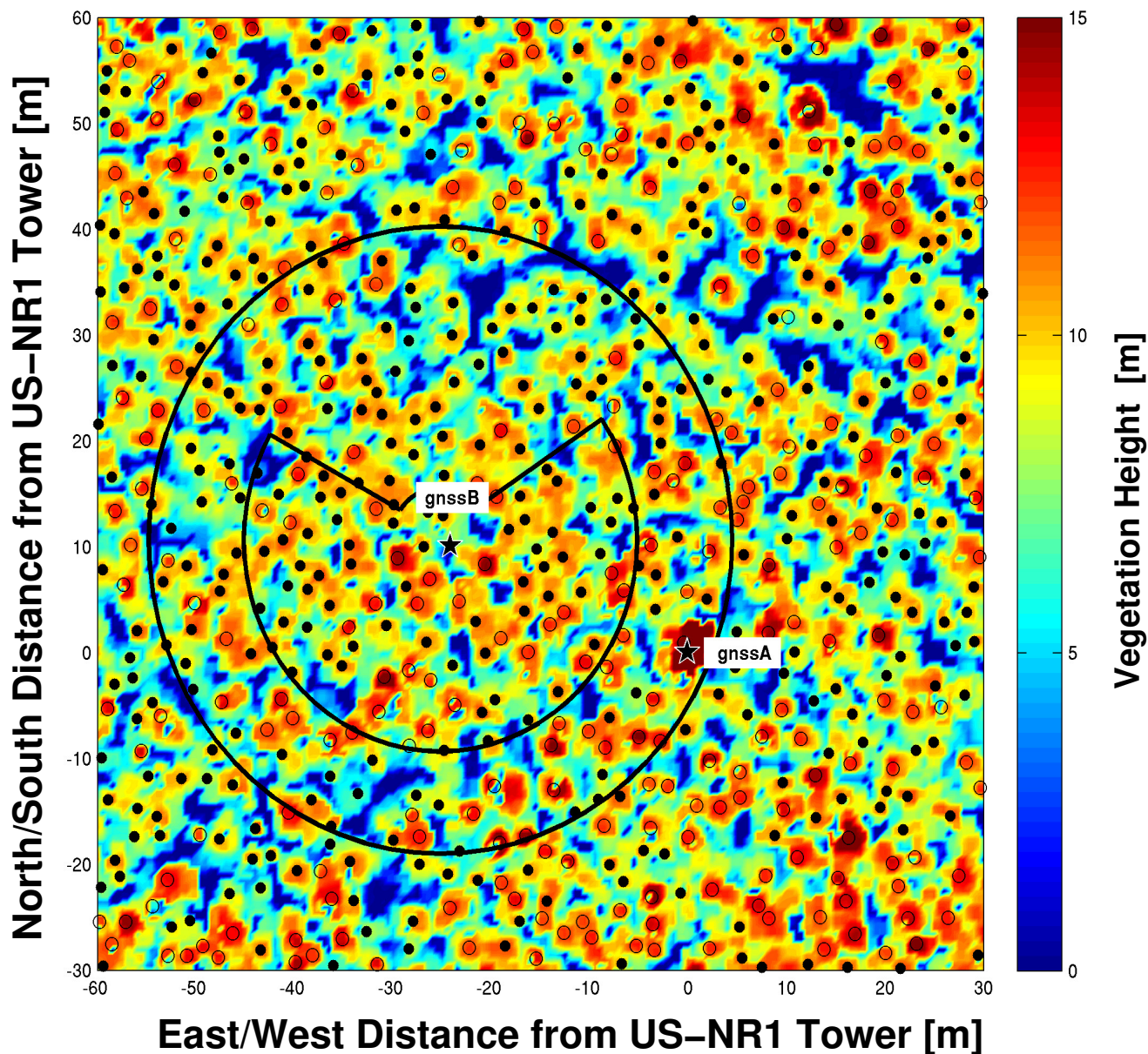
Figure 1. The location of the two GNSS antennas (gnssA and gnssB) are shown as stars on a 90 m x 90 m map relative to the location of the US-NR1 26-m tower. The gnssA antenna is at the top of the US-NR1 tower and gnssB is located in the forest 1.27 m above the ground on a tripod. The background colors show vegetation heights calculated from airborne lidar data within 0.5 m x 0.5 m regions. The filled circles indicate tree locations that are shorter than 12 m and open circles indicate trees taller than 12 m. The outer black circle around gnssB shows the VOD footprint area with a radius of \approx 30 m, while the inner black circle shows an alternate VOD footprint based on examination of the skyplot shown in Fig. S3. The VOD footprint is further discussed in Appendix B.
