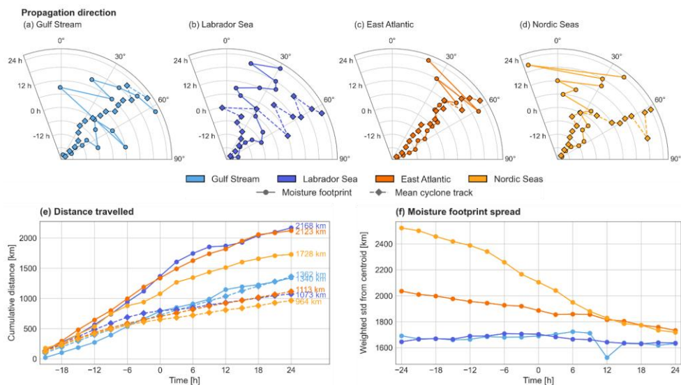
Figure A4: Movement of the moisture footprint and the mean cyclone track, characterized in terms of (a)-(d) propagation direction, (e) distance travelled, and (f) moisture footprint spread, which is defined as the weighted mean standard deviation of the source latitude and longitude positions. The coordinates of the moisture footprint are found by calculating the spherical center of mass of the mean moisture footprints. We then used the great-circle distance to track its movement and compared it with that of the mean cyclone center.
