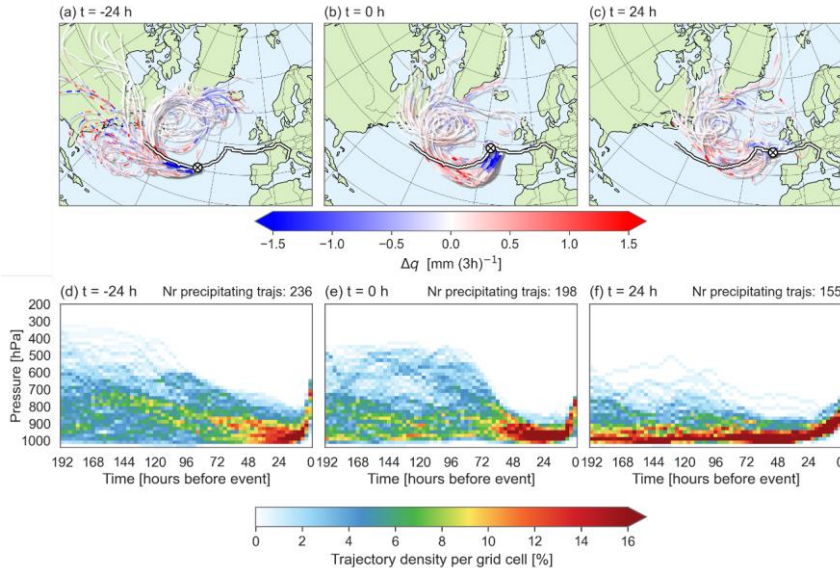
Figure 6: 8-day backward trajectories of the precipitating waters-air parcels of an East Atlantic cyclone, for (a) t = -24 h (6 May 2019, 10:00 UTC), (b) t = 0 h (7 May 2019, 10:00 UTC), and (c) t = 24 h (8 May 2019, 10:00 UTC). The trajectories are coloured by their change in specific humidity over a 3-hour period (red means moisture uptake events and blue intermittent precipitation). Additionally shown are the cyclone track (white line) and the cyclone center location (white cross). The 20% of trajectories exhibiting the most intense precipitation are mapped on the foreground for the sake of clarity. The three bottom panels show the vertical density of only the most intensely precipitating trajectories, and the number of trajectories shown here is indicated in the top right of each panel. For all panels, only the 20% of trajectories exhibiting the most intense precipitation are shown.
