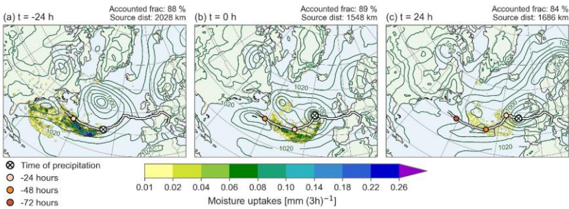
460 Figure 5: Moisture source footprint of uptakes contributing to precipitation in the cyclone center of an East Atlantic cyclone, for (a) t = -24 h (6 May 2019, 10:00 UTC), (b) t = 0 h (7 May 2019, 10:00 UTC), and (c) t = 24 h (8 May 2019, 10:00 UTC). Additionally shown are MSLP (in intervals of 5 hPa; dark green contours), the cyclone track (white line), and the cyclone center location at the time of the precipitation (white cross). Cyclone center positions at 24-hour intervals prior to the precipitation are indicated by colored dots. 465 The weighted mean accounted fraction and source distance are given in the top right of each panel.
