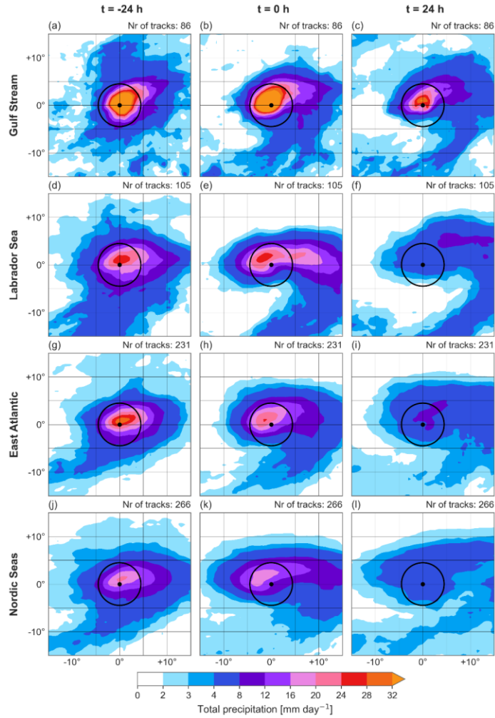
Figure 7: Cyclone-relative composites of the mean total precipitation (in \text{mm day}^{-1} ) of the cyclones in (a)-(c) the Gulf Stream, (d)-(f) the Labrador Sea, (g)-(i) the East Atlantic, and (j)-(l) in the Nordic Seas from t = -24 \text{ h} to t = 24 \text{ h} in intervals of 24 h. Precipitation is averaged over 12-hourly intervals centered on the given relative time t . Additionally shown are the cyclone center location (black dot) and surrounding circle with a radius of 500 km (black circle). The number of cyclones contributing to the composite is indicated in the top right of each panel.
