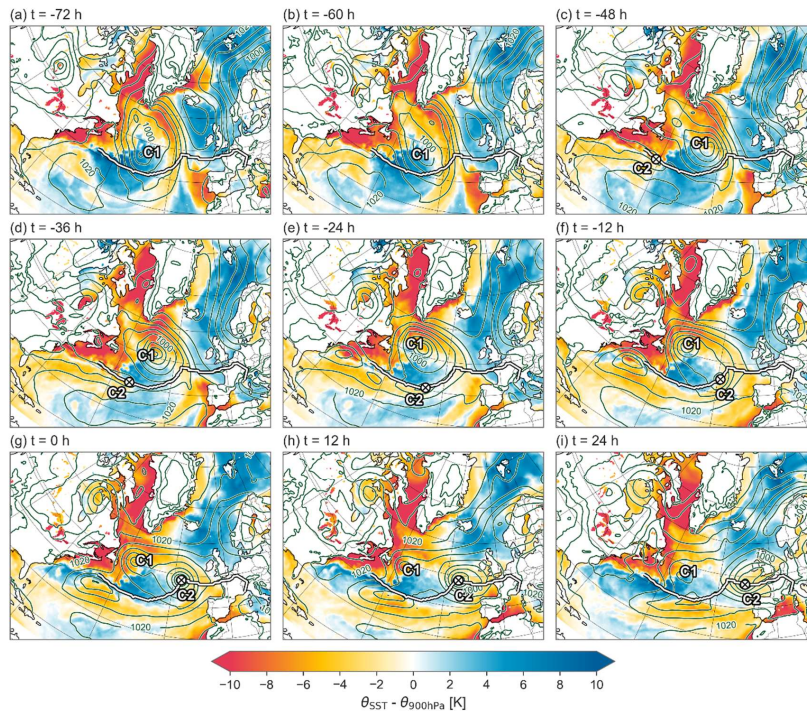
Figure 3: Sea-air potential temperature difference ( \theta_{\text{SST}} - \theta_{900\text{hPa}} , in K) associated with an East Atlantic cyclone, for t = -72 h (4 May 2019, 10:00 UTC) to t = 24 h (8 May 2019, 10:00 UTC) in 12-hourly intervals. Additionally shown are SLP contours (in intervals of 5 hPa; dark green lines), the cyclone track (white line), and the cyclone center location (white cross labelled C2; visible only from -48 hours onward, as cyclogenesis did not occur until -59 hours). Label C1 represents the location of the preceding primary cyclone.
