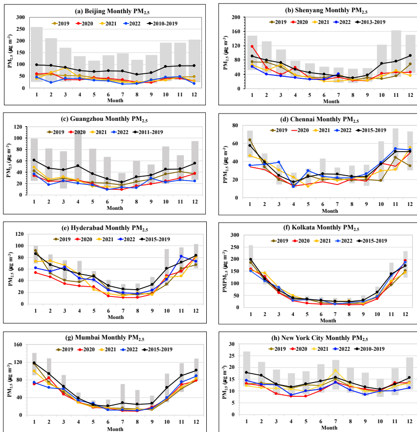
Figure 11: Monthly variations of PM_{2.5} concentration in 2019 (brown), 2020 (red), 2021 (orange), 2022 (blue), and the pre-pandemic climatology (with black line denoting the average and gray shaded areas the range of observations during the pre-pandemic period) in Beijing (a), Shenyang (b), Guangzhou (c), Chennai (d), Hyderabad (e), Kolkata (f), Mumbai (g), and New York City (h). The time series of stringency index for these cities are shown in Figure S1.
