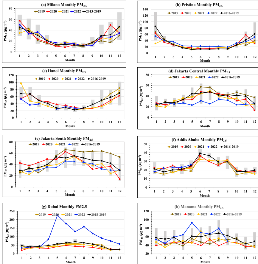
Figure 12: Monthly variations of PM_{2.5} concentration in 2019 (brown), 2020 (red), 2021 (orange), 2022 (blue), and the pre-pandemic climatology (with black line denoting the average and gray shaded areas the range of observations during the pre-pandemic period) in Milano (a), Pristina (b), Hanoi (c), Jakarta (central and south) (d and e), Addis Ababa (f), Dubai (g), and Manama (h). The time series of stringency index for these cities are shown in Figure S2.
