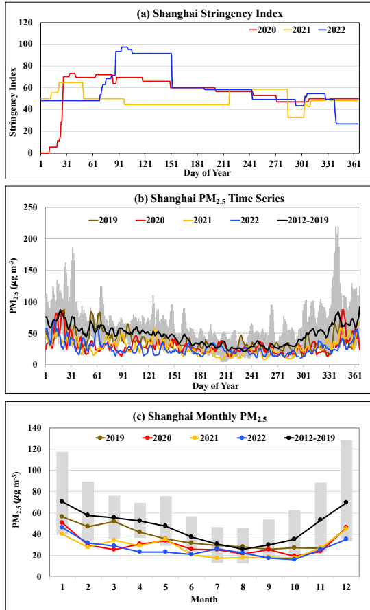
Figure 3: Time series of (a) the lockdown stringency index during the pandemic years (2020 - red, 2021 - orange, and 2022 - blue) and (b) the 5-day running mean PM 2.5 concentration over years for four individual years of 2019-2022 (with brown, red, orange, and blue line denotes 2019, 2020, 2021, and 2022, respectively) in Shanghai, China. The monthly average PM 2.5 concentrations (µg m -3 ) are shown in (c). Also shown in (b) and (c) is the pre-pandemic climatology with black line denoting the average and gray shaded areas the range of observations during the pre-pandemic period.
