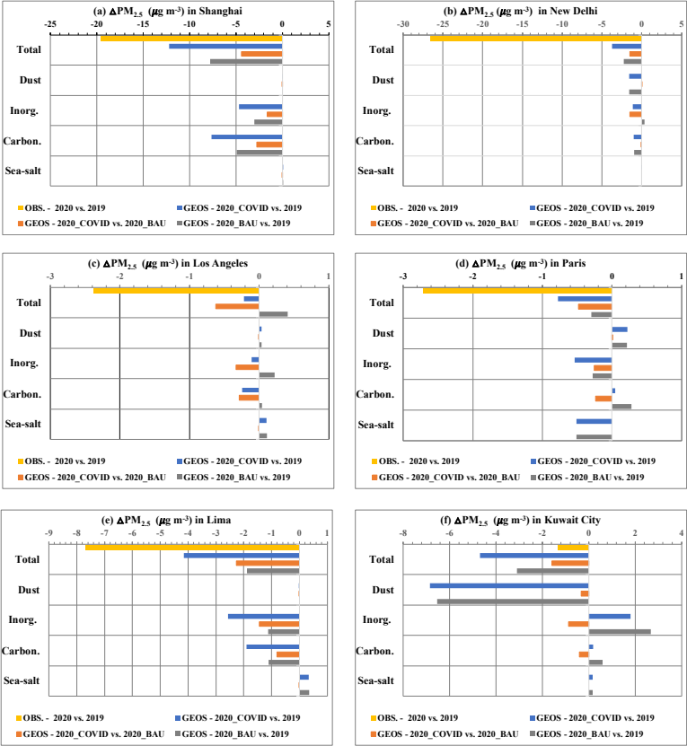
Figure 10: Absolute differences ( \mu g m^{-3} ) in March-April average PM_{2.5} between 2020 and 2019 (a negative value indicating that PM_{2.5} was smaller in 2020 than 2019) in Shanghai, China (a), New Delhi, India (b), Los Angeles, USA (c), Paris, France (d), Lima, Peru (e), and Kuwait City, Kuwait (f). Shown here include observed (yellow bars) and GEOS simulated (blue bars) changes in total PM_{2.5} . The GEOS simulations are further classified into dust, inorganic aerosol, carbonaceous aerosol, and sea salt, shown below the total PM_{2.5} change. For both total and component PM_{2.5} , GEOS simulation is partitioned into GEOS PM_{2.5} change due to anthropogenic emission change (orange) and GEOS PM_{2.5} change due to differing meteorology (gray). Relative changes in PM_{2.5} are listed in Table 2.
