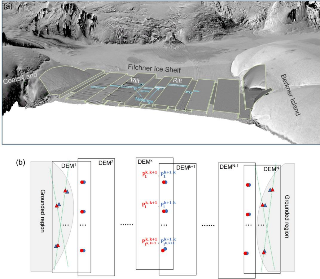
Figure 1. (a) High-resolution small-coverage DEMs (e.g., REMA strips of \sim 16\sim 18 km \times \sim 110\sim 120 km) are unified and integrated for accurate 3D rift structural and mélange dynamic monitoring in a large Antarctic ice shelf environment (e.g., \sim 165 km wide Filchner Ice Shelf). The LIMA mosaic (Bindschadler et al., 2008) is draped on the RAMP DEM (Liu et al., 2001) with a vertical exaggeration factor of 40 times. (b) Concept of the MDAM system to connect sub-DEMs across the ice shelf through “tie points” (TP, represented by circles) to create a DEM time series. The “ground control points” (GCP, represented by triangles) are used to fix the combined DEM model to grounded regions at ice shelf margins. The closely located red and blue circles (triangles) are from adjacent sub-DEMs and form corresponding TP (GCP) pairs.
