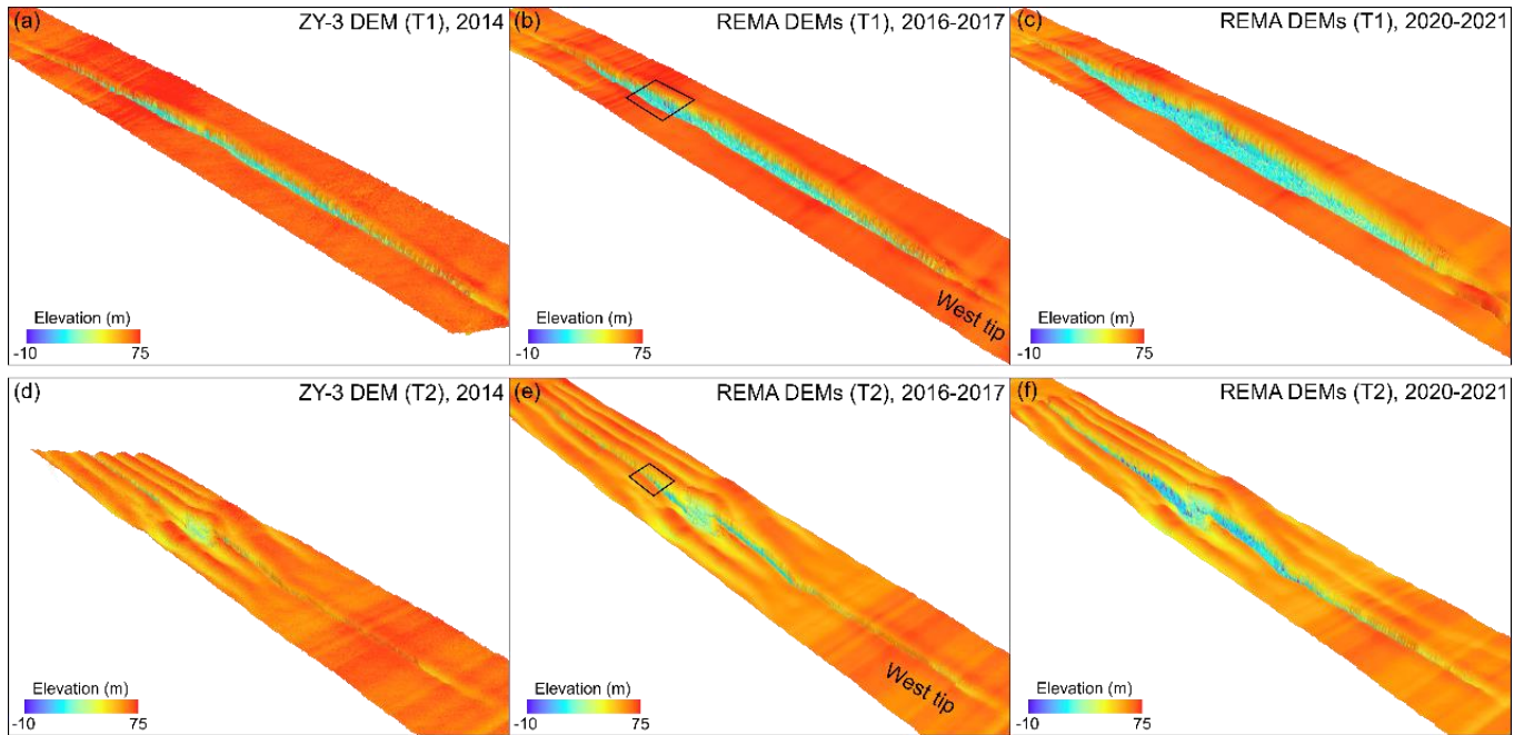
285 Figure 9. Multi-satellite DEM time series of two large rifts (T1 and T2) on Filchner Ice Shelf from 2014 to 2021 in 3D: (a) and (d) are reconstructed ZY-3 DEM of 2014, (b) and (e) are bias-corrected REMA DEMs of 2016-2017, and (c) and (f) are bias-corrected REMA DEMs of 2020-2021. The boxes in (b) and (e) indicate two rift sections where details of 3D structure and mélange are presented in Fig. 10.
