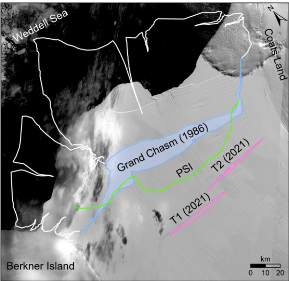
395 Figure A1. Rifts of T1 and T2 (pink) in 2021, Grand Chasm (blue) in 1986; passive shelf ice (PSI) boundary (green) (Fürst et al., 2016); ice bergs calved in 1986; background is Landsat image of February 11, 2021.
