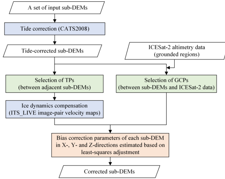
140 Figure 2. Data processing principle of the multi-temporal DEM adjustment model (MDAM).
