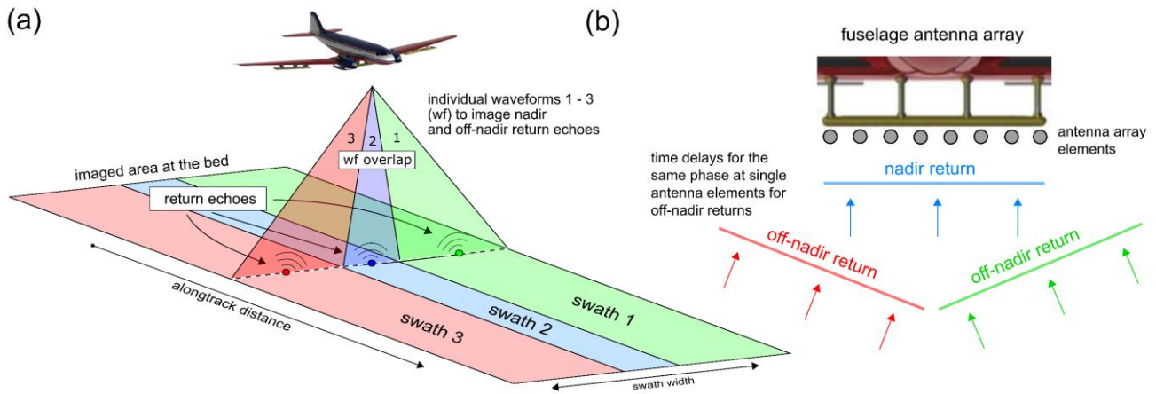
Figure 2: (a) Individual waveforms from a multi-antenna radar array used to image both nadir and off-nadir return echoes from the ice-bed interface. (b) Time delays for the same phase at single antenna elements are used to geolocate the off-nadir return echoes.
