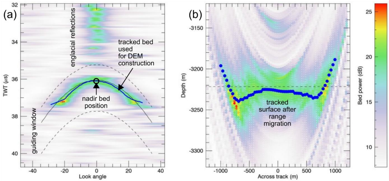
145 Figure 3: (a) Cross-track surface tracking at each nadir bed position produced from the MUSIC algorithm (Paden et al., 2010). (b) The tracked surface is range migrated to convert the two-way travel time values to depth.
