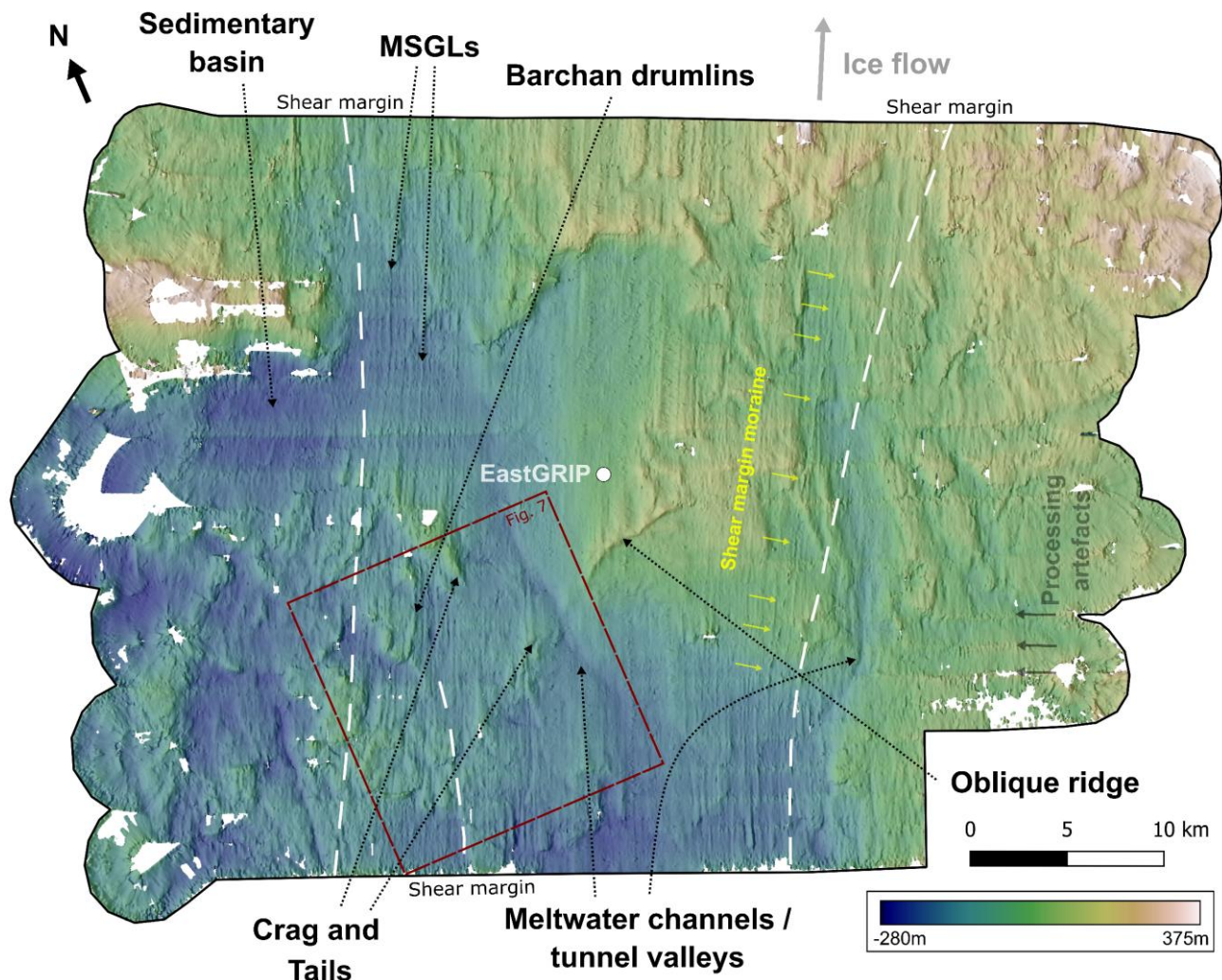
200 Figure 5: Subglacial topography produced from swath radar measurements at the onset of NEGIS (Carter et al., 2025). The hill-shaded DEM (referenced to WGS84) allows interpretation of an assemblage of subglacial landforms, characteristic of ice streaming, such as mega-scale glacial lineations, crag and tails, and barchan drumlins. Location of the survey shown in Fig. 1 and the red box shows the location of Fig. 7. Arrows on top indicate True North and direction of ice flow. The line delineating the location of the shear margin (maximum shear strain rate) is dashed, as this 205 represents the central point of the broader transition between slow and fast flow (the shear zone).
