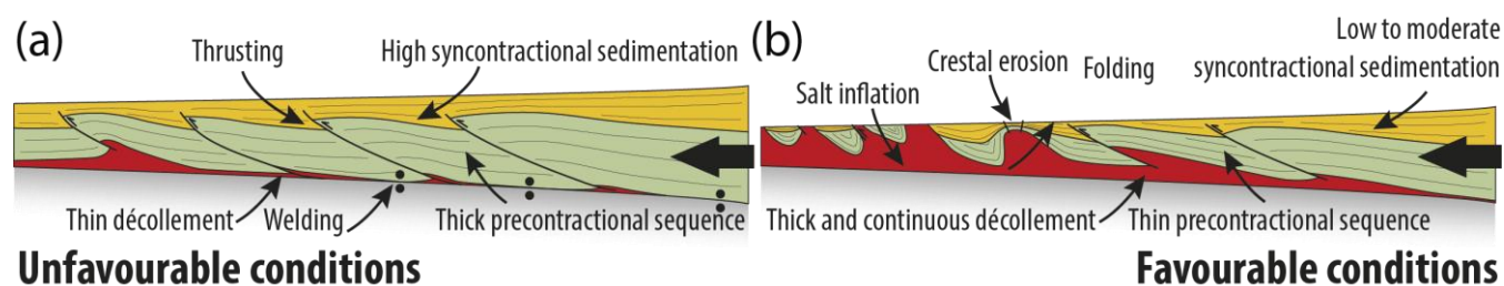
Figure 1: Summary sketches that illustrate unfavorable (A) and favorable (B) conditions for the development of purely contractional diapirs in fold-and-thrust belts.
