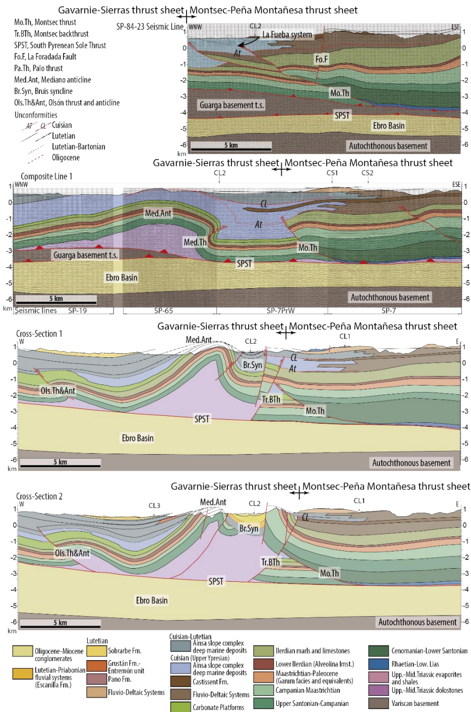
Figure 7. Cross sections and interpreted seismic lines illustrating the subsurface structure of the Montsec-La Fueba system (SP-84-23 seismic line), and the north to south along strike variability of the Montsec-Mediano anticline structures (Composite line 1, Cross-section 1 and Cross section 2). See fig. 4 for location.
