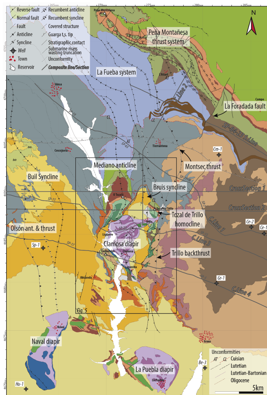
245 Figure 4. Geological map of the area studied. See figure 3 for the colour legend of stratigraphic units. Main structural features described in the text are labelled. Dark grey lines represent seismic sections, composite lines and cross-sections traces. Note that black-white dashed lines denote buried structural features. The tip line of the Guarga basement thrust sheet is represented as a dashed black and white line with open black arrows. Southern and northern areas are adapted from Barnolas et al. (1994a,b; 1999) and Santolaria et al. (2014).
