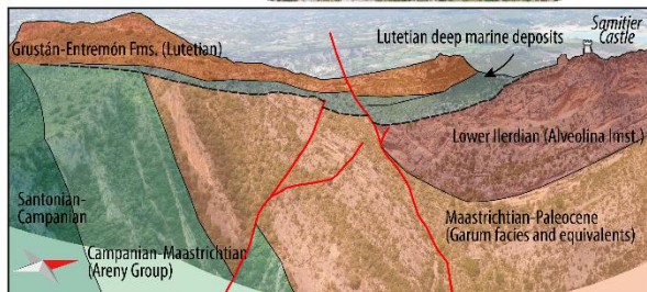
Figure 6. (a), Drone image of the northern boundary of the Clamosa diapir and the Mediano anticline and its interpretation. (b), Close up view of northwestern flank of the Clamosa diapir and Mediano anticline. (c), Interpreted picture of the NNE-SSW trending, west-dipping extensional faults related to the collapse of the diapir during Oligocene. See their location in Fig. 5.
