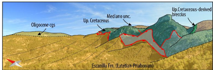
Figure 6. (a), Drone image of the northern boundary of the Clamosa diapir and the Mediano anticline and its interpretation. (b), Close up view of northwestern flank of the Clamosa diapir and Mediano anticline. (c), Interpreted picture of the NNE-SSW trending, west-dipping extensional faults related to the collapse of the diapir during Oligocene. See their location in Fig. 5.
