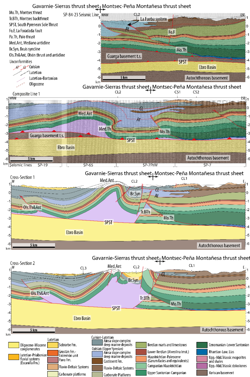
360 Figure 7. Cross sections and interpreted seismic lines illustrating the subsurface structure of the Montsec-La Fueba system (SP-84-23 seismic line), and the north to south along strike variability of the Montsec-Mediano anticline structures (Composite line 1, Cross-section 1 and Cross section 2). See fig. 4 for location and appendix B for the uninterpreted version of the seismic lines. Note that the thickness of the Upper Cretaceous to Ilerdian sequence in the Tozal de Trillo Homocline (Cross-sections 1 and 2) and the growth of the same sequence in cross-section 2 are apparent due to the low angle between the section traces and the strike of these tilted sequences there. 365
