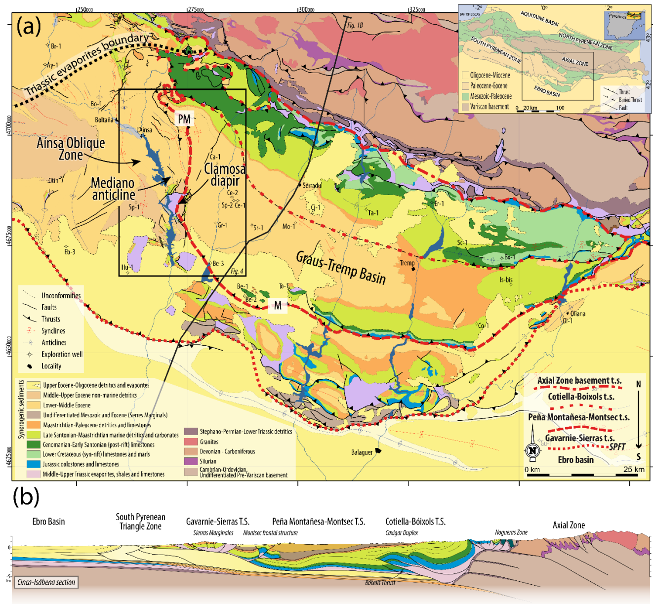
95 Figure 2. (a), Geological map of the South Pyrenean Central Salient. Dashed and dotted red lines represent the contact between the Axial Zone and the Southern Pyrenean fold and thrust belts and the Bóixols-Cotiella, Montsec-Peña Montañesa and Gavarnie-Sierras thrust sheets (modified from Muñoz et al., 2018 and Santolaria et al., 2024; inset map after Beamud, 2013). A black rectangle frames the studied area shown in Fig. 4. (b), Cross-section illustrates the western half of this Pyrenean Salient (from Santolaria et al., 2024). PM, Peña Montañesa thrust; M, Montsec thrust.
