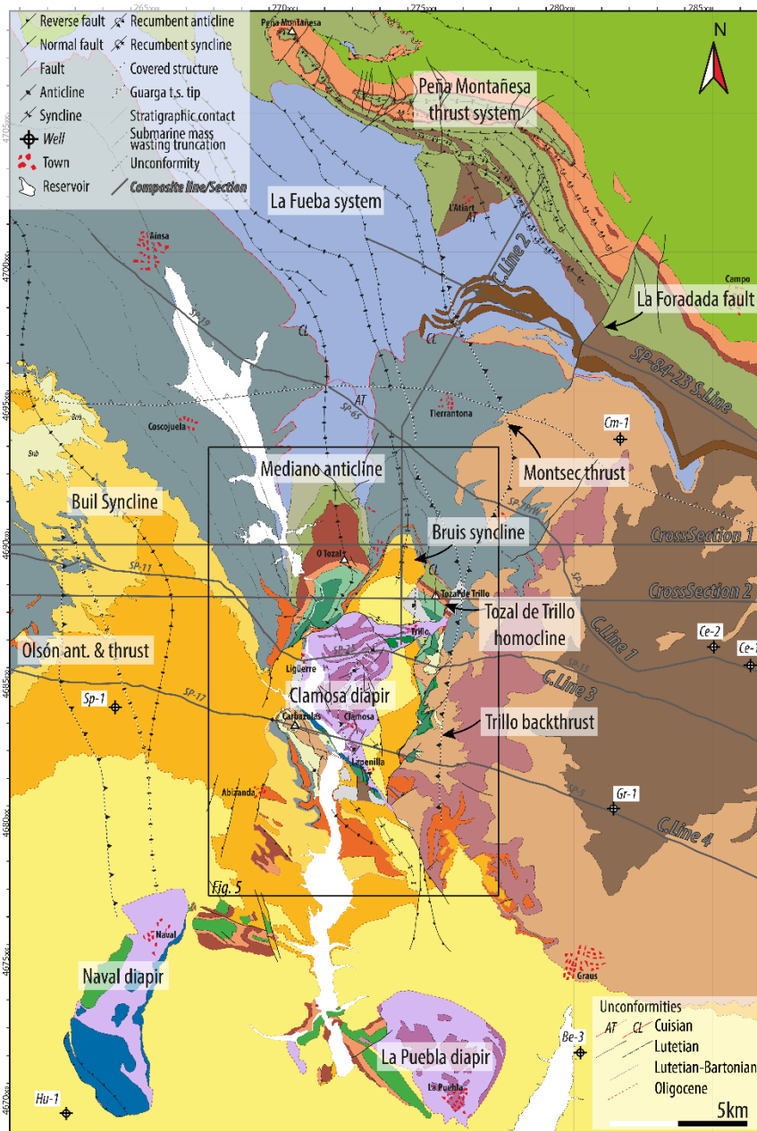
Figure 4. Geological map of the area studied. See figure 3 for the colour legend of stratigraphic units. Main structural features described in the text are labelled. Dark grey lines represent seismic sections, composite lines and cross-sections traces. Note that black-white dashed lines denote buried structural features. The tip line of the Guarga basement thrust sheet is represented as a dashed black and white line with open black arrows. Southern and northern areas are adapted from Teixell et al. (1994a, b) Robador-Moreno and Zamorano-Cáceres (1999) and Santolaria et al. (2014).
