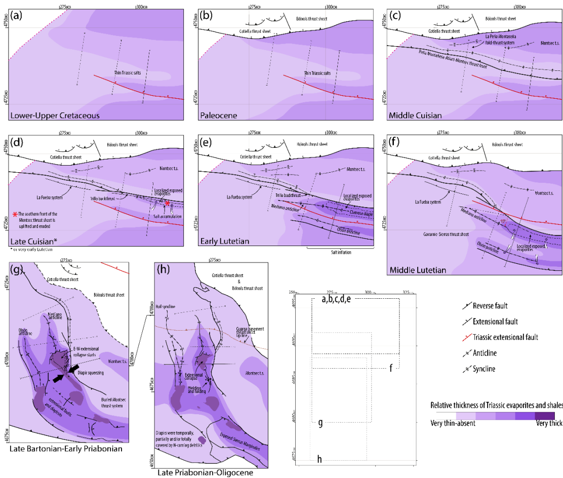
Figure 10. Plan view reconstruction of the studied area (partly modified from Muñoz et al., 2013 and Santolaria et al., 2014). Weak to strong purple denote thin to thick Triassic salt accumulations. Red line represents the basement normal fault bounding the southern salt basin as seen in Fig. 9.
