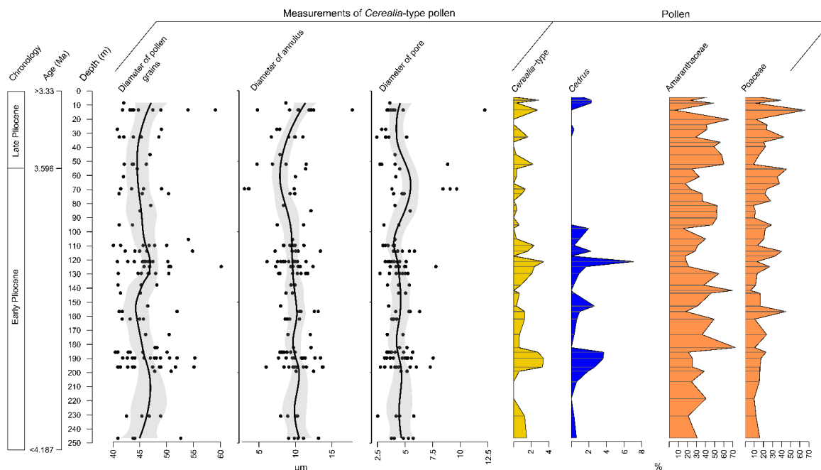
480 Figure 5: Measurements of diameter of pollen grains, annulus and pores of large pollen grains of Poaceae from the core BS-87 Burdur against core depth. The measurements are compared with the variation in the percentages of some of the more characteristic pollen taxa, i.e. Cerealia -type, Cedrus , Amaranthaceae and Poaceae .
