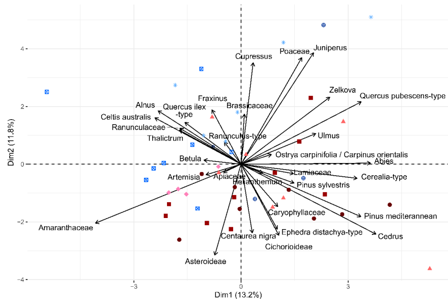
Figure 4: Principal component analysis (PCA) on selected terrestrial pollen taxa from the lacustrine succession of the Burdur Basin-fill (Türkiye). Sample map was coloured according to the PAZ (presented in Fig. 3).
