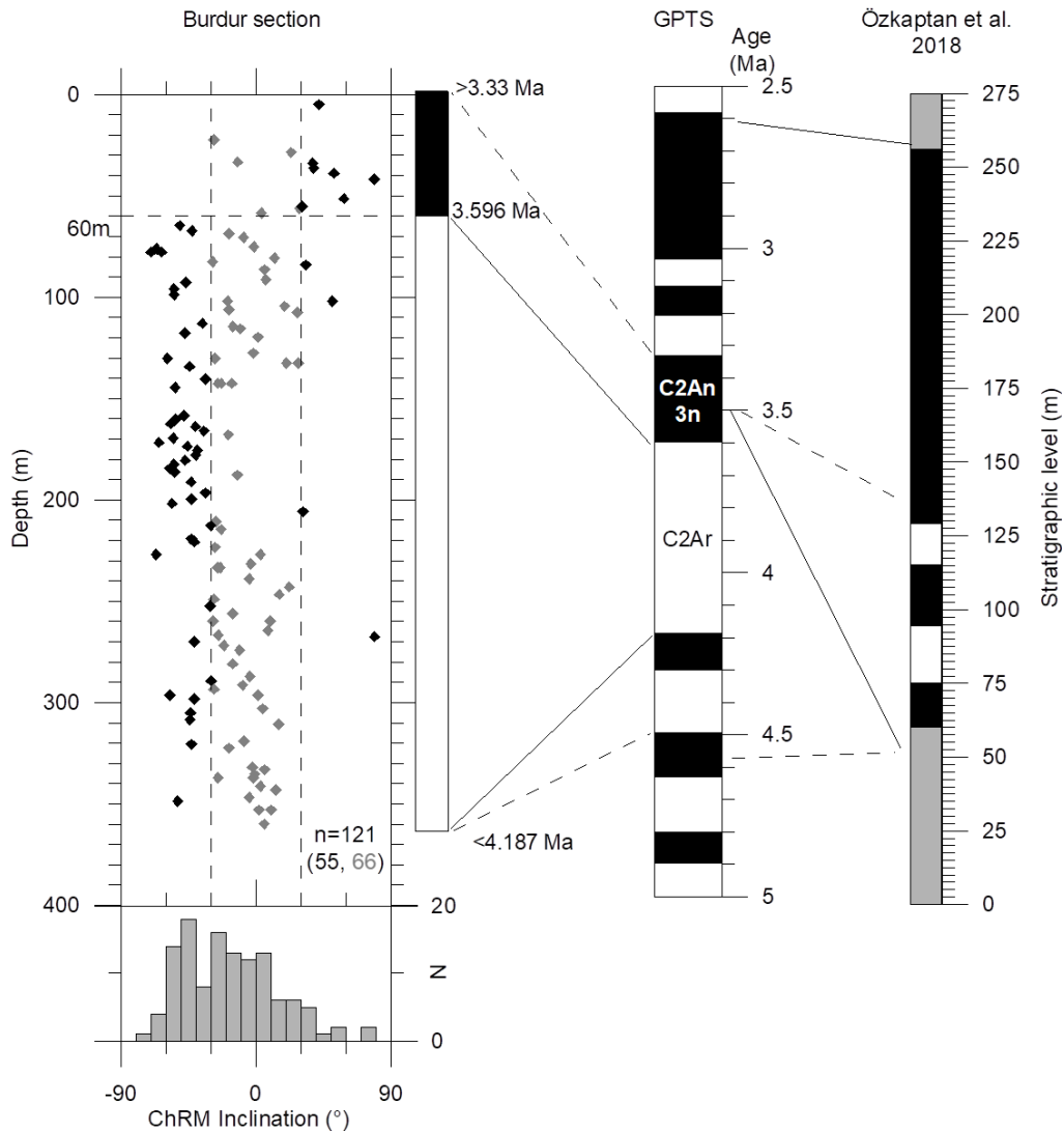
320 Figure 3: Magnetostratigraphic correlations of the Lake Burdur Pliocene lacustrine sediment in BS-87 core (this study; left) compared to the previously published surface section of Burdur (Özkaptan et al. 2018) with the GPTS (Hilgen et al., 2012). ChRM: Characteristic Remanent Magnetizations.
