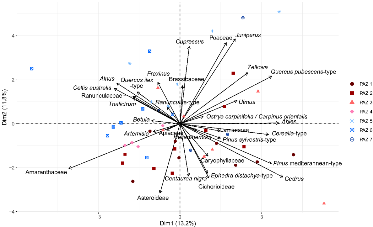
Figure 5: Principal Component Analysis (PCA) on selected terrestrial pollen taxa from the core BS-87 Burdur. The sample map was color-coded according to the PAZ (presented in Fig. 4).
