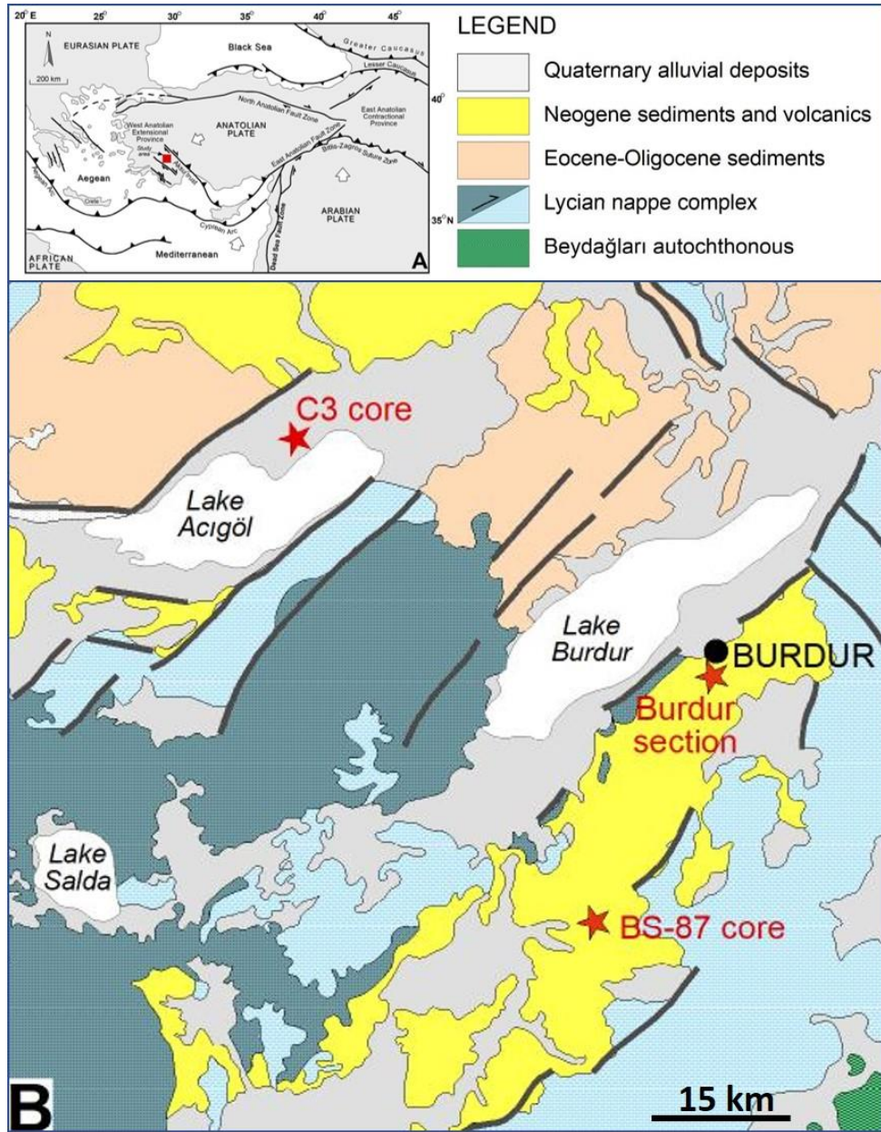
Figure 1: (A) Tectonic map of the Eastern Mediterranean showing major tectonic structures (after Bozkurt, 2003), (B) Geological maps of Acıgöl and Burdur Province and locations of selected cores and sections: Acıgöl C3 core (Andrieu-Ponel et al., 2021), Burdur Pmag section (Özkaptan et al., 2018) and Burdur BS-87 core (this study).
