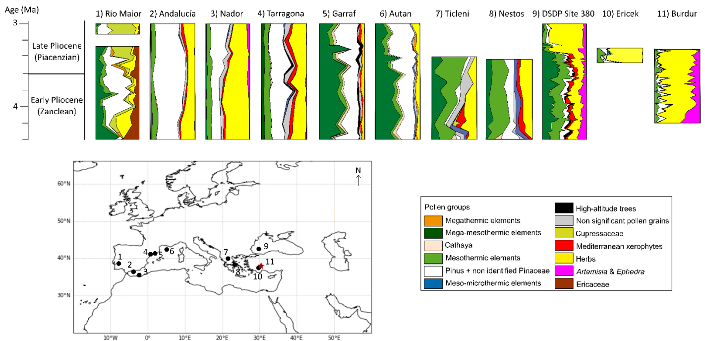
Figure 8: Vegetation changes around the Mediterranean Basin for the Early-Late Pliocene transition for selected palynological studies: 1) Rio Maior F16 (Diniz, 1984), 2) Andalucía G1 (Suc et al., 1995), 3) Nador (Feddi et al., 2011), 4) Tarragona E2 (Bessais and Cravatte, 1988), 5) Garraf 1 (Suc and Cravatte, 1982), 6) Autan 1 (Cravatte and Suc, 1981), 7) Ticleni 1 (Jiménez-Moreno et al., 2007), 8) Nestos 2 (Jiménez-Moreno et al., 2007), 9) DSDP site 380 (Popescu, 2006), 10) Ericek (Jiménez-Moreno et al., 2015) and 11) Burdur (this study) presented in percentages. The description of ecological classification of pollen taxa is presented in Supplementary Table S4.
