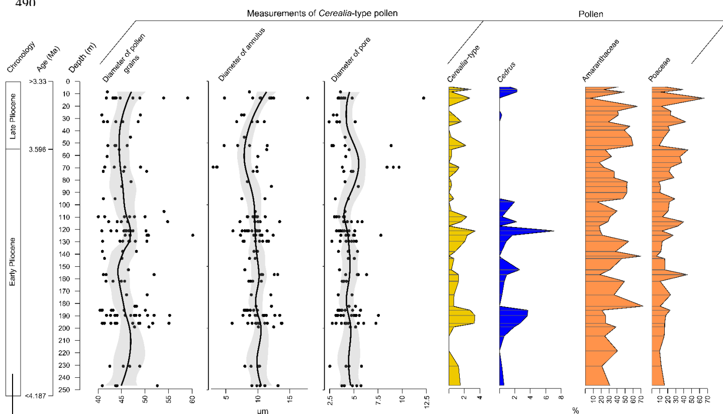
Figure 6: Measurements of diameter of pollen grains, annulus and pores of large pollen grains of Poaceae from the core BS-87 Burdur against core depth. The measurements are compared with the variation in the percentages of some of the more characteristic pollen taxa, i.e. Cerealia -type, Cedrus , Amaranthaceae and Poaceae.
