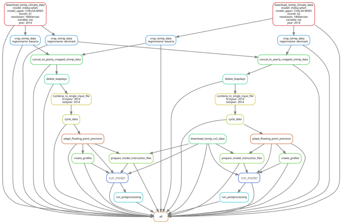
Figure 6. Illustration of the Snakemake workflow from our pipeline example. The pipeline consists of downloading, cropping, and mapping data to enable a model run. Different regions can easily be defined, resulting in one model run per region, in this case for two regions. Snakemake takes care that when an intermediate result changes, all steps depending on this intermediate result will be re-executed.
