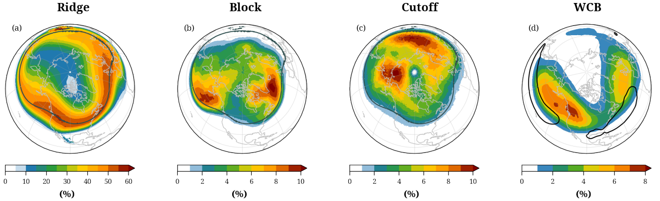
Figure 1. The climatological frequency of occurrence of weather features in DJF: (a) ridges, (b) blocks, (c) tropospheric cutoffs, and (d) WCBs at end-of-ascent. The black contours illustrate in (a-c) the climatological mean waveguide (i.e. the 2 PVU contour averaged for the four isentropes selected for DJF) and in (d) the 95th percentile of the WCB start-of-ascent frequency. Note the different contour intervals.
