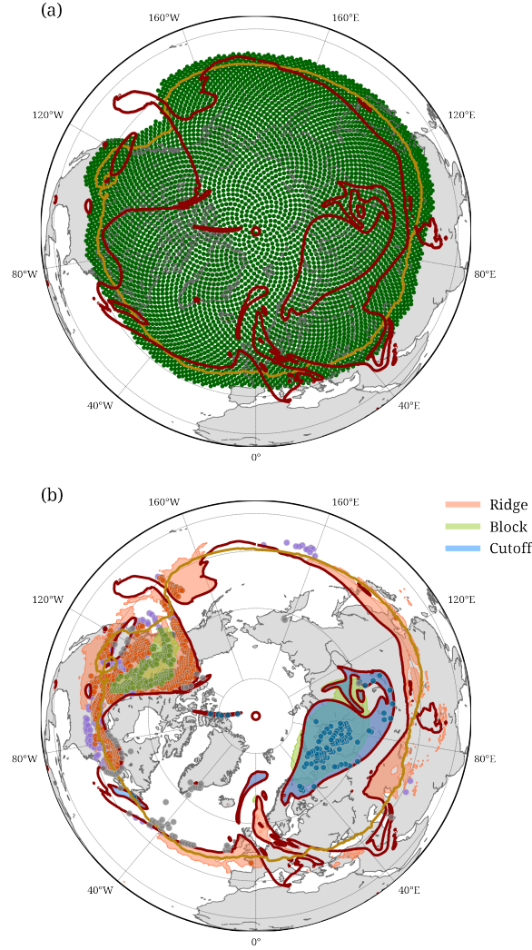
Figure 2. Example illustrating the Lagrangian analysis method to identify the four types of WCB-waveguide interactions at 00 UTC on 03 January 2016. The red and yellow contours represent the instantaneous and 30-day running mean waveguides (2 PVU isolines on 315 K), respectively. Green dots in (a) show the selected starting points on this isentrope for the five-day backward trajectory calculation. In (b) , regions identified as ridges, blocks, and tropospheric cutoffs are indicated with orange, light green, and blue shading, respectively. Dots in (b) show starting points of backward trajectories that satisfy the WCB ascent criterion, with the color indicating the interaction type: no-interaction (purple), ridge (orange), block (green), and cutoff (blue). Grey dots indicate stratospheric WCB air parcels, which are not included in the analysis.
