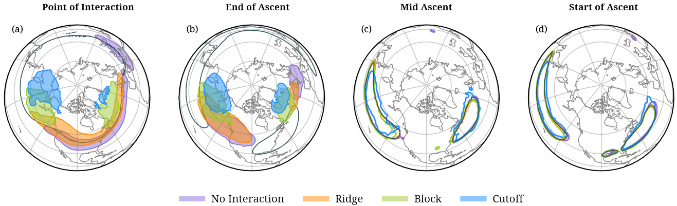
Figure 6. The main climatological frequency maxima (95th percentile regions) of WCB trajectories for: no-interaction (purple shading and contours denoting the regions where the interaction type frequency exceeds the 95th percentile), ridge interaction (orange), block interaction (green), and cutoff interaction (blue). The maxima are shown at the four trajectory phases (a) point-of-interaction, (b) end-of-ascent, (c) mid-ascent, and (d) start-of-ascent. In (c,d) shading is omitted to enhance readability. The black contours illustrate in (a) the climatological mean waveguide, in (b) the climatological jet stream identified by a wind speed of 30 \text{ m s}^{-1} , where both are averaged over the four isentropic levels considered, and in (c) and (d) the 95th percentile regions of total WCB mid-ascent and start-of-ascent, respectively.
