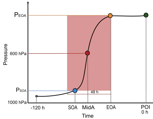
Figure 3. Schematic to introduce distinct WCB trajectory phases for a single five-day backward trajectory that fulfills the WCB criterion during the 48-hour time window indicated by the red box. The green dot denotes the starting point of the backward trajectory, which is also referred to as the ‘point-of-interaction’ (POI) of the WCB with the waveguide. The other dots denote the end-of-ascent (EOA, orange), the mid-ascent (MidA, red), which is when the trajectory crosses the 600-hPa level, and the start-of-ascent (SOA, blue).
