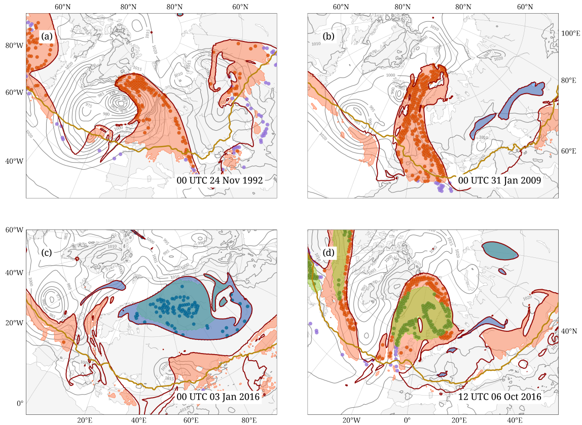
Figure 4. Four case studies illustrating WCB-waveguide interaction events previously discussed in the literature, at (a) 00 UTC on 24 November 1992, (b) 00 UTC on 31 January 2009, (c) 00 UTC on 03 January 2016, and (d) 12 UTC on 06 October 2016. The elements shown are the same as in Fig. 2b, except that here, stratospheric WCB air parcels are not shown.
