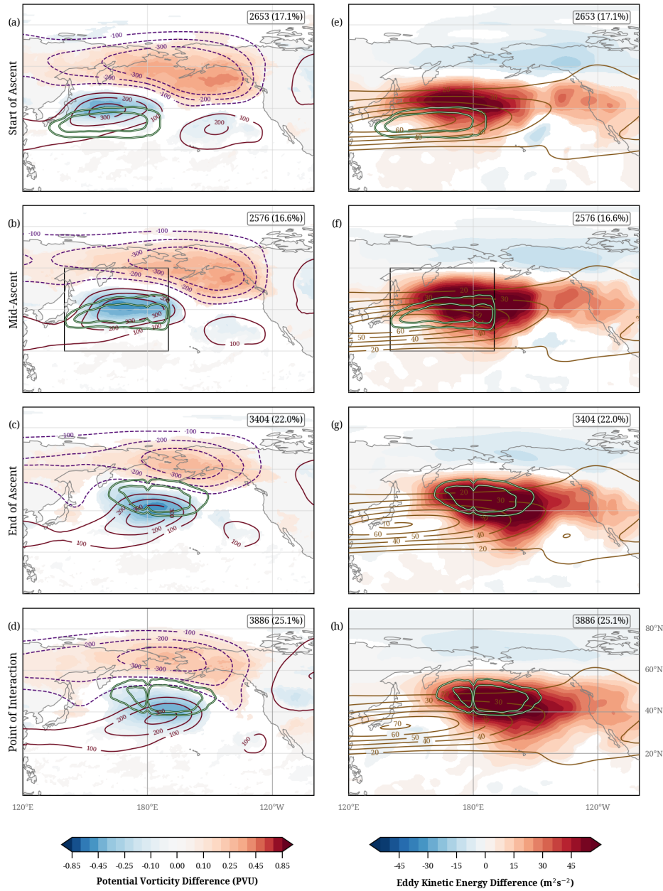
Figure 9. Composites of ridge-interaction time steps for the four trajectory phases: start-of-ascent ( a,e ), mid-ascent ( b,f ), end-of-ascent ( c,g ), and point-of-interaction ( d,h ). (a-d) show PV at 320 K and geopotential height anomalies at 250 hPa (solid and dashed lines for positive and negative values, respectively). (e-h) show 500 hPa EKE anomalies and low-pass filtered zonal wind at 250 hPa (brown lines). Grid points where PV and EKE anomalies fall within the 1st–99th percentile confidence interval (see text) are shown in white. The highlighted white-green contours in (a-h) show the 98th and 99th percentile of occurrence frequency of the ridge-interaction WCB air parcels in the corresponding phases. Only the WCB air parcels that ascend within the rectangle shown in (b,f) are selected for the analysis. The number of time steps included in each composite and the corresponding percentage w.r.t. all DJF time steps in the considered 43-y period are given in each panel.
