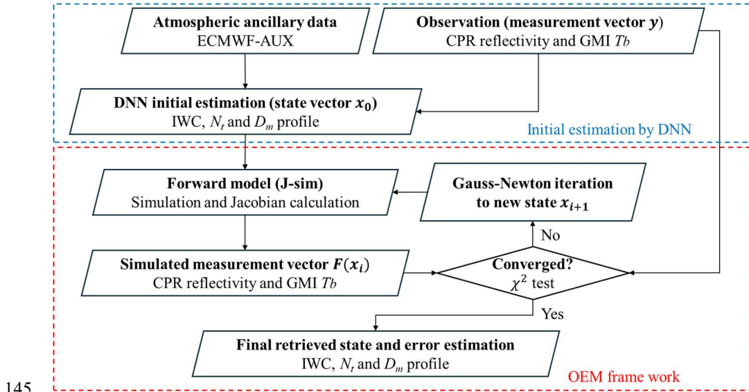
Figure 2:1: Flow of the retrieval algorithm.
