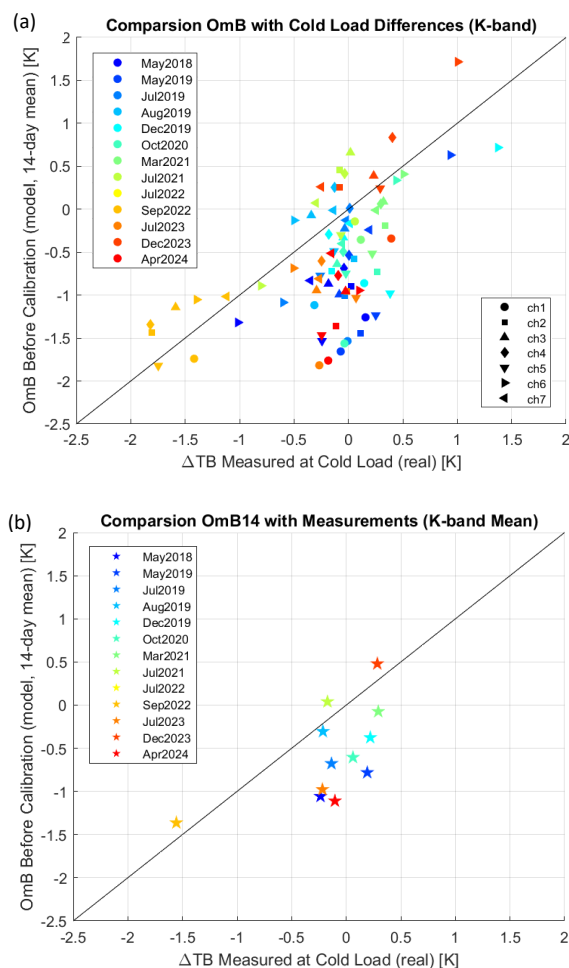
485 Figure 6: Comparison of observation minus background (OmB) T_B s as a 14-day mean (clear-sky only) before an absolute calibration with the observed T_B differences at the cold load during absolute calibrations for TOPHAT, (a) for channels 1–7 from the K-band separately, and (b) the mean over all channels. Data from 13 absolute calibrations which took place between May 2018 and Apr. 2024 are used.
