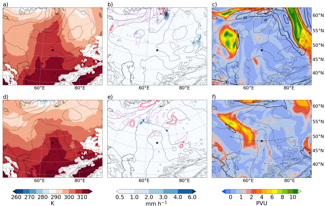
Figure 4. Synoptic situation before and at the time of cyclogenesis, i.e., at (a-c) 08 UTC on 1 July, and (d-f) 08 UTC on 3 July 2021. The cyclone center is always in the center of the panels, denoted by a black star. All panels show SLP (black lines, every 4 hPa). In addition, left panels show \theta at 850 hPa (colors, in K), middle panels show hourly precipitation (color, in \text{mm h}^{-1} ) and PV at 850 hPa (pink, red, and orange contours for 1, 2, and 4 PVU, respectively), and right panels show PV at 330 K (colors, in PVU) and wind speed at 250 hPa (bold black contours, every 10 \text{ m s}^{-1} starting at 30 \text{ m s}^{-1} ). The gray dashed line in (f) indicates the location of the vertical cross section in Fig. 5a.
