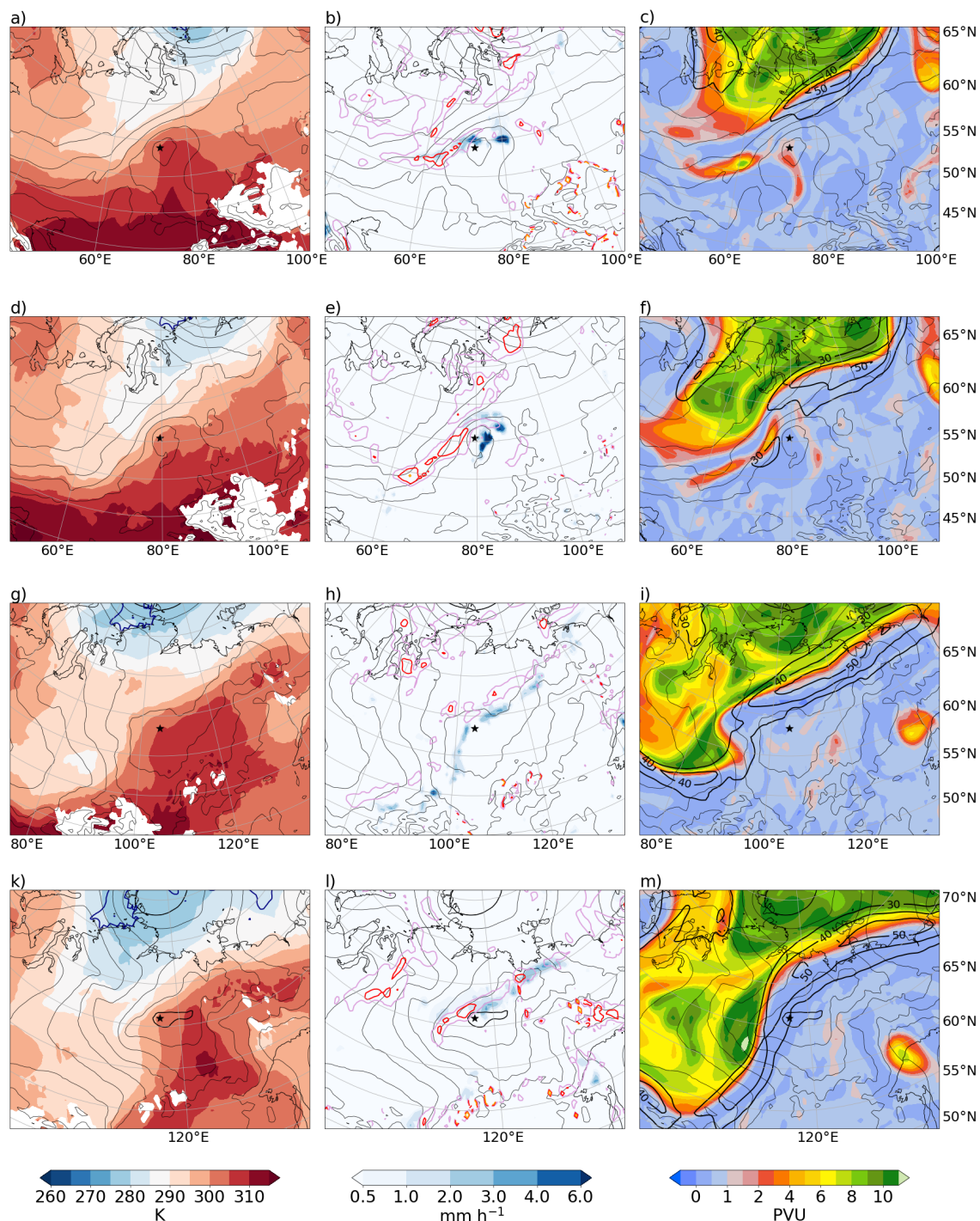
Figure 6. Same as Fig. 4, but during the propagation phase of the cyclone at (a-c) 20 UTC on 4 July, (d-f) 12 UTC on 5 July, (g-i) 12 UTC on 7 July, and (k-m) 16 UTC on 8 July 2021. The slightly bolder SLP contour around the cyclone centre in (k-m) indicate the 990 hPa contour.
