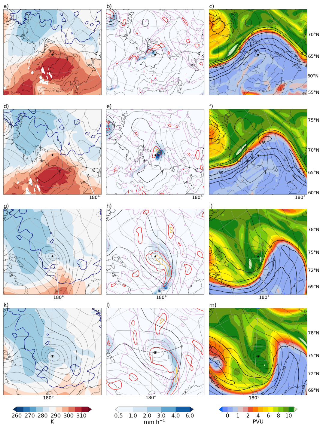
Figure 7. Same as Fig. 4, but during the intensification phase of the cyclone at (a-c) 12 UTC on 9 July, (d-f) 19 UTC on 9 July, (g-i) 12 UTC on 10 July, and (k-m) 18 UTC on 10 July 2021. The gray dashed line in Fig. 7l indicates the location of the vertical cross section in Fig. 5b, and the blue contour in the left panels indicates a sea ice concentration of 75%.
