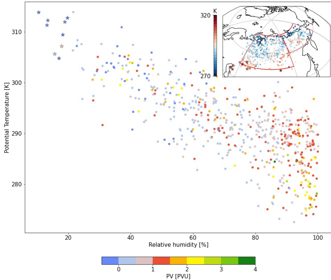
Figure 1. ERA5 climatology (1979–2021) of near surface conditions at the time of cyclogenesis for all identified Siberian summer cyclones. The scatter plot shows \theta versus relative humidity, and the color of the symbols indicates low-tropospheric PV. Siberian heat lows (in the upper left corner of the diagram) are denoted with a star. The map shows the cyclogenesis locations of all cyclones, and the color of the dots indicates \theta at the time of cyclogenesis. The considered area of interest is indicated by the red contours in the map.
