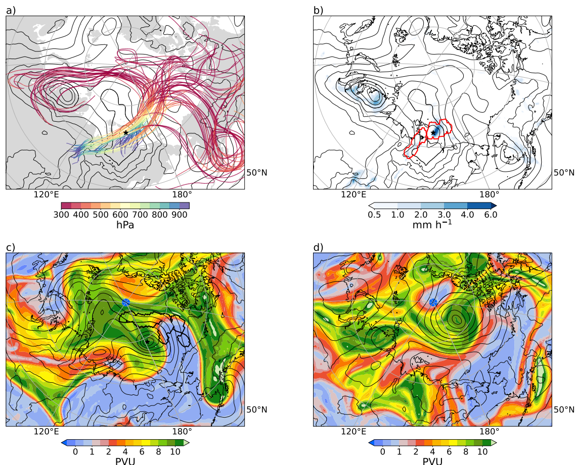
Figure 8. WCB trajectories and their implications during the cyclone's rapid intensification phase. (a) WCB trajectories that are in their ascent phase (500-800 hPa) at 18 UTC on 9 July. (b) Precipitation rates (colour) and WCB ascent mask (red contour) at 18 UTC on 9 July. (c) and (d) PV on 330 K at 18 UTC on 10 July and at 01 UTC on 13 July, respectively. The WCB outflow mask (thick black line) at 18 UTC on 10 July is additionally shown in (c). All panels show SLP (black lines, every 4 hPa).
