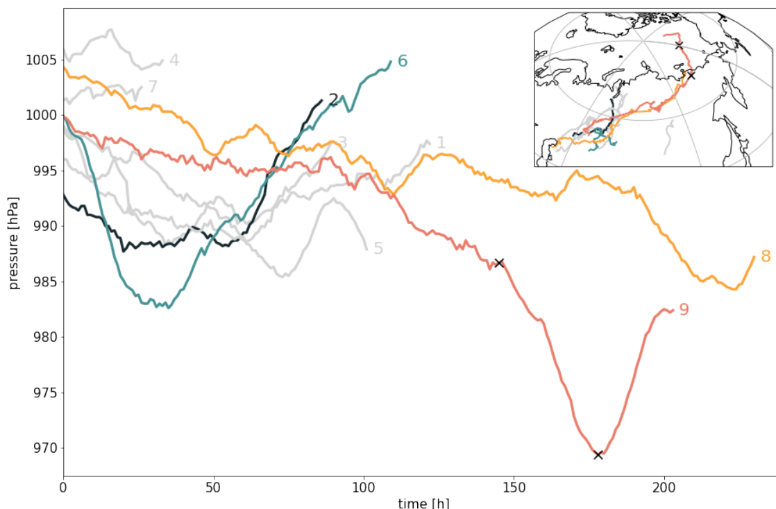
Figure 2. Tracks of the Siberian heat lows and time evolution of minimum SLP. The labels correspond to the event numbers in Table 1. The tracks highlighted in color are discussed in more detail in this paper. Cyclone 9 (red) is the main focus of this study. The 2 black crosses along the pressure evolution and track of this cyclone indicate the time and position of the cyclone at the onset of rapid intensification and maximum intensity, respectively.
