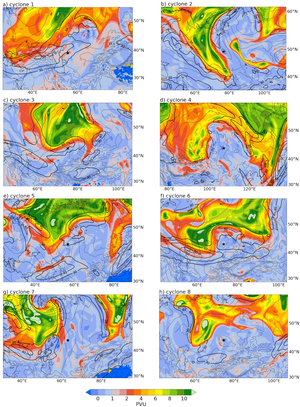
Figure 10. Upper-level PV (color) and wind speed (black contours, every 10 m s -1 starting at 30 m s -1 ) at a chosen time during the life cycle of: (a) cyclone 1 at 14 UTC on 21 August 1983 (2 h after cyclogenesis), (b) cyclone 2 at 22 UTC on 06 June 1985 (56 h after cyclogenesis), (c) cyclone 3 at 17 UTC 04 August 1991 (5 h after cyclogenesis), (d) cyclone 4 at 14 UTC in 12 June 2004 (7 h after cyclogenesis), (e) cyclone 5 at 08 UTC on 13 August 2004 (15 h after cyclogenesis), (f) cyclone 6 at 20 UTC on 12 July 2005 (9 h after cyclogenesis), (g) cyclone 7 at 23 UTC on 18 July 2012 (11 h after cyclogenesis, and (h) cyclone 8 at 17 UTC on 26 July 2017 (78 h after cyclogenesis). All panels are cyclone centred (the centres are additionally indicated with a star) and the faint black contours show SLP in every panel (990 hPa and 970 hPa contours are highlighted with bolder contours).
