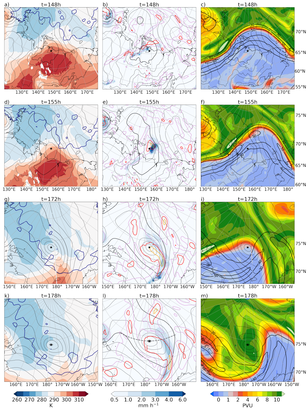
Figure 7. Same as Fig. 4, but during the intensification phase of the cyclone at (a-c) 12 UTC on 9 July ( t = 148 h), (d-f) 19 UTC on 9 July ( t = 155 h), (g-i) 12 UTC on 10 July ( t = 172 h), and (k-m) 18 UTC on 10 July 2021 ( t = 178 h). The gray dashed line in Fig. 7l indicates the location of the vertical cross section in Fig. 5b, and the blue contour in the left panels indicates a sea ice concentration of 75%.
