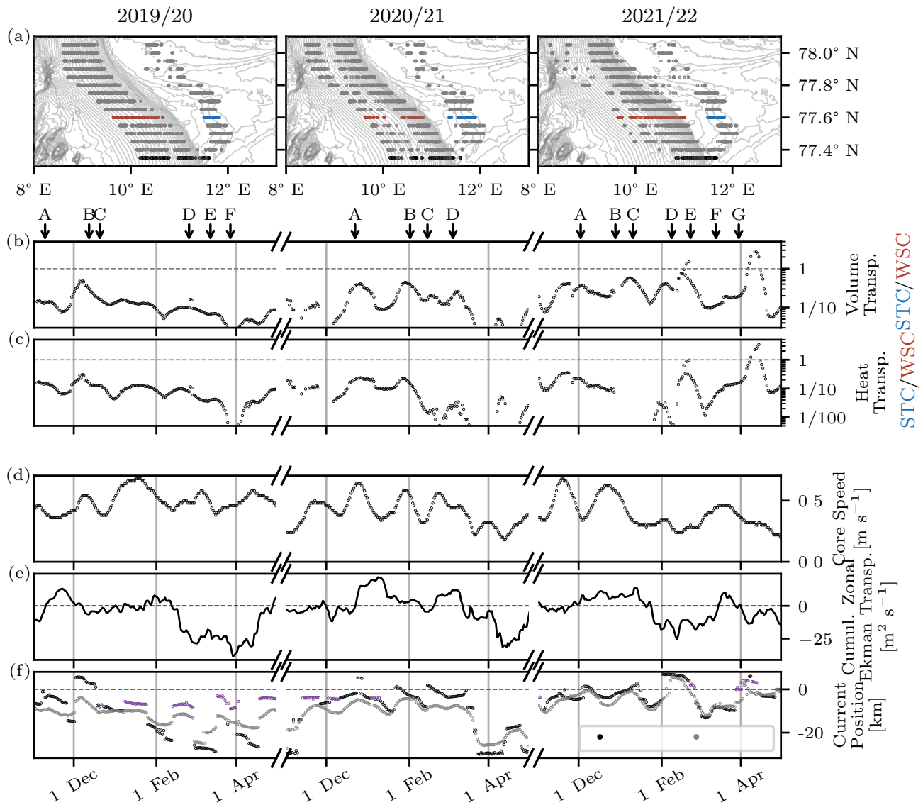
Figure 7. (a) Composites of core positions of the WSC over the continental slope and the STC on the outer WSS during the three winter seasons 2019/20, 2020/21 and 2021/22. WSC and STC core positions at 77.6° N are colored red and blue, respectively, and all core positions at 77.5° N are colored black. (b) – (f): Time series of the ratios between WSC and STC in the volume and heat transport, northward current core speed, cumulative zonal Ekman transport (spatially averaged over the whole WSS break area, see Figure 2 (b)) and WSC core position throughout the three winter seasons. At 77.5° N, the shelf break ( x=0 km, indicated with the dashed horizontal line in (f)) is located at 340 m depth. The onset times of all warming events are indicated with black arrows on top of (b). The gaps in (c) result from negative heat transport values, as the temperatures of the water mass transported by the STC on the shelf drops below the reference temperature of 0°C. In (f), WSC core positions during times when the core depth is found below 150 m are colored in purple.
