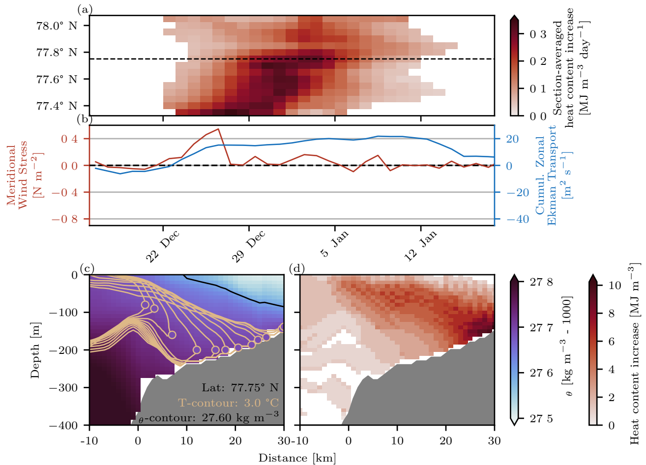
Figure 3. (a): Zonal- and depth-averaged heat content increase on the shelf as function of time and latitude for the warming event 2020/21-A. (b): Time series of spatially averaged meridional wind stress (red axes and graphs) and resulting cumulative zonal Ekman transport (blue axes and graphs) during the same warming event period. (c): Day-to-day propagation of one specific isotherm at one zonal section over the course of the warming event (isotherm and latitude values given in the lower right, the latitude is also indicated by the dashed horizontal line in (a)). The colored circles at the easternmost point of each isotherm line show the initial potential density anomaly (day 0 of the warming) of this point. The color-coded background is a composite of potential density anomalies at different time steps. For the x-range behind the colored circles, it is individual potential density anomaly profiles at the x-locations matching the maximum eastward extension of the isotherm at each time step during the warming event. The background data west of the circle on the initial isotherm is filled with data from the initial time step, the background data east of the circle on the final isotherm is filled with data from the final time step. In cases when the isotherm progresses further than 1 km over one day, the background density data is linearly interpolated. The black contour line indicates one example potential density anomaly level (value given in the lower right of each panel), to illustrate the tilt of the density front. (d): Zonal cross-sections of the final heat increase on the shelf due to the warming events at 77.75° N.
