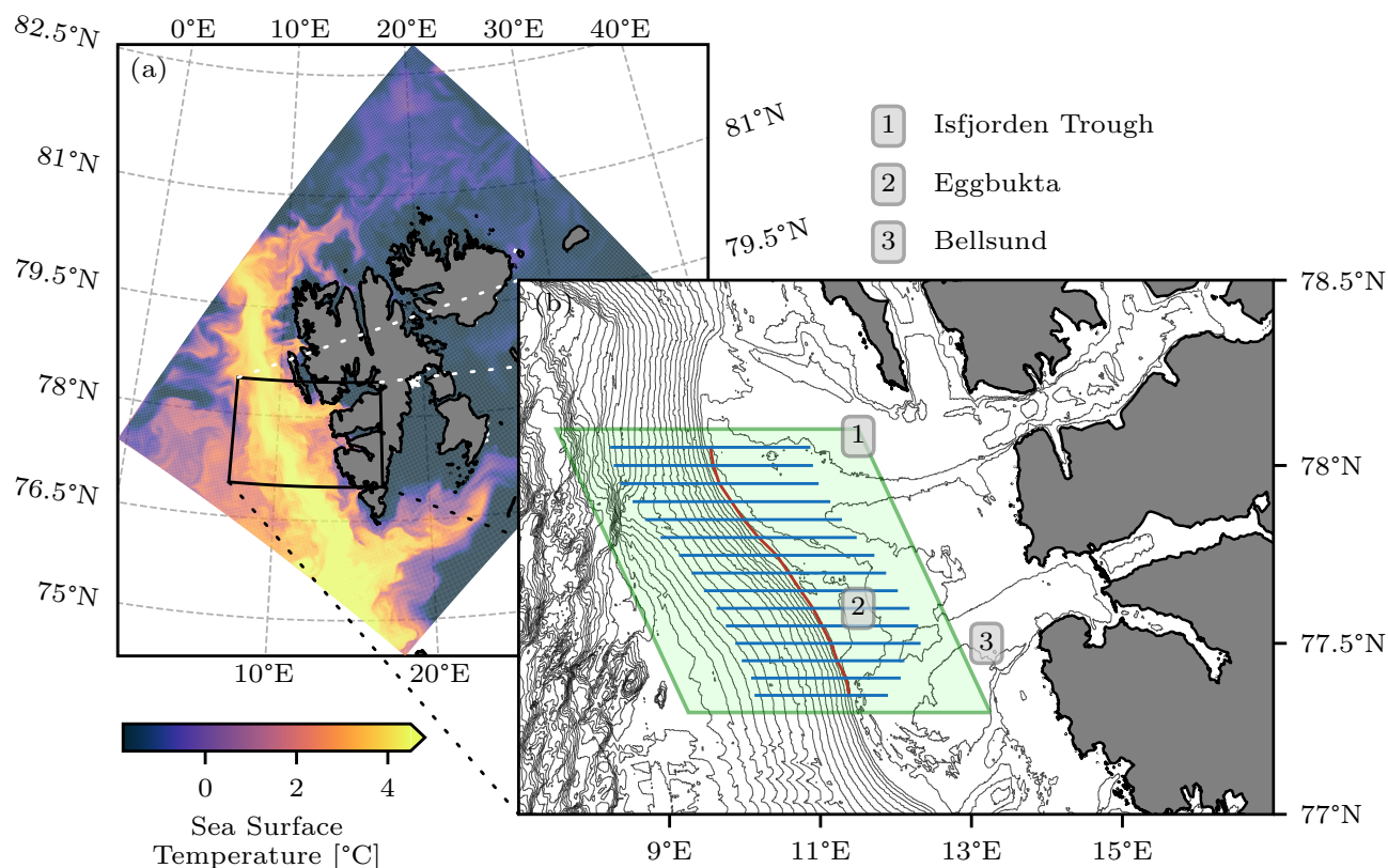
Figure 2. (a) Simulated SST over the whole ROMS model domain on 01.02.2020 12 UTC. (b) Zoom into the WSS region west of Spitsbergen. The red line marks the WSS break and the blue lines mark the 15 zonal sections used to analyze the warming events and the corresponding cross-shelf exchange mechanisms. The light green shading highlights the area over which the atmospheric wind forcing is evaluated.
