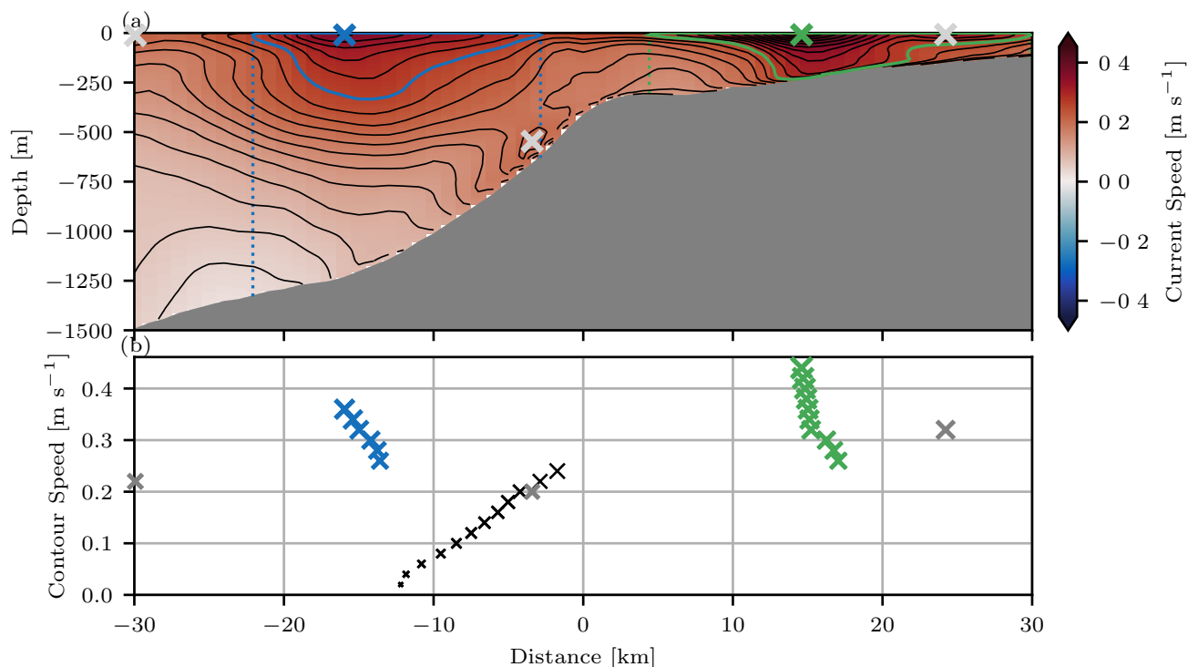
Figure C1. (a) Current speed cross section at 77.6^\circ N on 09.12.2019, with overlaid contour lines (black). Positions of peaks included in the analysis are indicated in color, peaks discarded due to insufficient total strength or prominence in light grey. The colored contours highlight the lowest contour line solely contributing to the peak marked with the corresponding color. The dotted vertical lines show the x-range associated with each current branch. (b) x-Positions of the geometric centers of each individual contour element shown in (a). Discarded peaks again in grey and the peaks remaining for further analysis in color.
