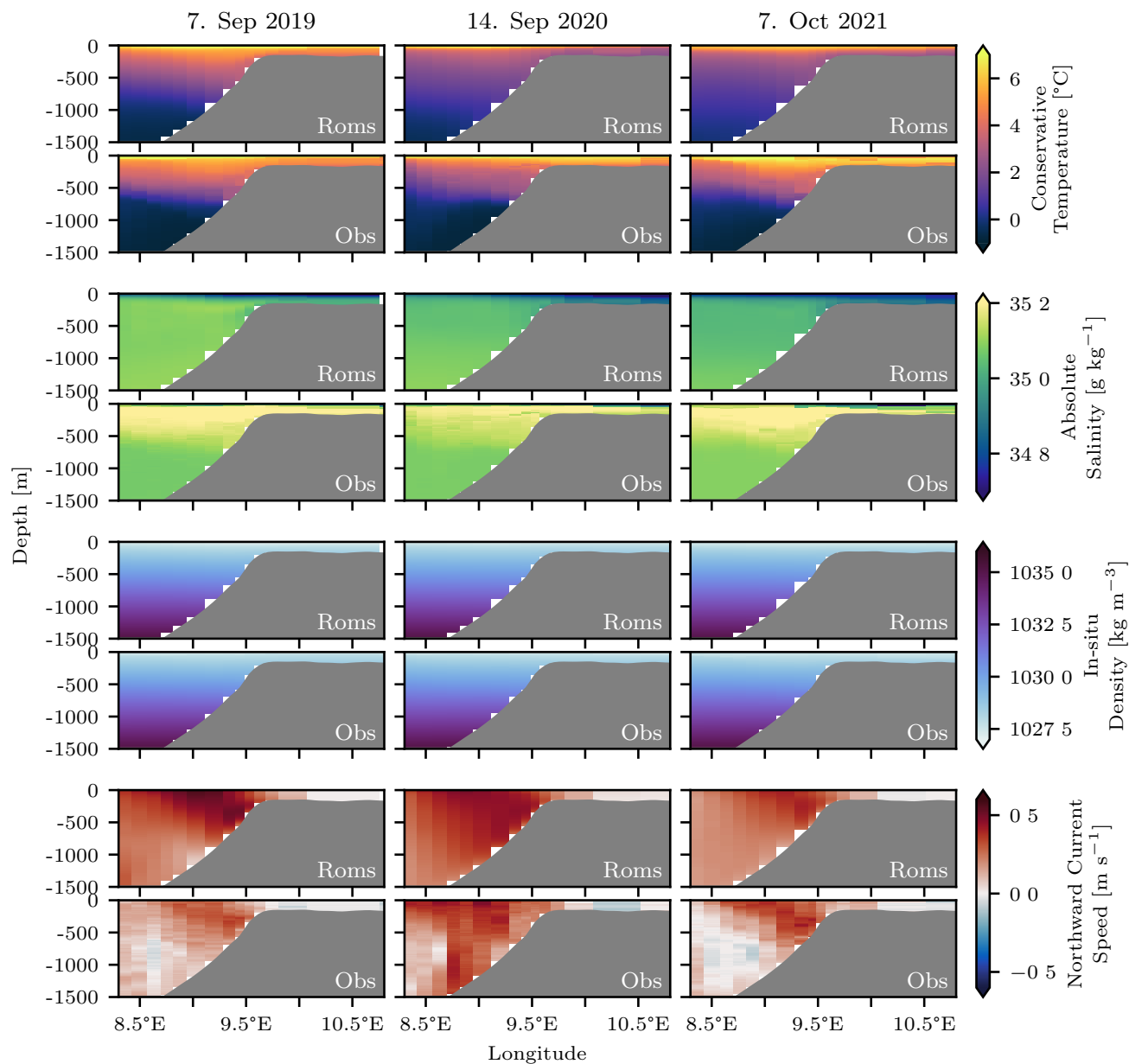
Figure D2. ROMS-simulated hydrography at the 78.0° N-section compared to observations (hydrography: CTD profiles, currents: lowered ADCP) in autumn before each of the three winters seasons investigated in this study.
