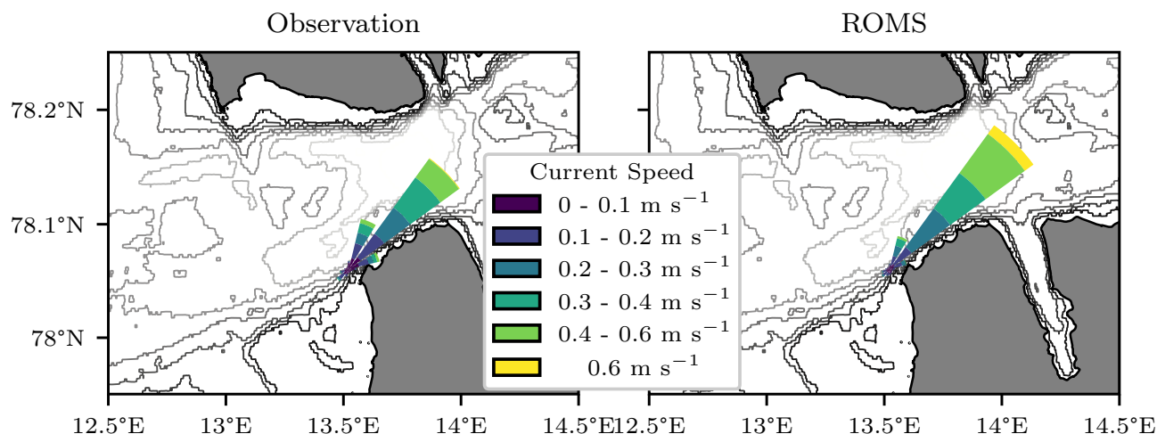
Figure D4. Comparison of current roses between mooring observations and ROMS simulations, based on the full two-year time period. The centers of the current roses are placed at the actual mooring location. The bathymetry is shown as gray contour lines in the background (50-m-spacing, fading with depth).
