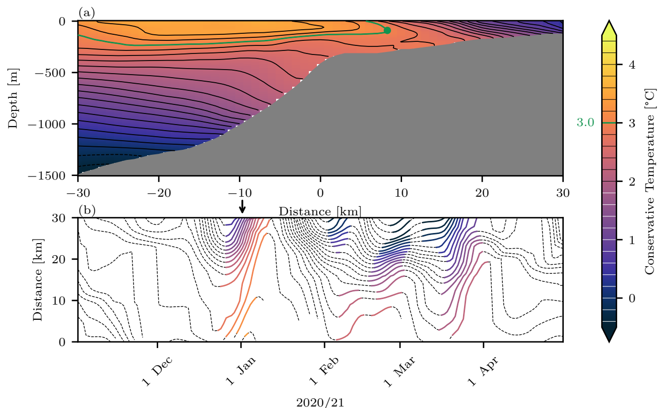
Figure B1. (a) Temperature cross section at 77.6° N on 01.01.2021. The black lines indicate the isotherms used to identify the warming events. The 3°C-isotherm is highlighted in green as an example and its easternmost point is marked with a round marker. (b) Time series of the on-shelf x-position of the easternmost points (the green marker for the example contour in (a)) for all isotherms during the winter season 2020/21. Those periods identified as a warming event are marked with color, corresponding to the value of the respective isotherm. The black arrow indicates the time of the cross section snapshot shown in (a).
