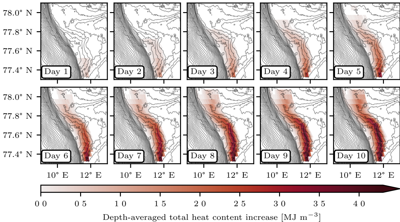
Figure 6. Horizontal day-to-day development of the depth-averaged total heat content increase on the WSS during the ten first days of warming event 2019/20-B.
