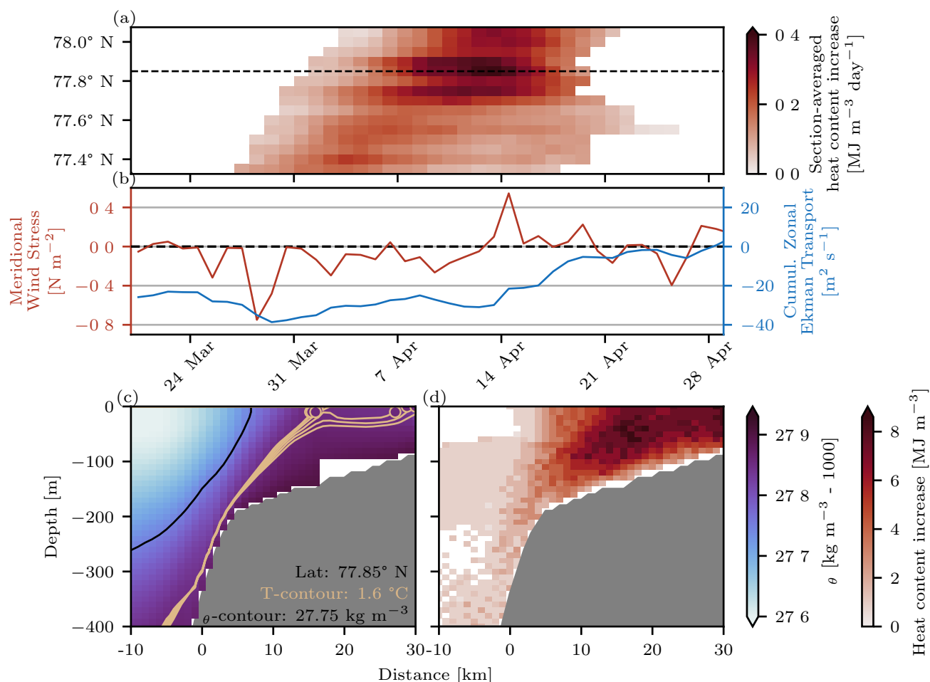
Figure 4. Same as Figure 3, but for warming event 2019/20-F.
