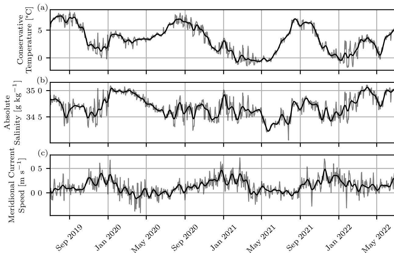
Figure A1. Time series of (a) temperature, (b) salinity and (c) meridional current speed at an example point from the WSS break section at 77.9° N at x=5 km in 10 m depth. The light curves in the background display the raw daily values, the opaque curves on top show the low-pass filtered smooth time series used for the further analyses.
