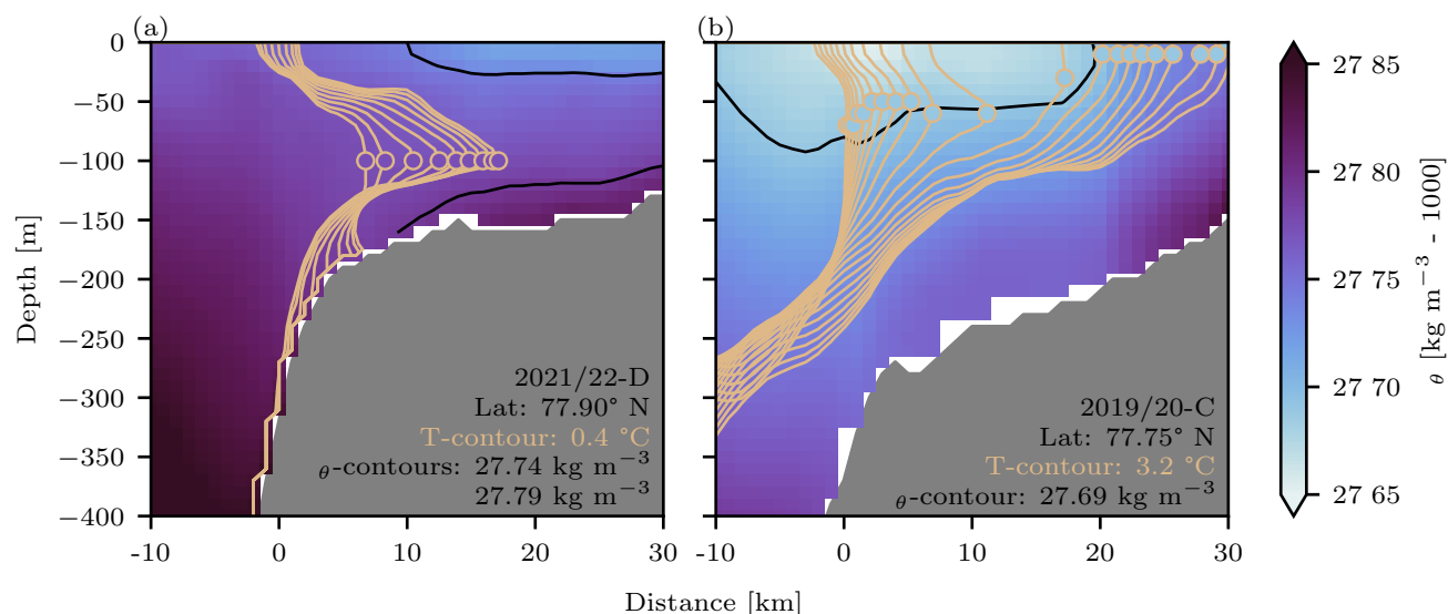
Figure 5. Same as Figure 3 (c), but for the warming events 2021/22-D and 2019/20-C
