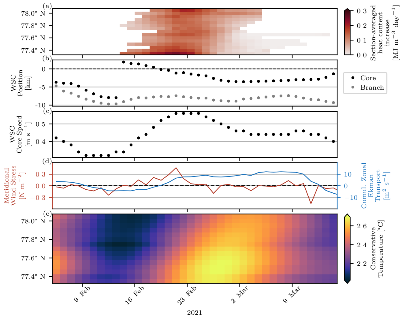
Figure 8. (a) Zonal- and depth-averaged heat content increase on the shelf as function of time and latitude during the warming event 2020/21-C. (b) Time series of the WSC core (black markers) and average branch position (light gray markers) at 77.35° N. (c) Time series of WSC northward core speed at 77.35° N. (d) Time series of spatially averaged meridional wind stress (red axes and graphs) and resulting cumulative zonal Ekman transport (blue axes and graphs). (e) Average temperature of the upper 150 m of the water column over the slope ( x < 0 km) as function of time and latitude.
