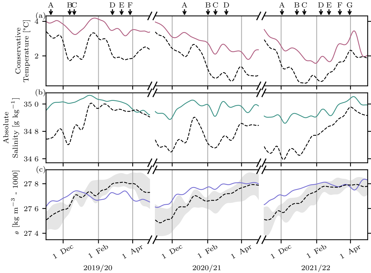
Figure 9. Average conservative temperature, absolute salinity and potential density anomaly of the upper 300 m of the water column over the slope ( x < 0 km, colored solid lines) and the shelf ( x > 0 km, black dashed lines) at 77.6^\circ N. In panel (c), the gray shading furthermore indicates the range of the average surface and bottom potential density anomaly on the shelf. The onset times of all warming events are indicated with black arrows on top of panel (a).
