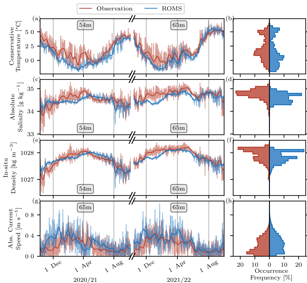
Figure D3. Comparison of observed and simulated conservative temperature (a), absolute salinity (c), in-situ density (e) and absolute current speed (g) at the location of the mooring in the mouth of Isfjorden. The light curves in the background display unfiltered hourly values, the opaque curves on top show the low-pass filtered smooth time series similar to the data used in the main study. The overall data distributions of the respective variables are shown in the right side panels (b) – (h), with colors matching the graphs in (a) – (g).
