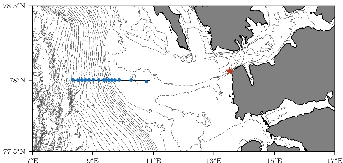
Figure D1. Positions of the 78.0° N-section across the WSS break as used in this study (black line), together with the positions of relevant CTD/lowered-ADCP stations (blue points) covered as part of the operational UNIS ocean observation program. The location of the mooring in the mouth of Isfjorden is shown with a red star.
