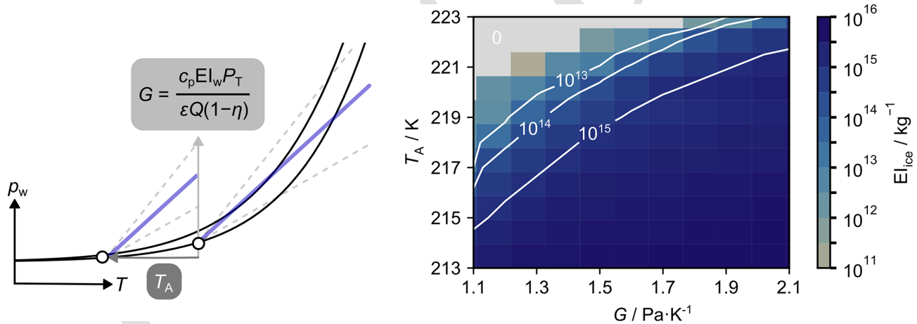
Figure 10. The dependence of contrail AEI_{ice} on T_A and the gradient of the contrail mixing line, as defined in Eq. (1). The simulation was performed for sulfur-rich plume vPM and EI_{nvPM} of 10^{12} \text{ kg}^{-1} , in line with the “soot-poor” baseline conditions described in Sect. 4.4. The region shaded in grey corresponds to AEI_{ice} = 0 . Physically, this represents mixing lines that do not intersect the water saturation line.
