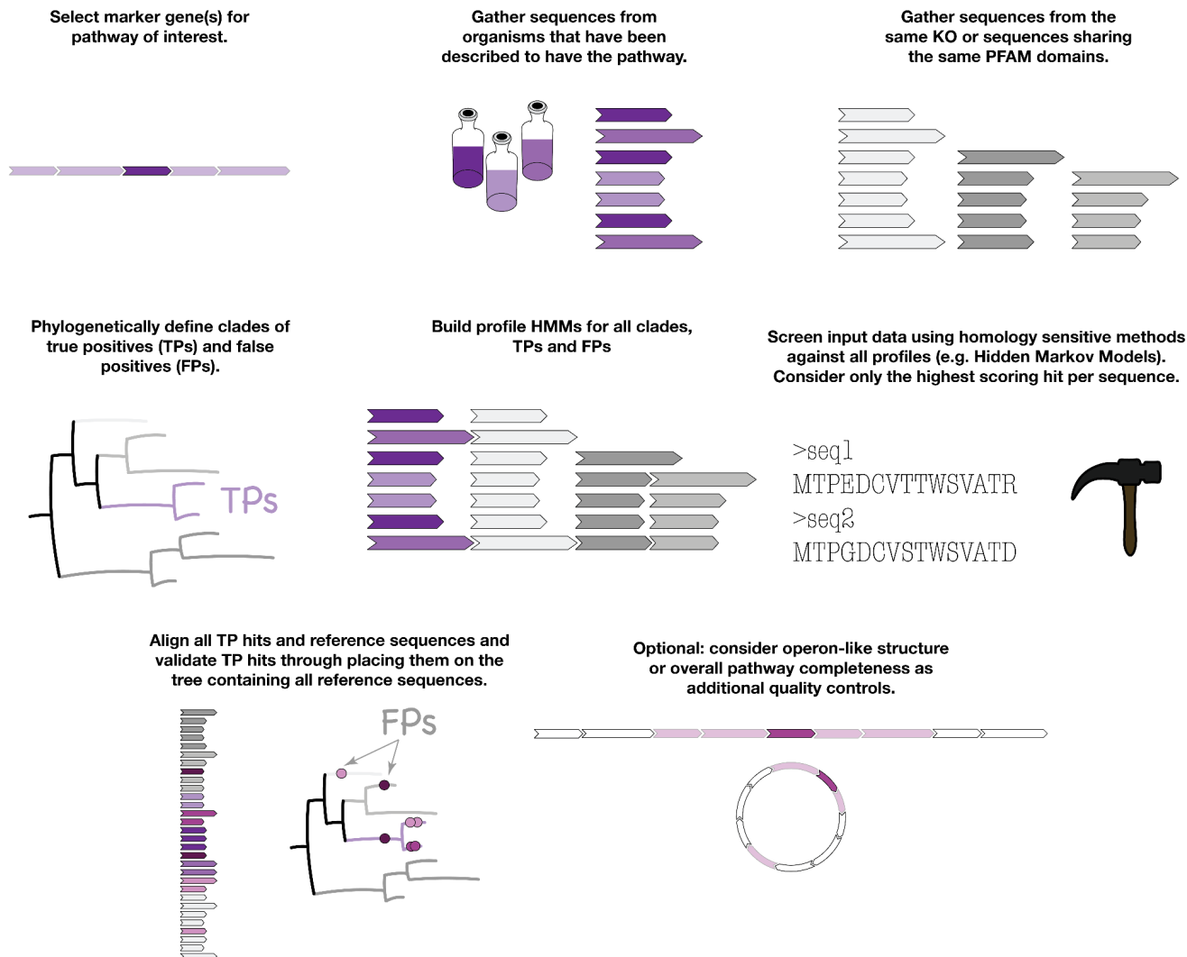
282 Figure 2: Methodological workflow for the robust screening and functional annotation of biogeochemically relevant pathways in 283 large-scale metagenomic data. The strategy utilizes a multi-stage verification process to ensure high-specificity annotations, starting with 284 the selection of specific marker genes and the gathering of reference sequences from known organisms and shared protein domains, such as 285 PFAM. These reference sequences are used to phylogenetically define clades of true positives (TPs) and false positives (FPs) to build profile 286 Hidden Markov Models (HMMs) for precise screening. Input metagenomic sequences are then screened using homology-sensitive methods, 287 with potential hits validated by placement onto the reference phylogenetic tree to confirm their functional identity. To further handle technical 288 uncertainty and ensure metabolic functionality, an optional final step evaluates the genomic context for operon-like organization or overall 289 pathway completeness within the reconstructed Metagenome-Assembled Genome (MAG).
