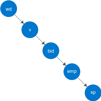
Figure 7: Bayesian network structure showing interdependencies among factors and damage types, derived from a score-based structure learning algorithm.
