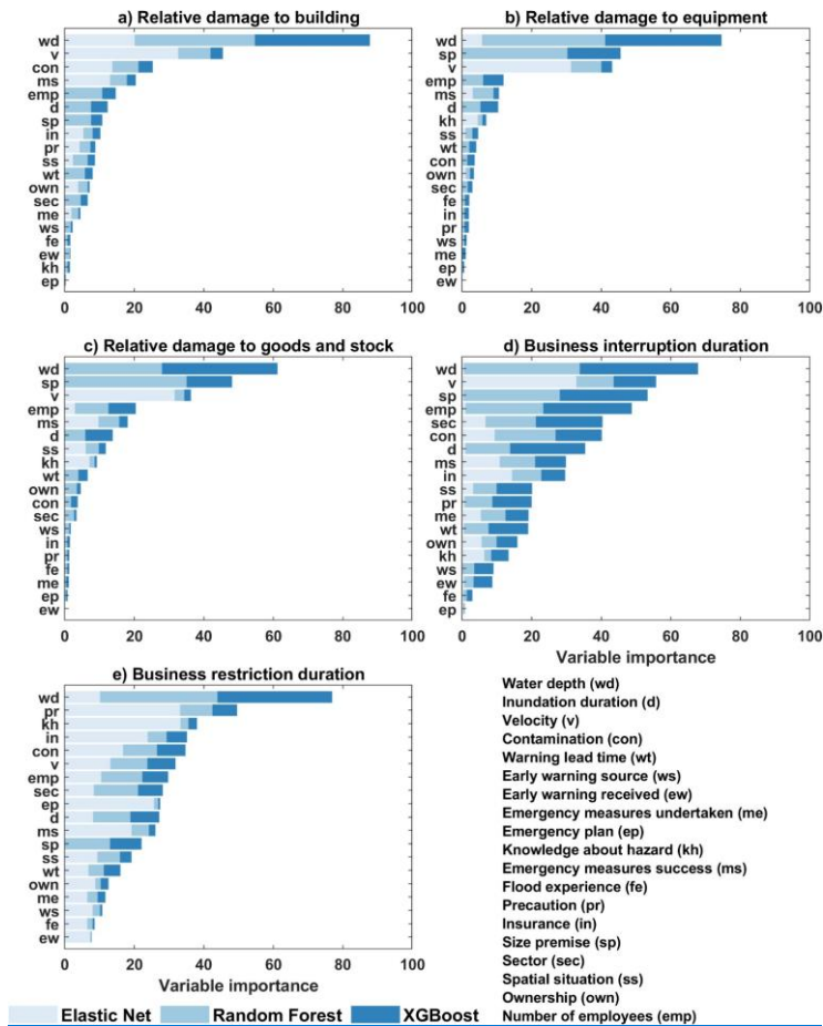
Figure 5: Importance of influencing variables (see Table 1 for abbreviations) for damage types: (a) buildings, (b) equipment, (c) goods & stock, (d) business interruption duration, and (e) business restriction duration. The x-axis shows the weighted importance of each variable, as determined by the three models (Random Forest, Elastic Net, and XGBoost).
