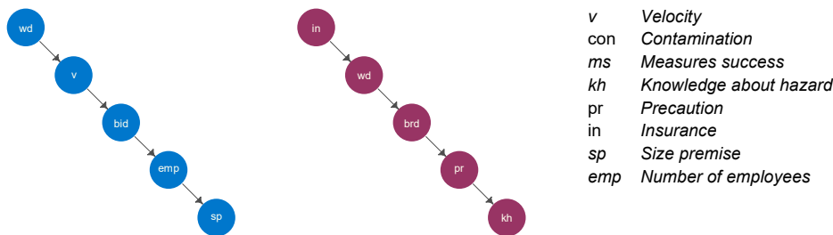
Figure 7: Bayesian network structure showing interdependencies among factors and damage types, derived from a score-based structure learning algorithm.
