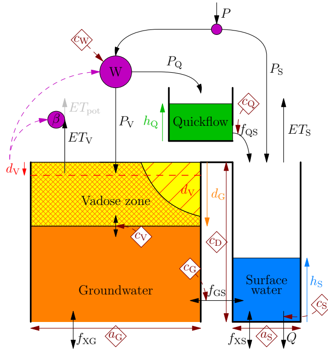
Figure 2. WALRUS model structure with the three reservoirs (orange + yellow, green and blue) and their state variables (coloured arrows), fluxes (black arrows) and model parameters (brown diamonds. Figure copied from Brauer et al. (2014a).
