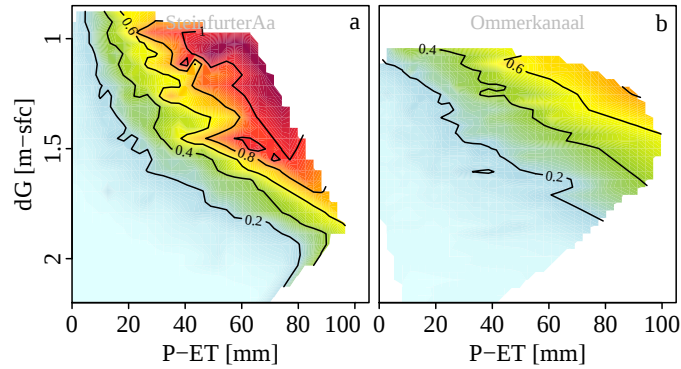
Figure 5. Sensitivity of peak discharge (colour and contour lines in \text{mm h}^{-1} ) to effective rainfall sum ( x -axis) and initial groundwater depth ( y -axis) for two contrasting catchments. Colours represent the same values as the contour lines and are added to make the figures easier to interpret. The surface is interpolated through the cloud of all floods. Figures for the other catchments are provided in the supplement (Fig. S8).
