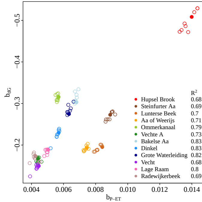
Figure 6. Parameters b_{P-ET} and b_{dG} from Eq. 5, together with the corresponding coefficients of determination ( R^2 ) for all catchments and all scenarios. The filled circles are for the current climate and the open circles for future climates. The colors match the colors in Fig. 3.
