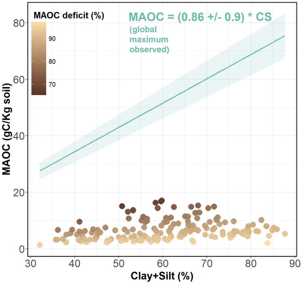
362 Figure 5. Relation between the mineral-associated organic carbon (MAOC) and the percent Clay+Silt 363 (CS) in the soil samples and the boundary line (in blue) with confidence intervals adjusted by Georgiou 364 et al. (2022) for high-activity mineral soils, indicating the maximum observed mineralogical capacity for 365 each CS content. The equation for the boundary line is provided in the panel. Points are colored based 366 on their MAOC deficit (1- MAOC content / MAOC maximum observed capacity).
