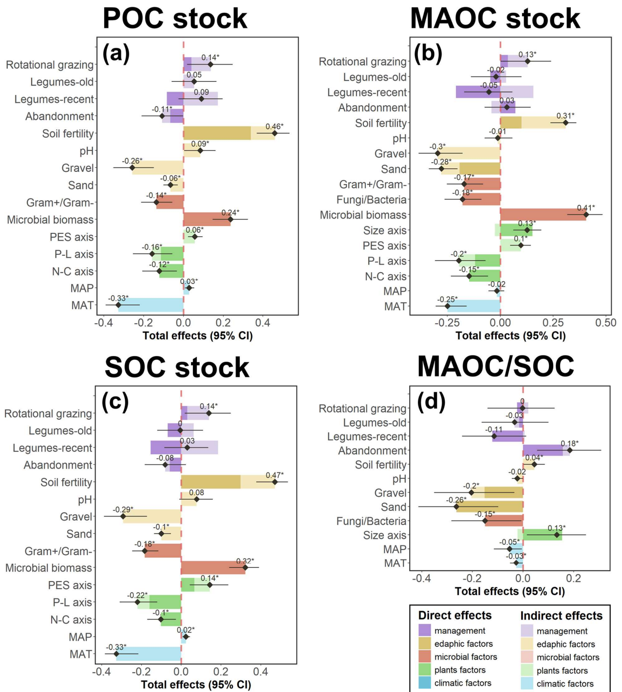
419 Figure 7. Direct, indirect and total standardized effects of all studied variables included in the structural equation model 420 (Figure6) over the (a) particulate organic carbon (POC), (b) mineral-associated organic carbon (MAOC), and (c) soil organic 421 carbon (SOC) stocks and (d) the relative MAOC abundance (MAOC/SOC). Bars indicate direct (dark colors) and indirect 422 (light colors) effects, and the black points-ranges indicate the total (i.e. direct + indirect) effect (with its 95% confidence 423 interval). Stars over the total effect values indicate significant effects at a level of 0.05.
