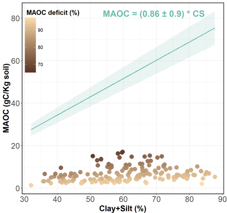
362 Figure 5. Relation between the mineral-associated organic carbon (MAOC) and the percent Clay+Silt (CS) in the soil samples 363 and the boundary line (in blue) with confidence intervals adjusted by Georgiou et al. (2022) for high-activity mineral soils, 364 indicating the maximum observed mineralogical capacity for each CS content. The equation for the boundary line is provided 365 in the panel. Points are colored based on their MAOC deficit (1- MAOC content / MAOC maximum observed capacity).
