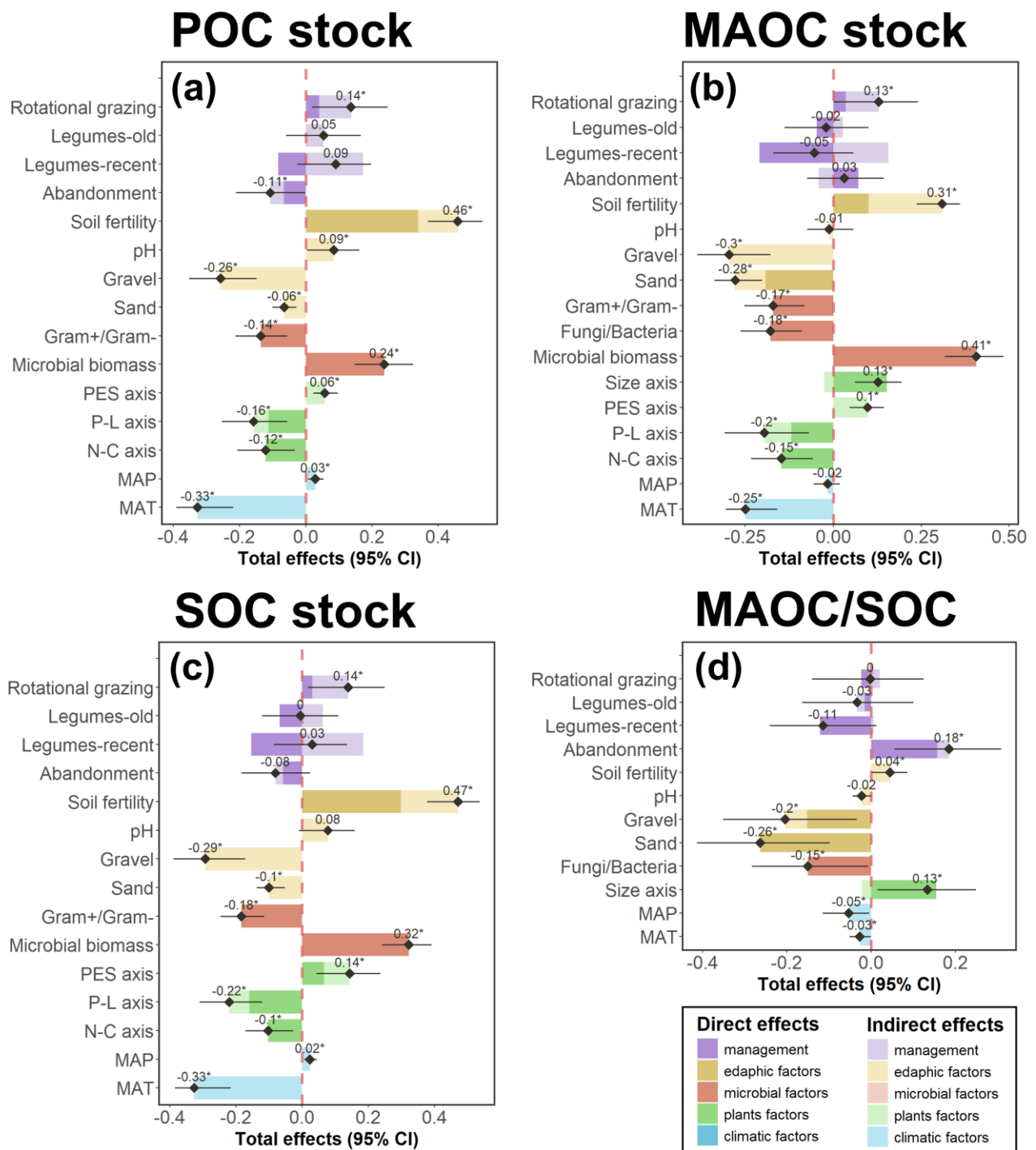
418 Figure 7. Direct, indirect and total standardized effects of all studied variables included in the structural equation model 419 (Figure6) over the (a) particulate organic carbon (POC), (b) mineral-associated organic carbon (MAOC), and (c) soil organic 420 carbon (SOC) stocks and (d) the relative MAOC abundance (MAOC/SOC). Bars indicate direct (dark colors) and indirect 421 (light colors) effects, and the black points-ranges indicate the total (i.e. direct + indirect) effect (with its 95% confidence 422 interval). Stars over the total effect values indicate significant effects at a level of 0.05.
