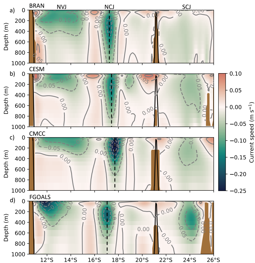
350 Figure 4. South Equatorial Current jet historical assessment (1993 to 2023). Mean current speed meridional 162°E sections for a) BRAN2020 and b) CESM, c) CMCC and d) FGOALS. Positive is eastward. The positions of the NVJ, the NCJ and the SCJ are indicated. The black dashed lines show the latitude of maximum NCJ current speed. The model bathymetry is shown in brown, and the GEBCO 2023 bathymetry is overlaid as solid black lines (GEBCO, 2024). Contours are in grey; positive contours and solid and negative contours are dashed.
