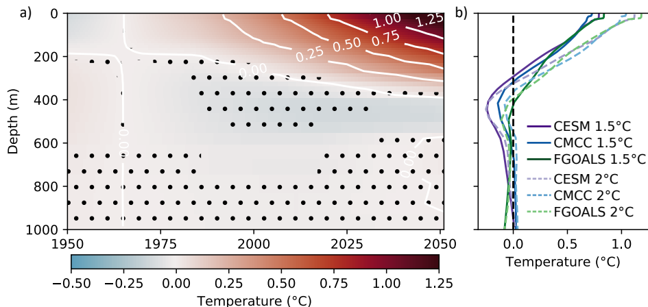
435 Figure 5. Warming in the Coral Sea. a) HighResMIP model ensemble mean Coral Sea temperature anomaly (relative to 1950 – 1979). Contours are in white; positive contours and solid and negative contours are dashed. The stippling indicates depths/times when all three models did not agree on the sign of the anomaly. b) Temperature anomaly profiles under 1.5° C and 2° C global warming. A different time point was selected for each HighResMIP model, depending on when the model reached 1.5° C and 2° C global warming (Table S1).
