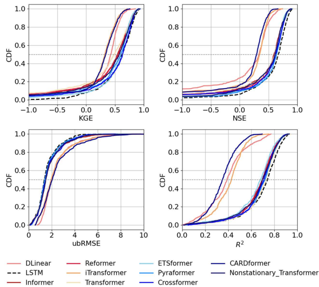
Figure 4. Comparative analysis of the Cumulative Density Functions (CDF) based on spatial cross-validation experiment results. The CAMELS dataset was divided into three folds according to the spatial distribution of the basins. One fold was used as the test set, while the remaining two served as the training set. By cycling through this process, every basin was evaluated as part of the test set. Combined results from all three folds were then used to compute overall evaluation metrics. Horizontal dashed lines indicate median values (CDF = 0.5). Detailed numerical results are provided in Supplementary Table S5.
