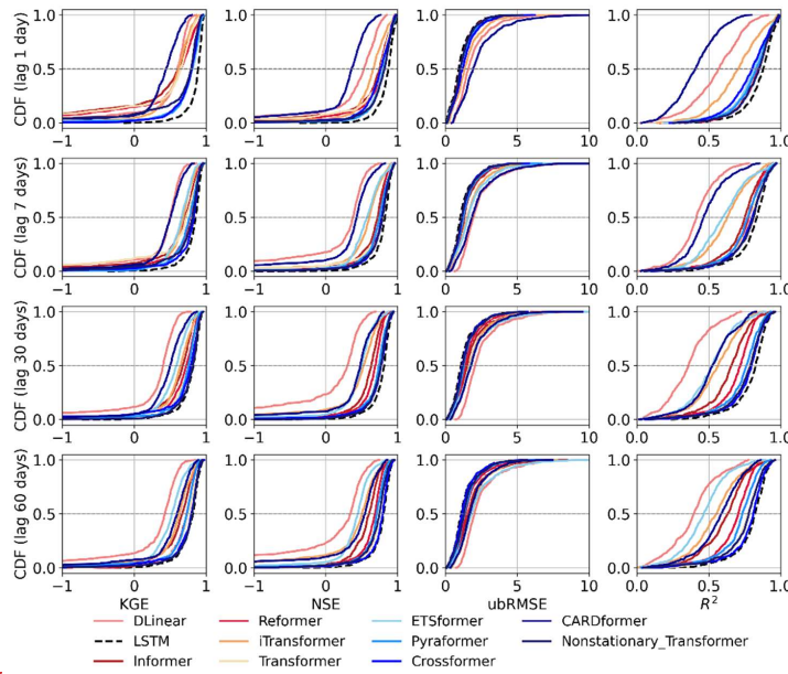
Figure 2. Comparative analysis of the Cumulative Density Functions (CDF) based on results from time-lagged forecasting experiments. The CDF represents the distribution of performance metrics across all basins. The four columns correspond to different evaluation metrics: Kling–Gupta Efficiency (KGE), Nash–Sutcliffe Efficiency (NSE), unbiased Root Mean Square Error (ubRMSE), and Coefficient of Determination ( R^2 ). The four rows represent different time lags: 1 day, 7 days, 30 days, and 60 days. Horizontal lines indicate median values (CDF = 0.5). Detailed numerical results, including median values, are provided in Supplementary Table S2.
