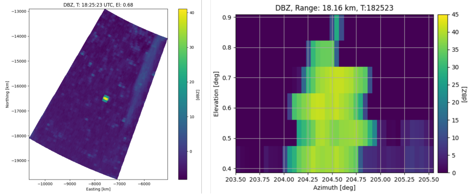
Figure 14. Left: CHILL radar reflectivity sector scan at the elevation of the RTS. Right: Vertical cut of CHILL reflectivity data through 6 sector scans extracted at the location of the generated target.
