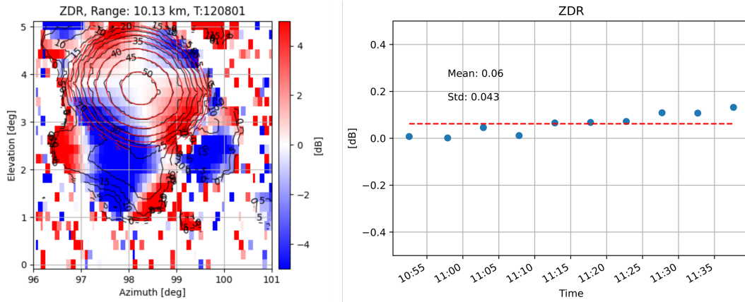
Figure 10. Left: Differential reflectivity pattern of a box scan acquired with the short pulse. Right: Time series of the differential reflectivity where the target Z_{dr} was set to 0 dB.
