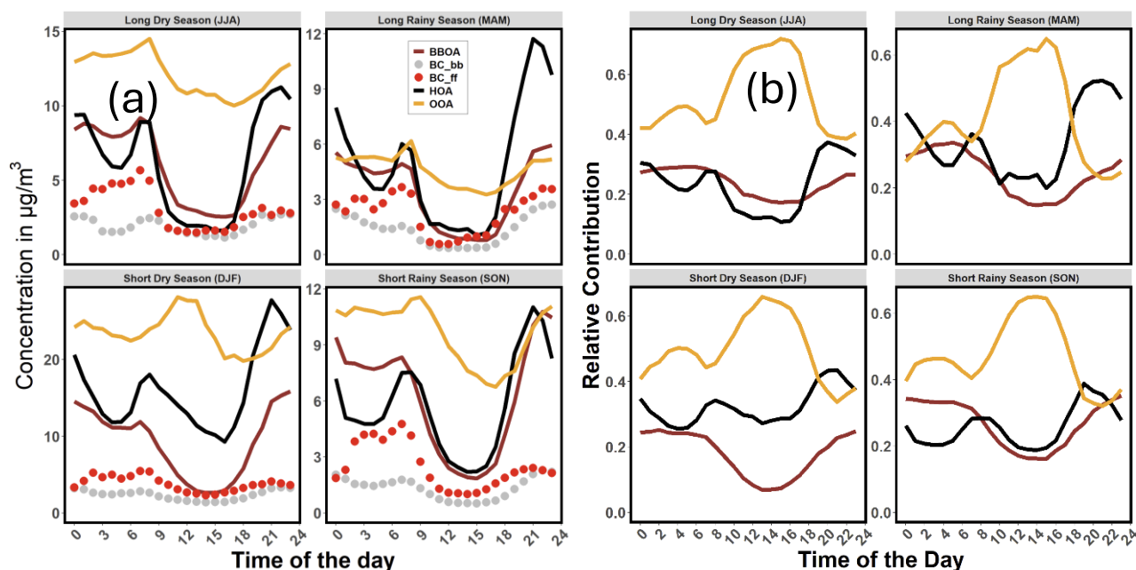
Figure 5: Seasonal diurnal patterns of PMF-resolved organic-only PM 1 sources and BC components (BC- 455 ff and BC_bb), presented as absolute mass concentrations (a) and relative PMF source contributions (b).
