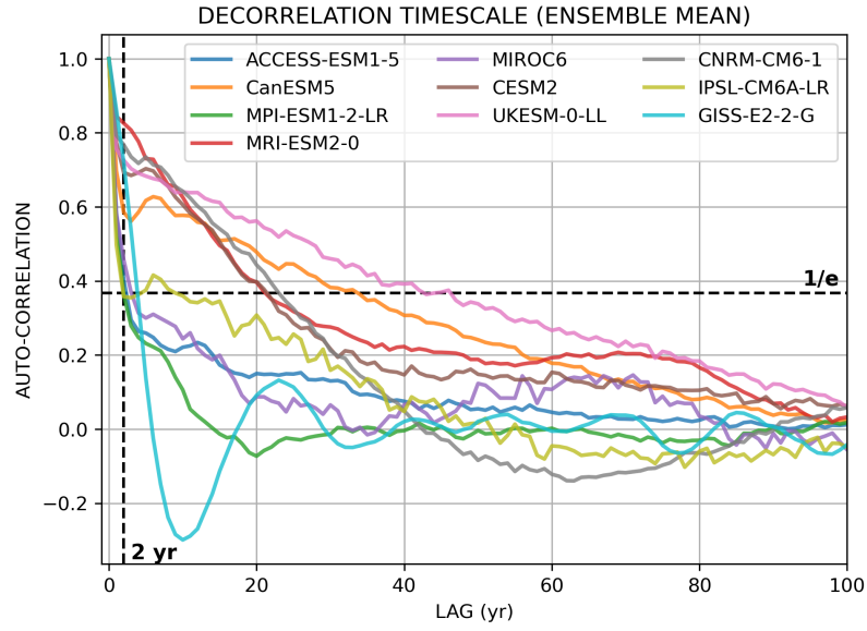
Figure B6. Decorrelation timescale of AMOC intensity time series for each model. Evolution of the normalized auto-correlation with respect to the considered lag. Decorrelation timescale corresponds to the the e-folding timescale, i.e. the lag when the normalized auto-correlation falls below 1/e .
