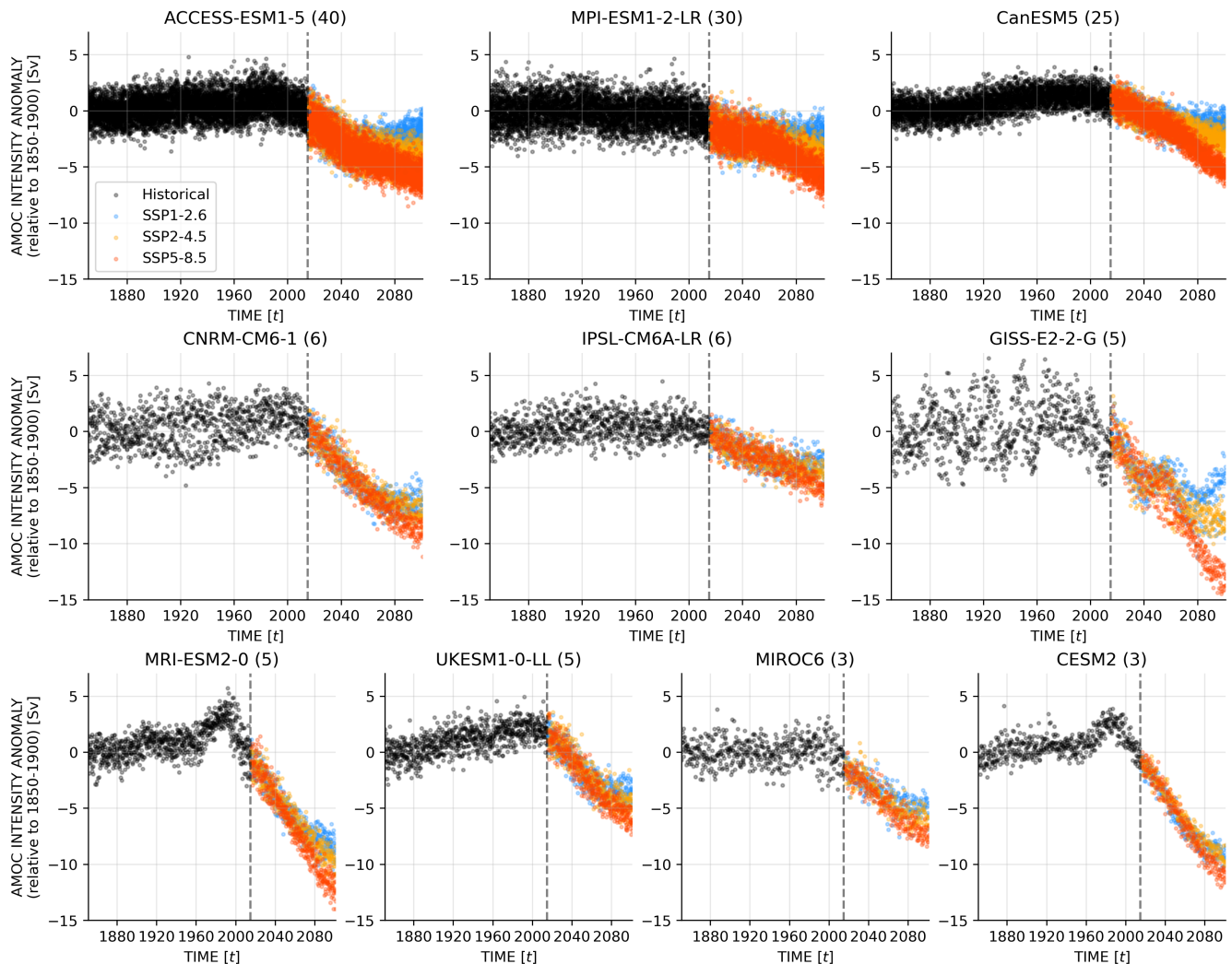
Figure 1. Evolution of AMOC intensity anomaly. Each subplot presents historical time series (black) followed by the three scenarios SSP1-2.6 (blue), SSP2-4.5 (orange), or SSP5-8.5 (red) for a given model. For each model, all realizations/members of the ensemble are shown, and the relative intensity uses as a reference the ensemble average between 1850 and 1900.
