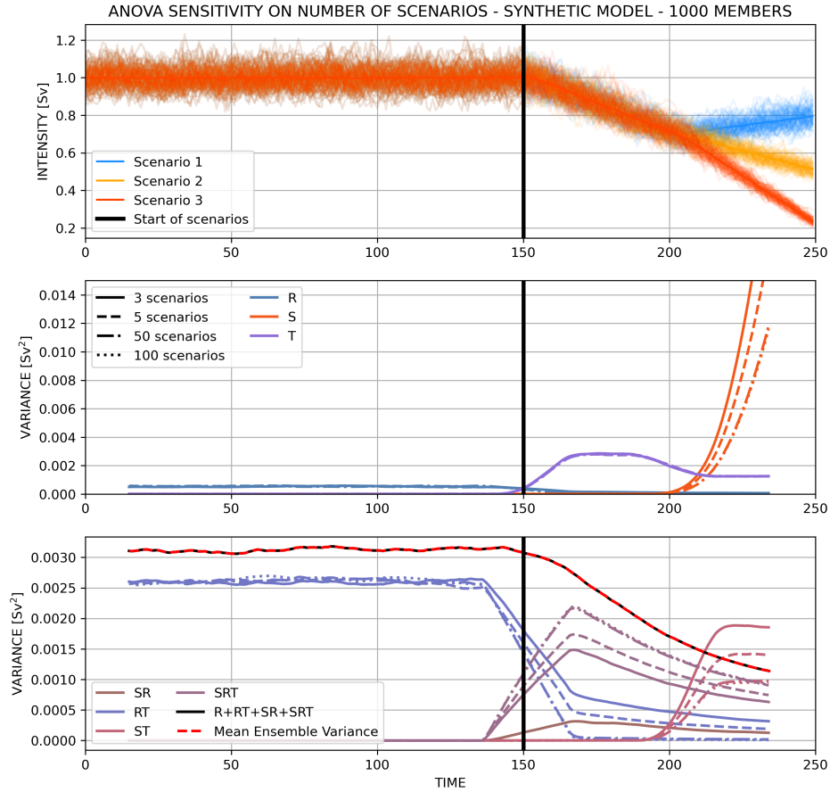
Figure A1. ANOVA decomposition of the synthetic data set. (Top panel) Synthetic AMOC trajectories for 1000 members and 3 scenarios, with a constant first period (years 0-150) where all scenarios are merged, a second period (years 150-200) with the same slope between scenarios but realizations show phase shifts in variability, and a third period (after year 200) where scenarios start to separate and follow different slopes. Internal variability is represented by a random Gaussian noise scaling with the AMOC intensity such that \sigma(\psi_t) = \alpha\psi_t , with \alpha = 0.04 \text{ yr}^{-1/2} ; dt = 1 \text{ yr} . (Middle and bottom panels) ANOVA decomposition of the synthetic data set with separation between the main effects of time (T), scenarios (S), and realizations (R), as well as the interactions between these dimensions. The mean variance of the ensemble (red dotted line) is calculated as the variance of the ensemble (across realizations) averaged over the scenarios and over a sliding window of 30 years. The total internal variability from the ANOVA is calculated from the sum of all factors associated with the R dimension (R, RT, SR, and SRT, black line). The sensitivity of the results to the number of scenarios is represented by different lines of the same color: 3 scenarios in solid line, 5 scenarios in dashed line, 50 scenarios in dash-dotted line, and 100 scenarios in dotted line.
