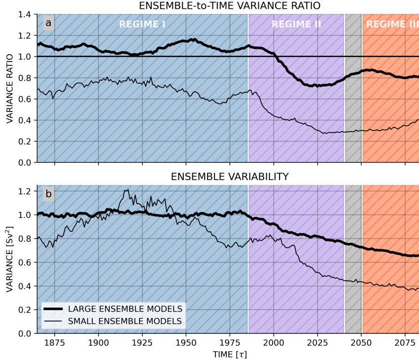
Figure 4. Time and ensemble variance (a) Comparison of their variability with the ensemble-to-time variance ratio. We use this ratio as a proxy of ergodicity. Here ensemble and time variance are derived from the sum of interactions according to the variance reconstruction method described in section 2.2.2. Similar results are obtained using the statistical separation methodology proposed by Zhang et al. (2023). (b) Evolution of ensemble variability (i.e., inter-member spread) over time. Thick lines represent large ensemble models and thin lines small ensemble models.
