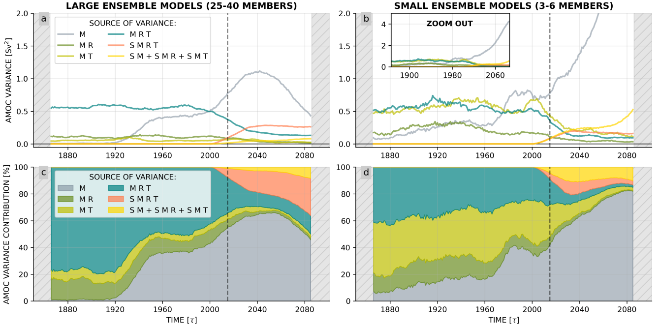
Figure 7. Evolution of the model-associated factors of variability. (a, b) Variance associated to model main effect and interactions. Small and large ensemble models have the same y-axis, and a zoom-out box is displayed for the variance of the small ensemble models to show the full increase in model contribution (b). (c, d) Variance contribution of model main effect and interactions to the total model-associated variability. Letters refer to the dimension involved in the variance calculation, with a single letter for main effects and a combination of letters for interactions: S refers to the scenario dimension, T to time, M to model, and R to realizations (see section 2.2.1). Results are presented for large ensemble models (a, c) with 25-40 members and small ensemble models (b, d) with 3-6 members.
