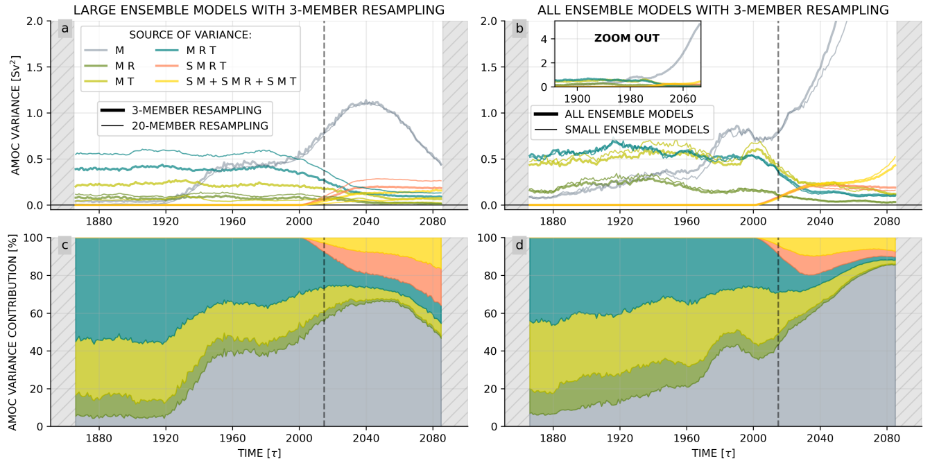
Figure B5. Sensitivity test on bootstrapping methodology: application to the variability of model-associated factors (a, b) Variance associated to model main effect and interactions. (c, d) Variance contribution of model main effect and interactions to the total model-associated variability. Left-hand panels show the sensitivity of the large ensemble results to the number of members in each resampling. Thin lines present the control experiment with 20 members of each model (identical to Fig. 3 a, c, e) and thick lines present the results obtained using 3 members of each model per resampling. Right-hand panels show the sensitivity to combining large and small ensemble models. Thin lines present the control experiment with only small ensemble models (identical to Fig. 3 b, d, f) and thick lines present the results obtained with all ensembles. 3-member resampling are used here.
