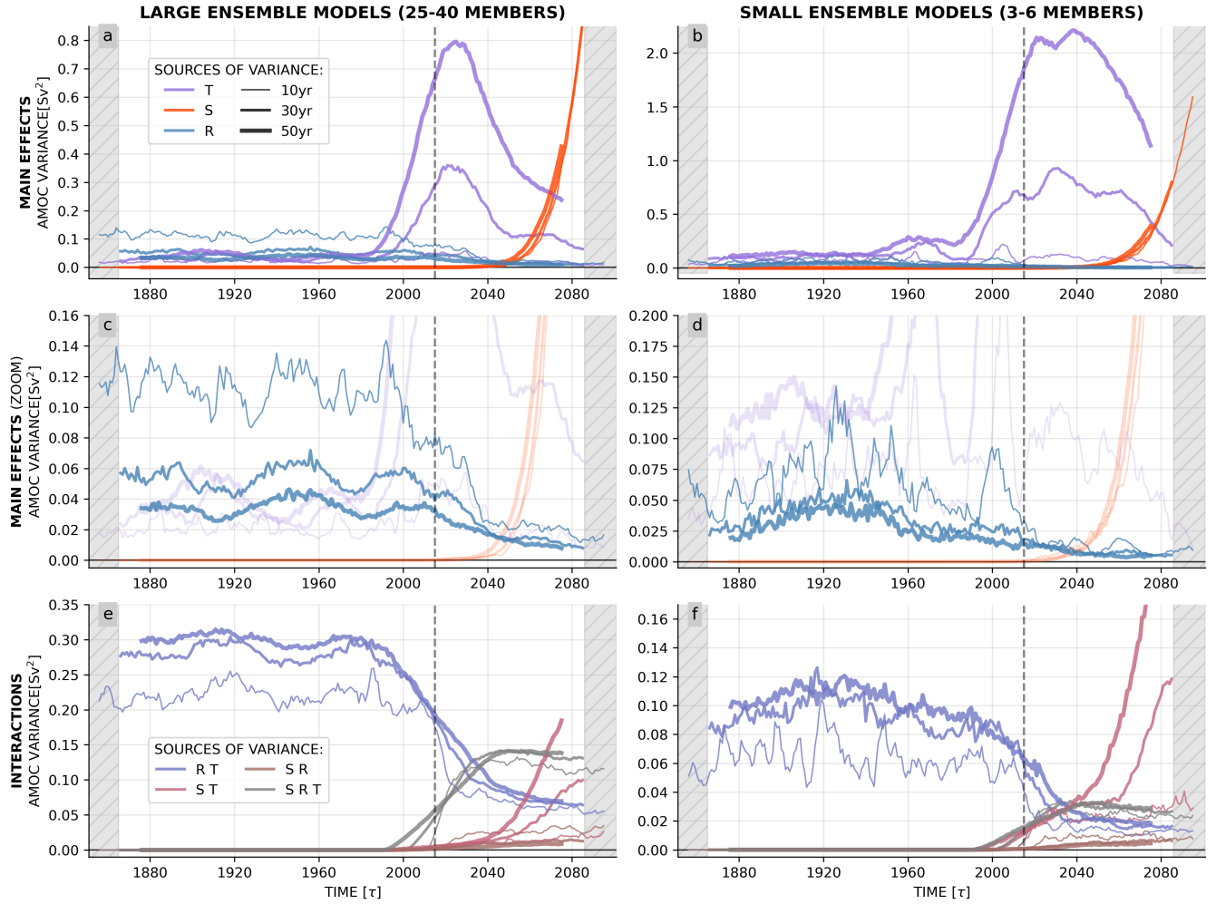
Figure B2. Sensitivity test on time window size. Variance associated to each main effect (a-d) and interaction (e,f). (c,d) Zoom on ensemble main effect. Line thickness represents the size of the time window from 10 (thin) to 50 years (thick). Results are presented for large ensemble models (a, c, e) with 25-40 members and small ensemble models (b, d, f) with 3-6 members.
