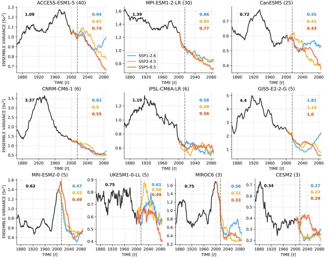
Figure 6. Evolution of internal variability, measured by the ensemble variance, over time and scenarios. Each subplot presents historical time series (black) followed by the three scenarios SSP1-2.6 (blue), SSP2-4.5 (orange), or SSP5-8.5 (red) for a given model. The values written in each subplots correspond to 50-year averaged period of internal variability: 1900-1950 for historical (black) and 2050-2100 for scenarios (colors). A 30-year rolling averaged is applied to isolate long term trends.
