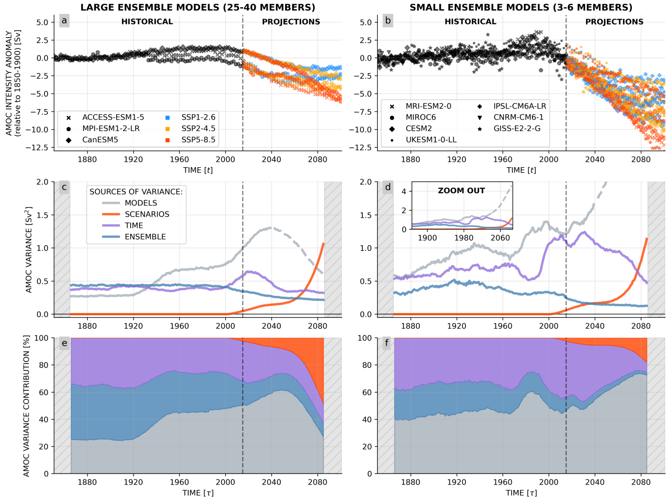
Figure 2. General picture of the AMOC evolution at 26°N from CMIP6 ensemble models. (a, b) Ensemble-averaged AMOC anomaly time series over historical (1850-2015, black) and projection (2015-2100, colors) periods. Reference value is the individual model average from 1850-1900. (c, d) AMOC variance associated with each of the four general factors based on the statistical separation methodology of Zhang et al. (2023). Model contribution has been represented with a dashed line after 2040 to highlight the lack of consistency between c and d regarding this result. Small and large ensemble models have the same y-axis, and a zoom-out box is displayed for the variance of the small ensemble models to show the full increase in model contribution (d). (e, f) Contribution of each factor to the total variance. Results are presented for large ensemble models (a, c, e) with 25-40 members and small ensemble models (b, d, f) with 3-6 members.
