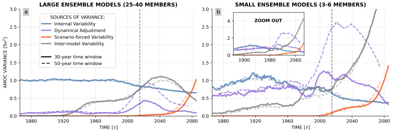
Figure 8. Summary picture of the sources of AMOC variability. (a, b) AMOC variance associated with each of the four sources of variance based on the physical attribution methodology described in section 4. Line style represents the size of the time window, either 30 (solid line), or 50 years (dashed line). Small and large ensemble models have the same y-axis, and a zoom-out box is displayed for the variance of the small ensemble models to show the full increase in model contribution. Results are presented for large ensemble models (a) with 25-40 members and small ensemble models (b) with 3-6 members.
