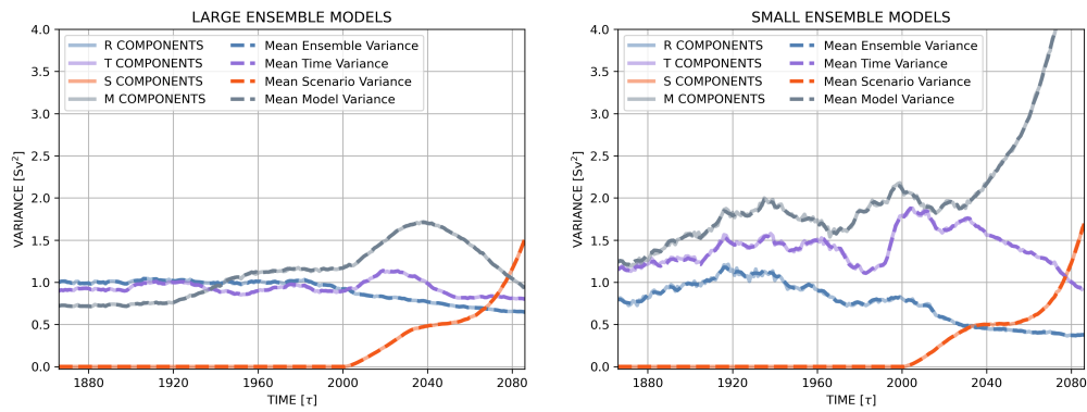
Figure B1. Statistical variance reconstructed from ANOVA components. The mean variance computed across each dimension is compared to the sum of all components involving this dimensions. Results are presented for large ensemble models (left) with 25-40 members and small ensemble models (right) with 3-6 members. Results indicate that the two methods lead to exactly equal time series.
