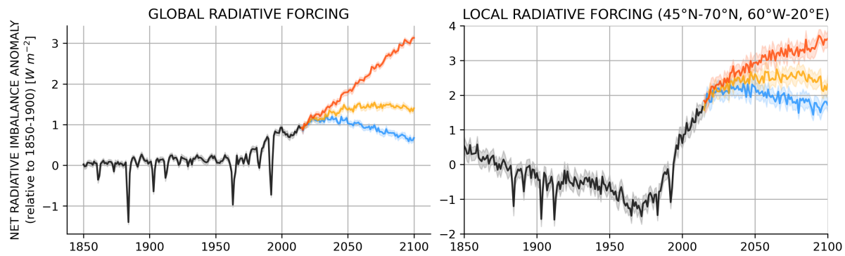
Figure B7. Evolution of the net radiative imbalance averaged across the three large-ensemble models at the global scale (left) and regionally over the North Atlantic (45°–70° N, 60° W–20° E; right). The historical period is shown in black, while future projections are shown in blue (SSP1-2.6), orange (SSP2-4.5), and red (SSP5-8.5). The multi-model mean is calculated using a bootstrapping approach, which is also used to estimate the 95% confidence interval percentiles, displayed as shaded envelopes.
