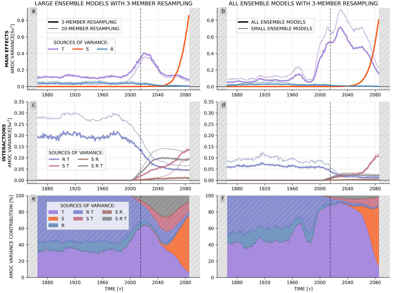
Figure B4. Sensitivity test on bootstrapping methodology: application to the variability of physical factors. (a-d) Variance associated to each main effect (a, b) and their interaction (c, d). (e, f) Relative variance contribution of each main effect and their interactions to the total physical factor variability. Left-hand panels show the sensitivity of the large ensemble results to the number of members in each resampling. Thin lines present the control experiment with 20 members of each model (identical to Fig. 3 a, c, e) and thick lines present the results obtained using 3 members of each model per resampling. Right-hand panels show the sensitivity to combining large and small ensemble models. Thin lines present the control experiment with only small ensemble models (identical to Fig. 3 b, d, f) and thick lines present the results obtained with all ensembles. 3-member resampling are used here.
