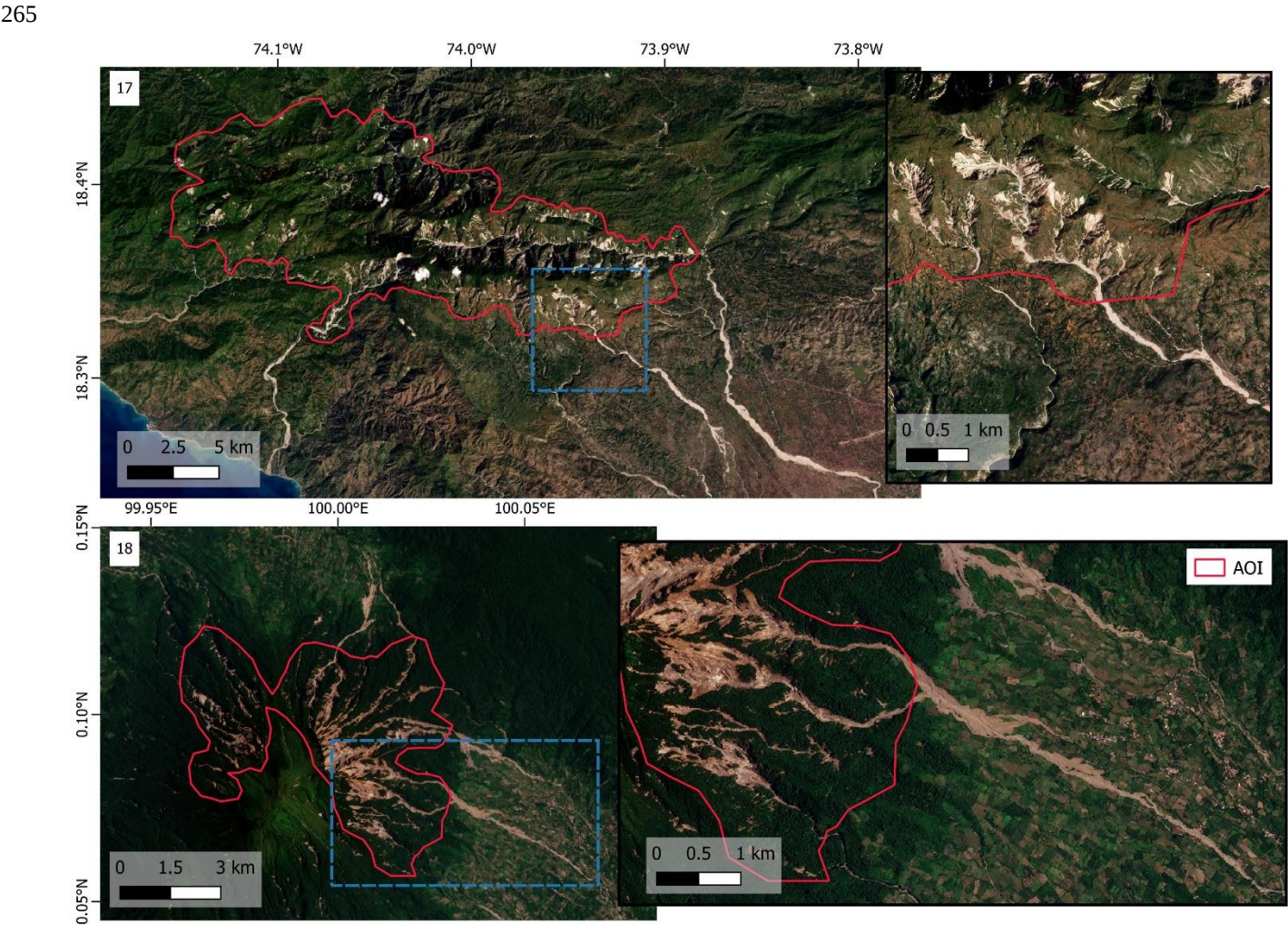
Figure 6. Two HTC reported to be triggered by earthquakes. The long runouts indicate highly mobile flows, suggesting the combined action of the seismic shaking with nearly coincident rainstorms. Top: overview (left) and zoom-in (right) of Pic Macaya, Haiti in 2021 (17), and bottom: Mt. Talakmau in Indonesia in 2022 (18). Blue-dashed rectangles indicate zoom-in areas. Satellite images: Planet Team, (2017).
