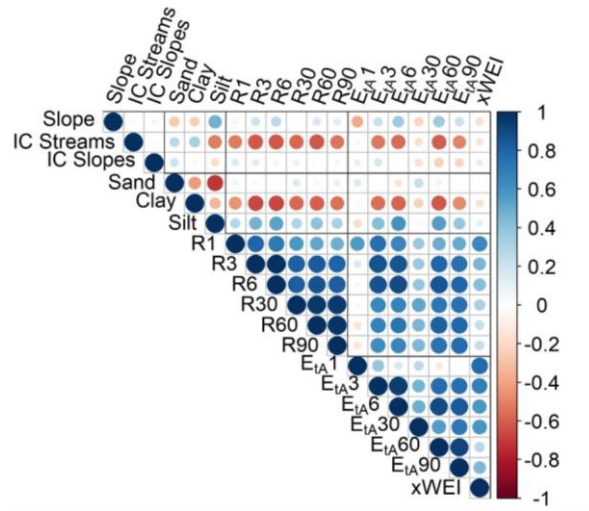
Figure 12. Correlation matrix for terrain and rainfall variables measured at the scale of the CHIRPS pixels. The darker lines divide the variables into groups: topography, sediment granulometry, rainfall intensity, and rainfall extremity. Ri variables refer to the accumulated rainfall the corresponding days, i, before the HTC. E IA i refers to the percentage of the extremity of the corresponding rainfall duration in i days, compared to the maximum recorded.
