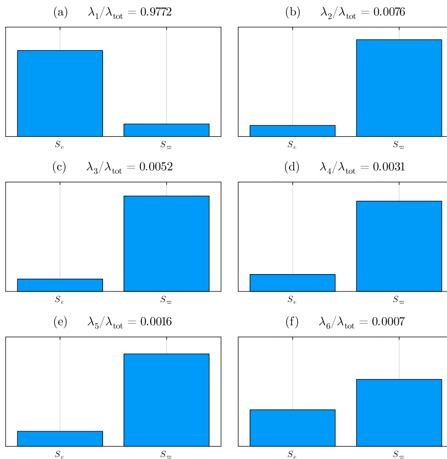
Figure 8. Magnitudes of the total Sobol index for eccentricity e and longitude of the perihelion \varpi . To obtain this figure, the values of obliquity and p\text{CO}_2 were held constant respectively at \varepsilon = 22.23^\circ and 5 \times 280 ppm.
