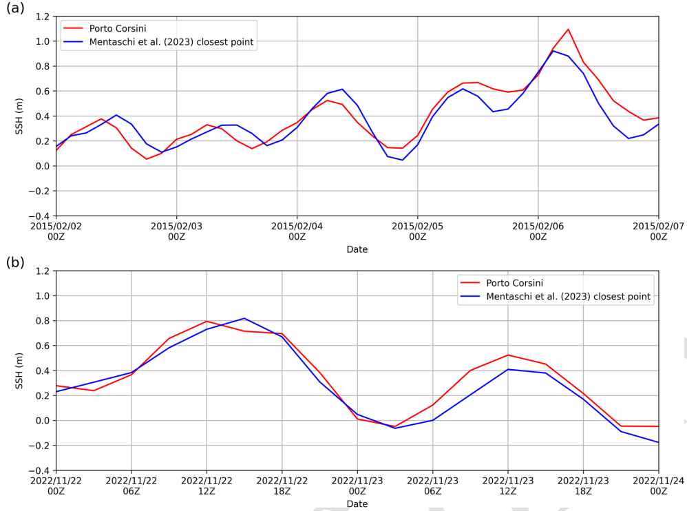
Figure 4. Comparison between the data of storm surge from Mentaschi et al. (2023) (blue line), with the filtered SSH data observed at the Porto Corsini station (red line) for the 2015 event (a) and 2022 event (b).
