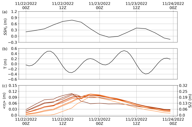
Figure 7. Boundary conditions for SSHs (m) (a), T (m) (b), and both \langle \eta \rangle (m) and S/2 (m) (c) during the 2022 event. In panel (c), \langle \eta \rangle and S are proportional; the left y-axis corresponds to \langle \eta \rangle , while the right y-axis represents S/2 , allowing both quantities to be conveyed by a single curve. Darker (lighter) colors indicate a more meridional (zonal) coastline orientation.
