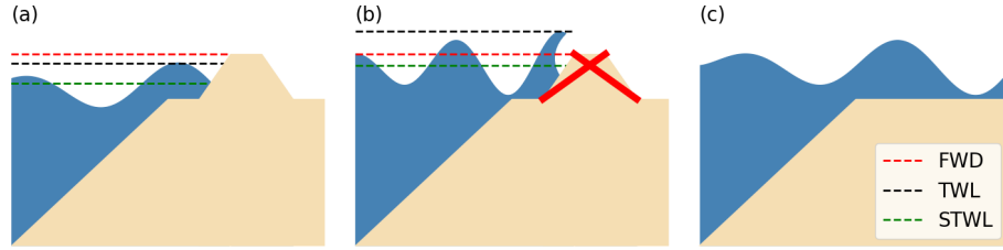
Figure 2. Schematic representation of coastal protections in LISFLOOD-FP. (a) protective action when TWL < FWD . (b) failure for TWL > FWD . (c) free flood propagation upon protection failure. Red line represents the FWD, black line the TWL and green line the STWL.
