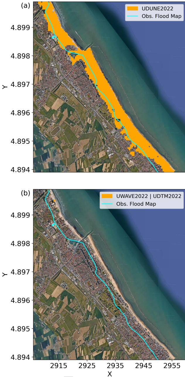
Figure 12. LISFLOOD-FP uncertainty associated with dunes UDUNE2022 (a), waves UWAVE2022 and DTM UDTM2022 (b). Orange areas represent the uncertainty, given by the difference of flooded areas in the simulations. The cyan line corresponds to the limits of the observational flood map. ©Google Maps.
