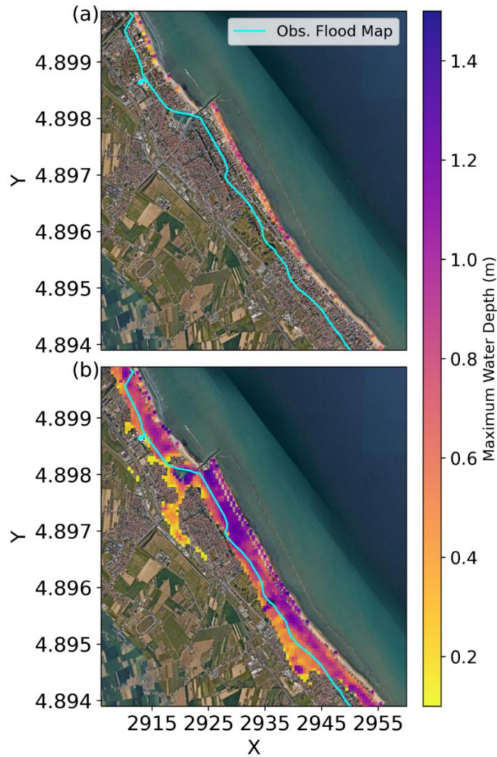
Figure 10: Waves' contribution to flood: simulation E2015DWL which does not consider the contribution of swash (a) and simulation E2015TWL which considers the full extent of TWL as contributing to both dune failure and water supply (b). © Google Maps
