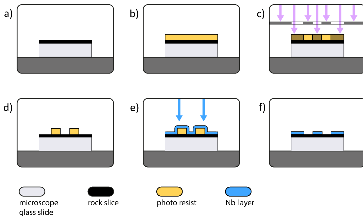
Figure 4. Schematic of the application of marker structures on a rock sample, by means of UV-lithography and sputter coating. a) sideview of a typical MMT sample consisting of a tiny drill core from a thin section. b) application of photo resist on the sample. c) a mask with the desired structures is placed above the sample. UV-light shines through the transparent parts of the mask and breaks down the exposed photo resist. d) the exposed photo resist is easily removed after developing. e) A Nb-sputter coating is applied on top of the sample. f) lift-off, the sample is placed in acetone for 30 minutes to remove all the unwanted sputter coating. The desired structures are left in Nb on top of the sample.
