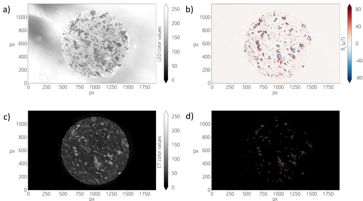
Figure 2. Example images of the data used in Micromagnetic Tomography. One QDM pixel equals 1.20 \mu\text{m} and the field of view equals 2.30 \text{ mm} \times 1.44 \text{ mm} . All images are scaled to figure a). a) and b) are data obtained with the QDM. a) is a LED micrograph of the sample. b) is a vertical component ( B_z -) map of the magnetic surface flux. c) is density-based data obtained with the nanoCT scanner. d) is magnetic grain data extracted from the CT data with the use of 3D-visualization and analysis software.
