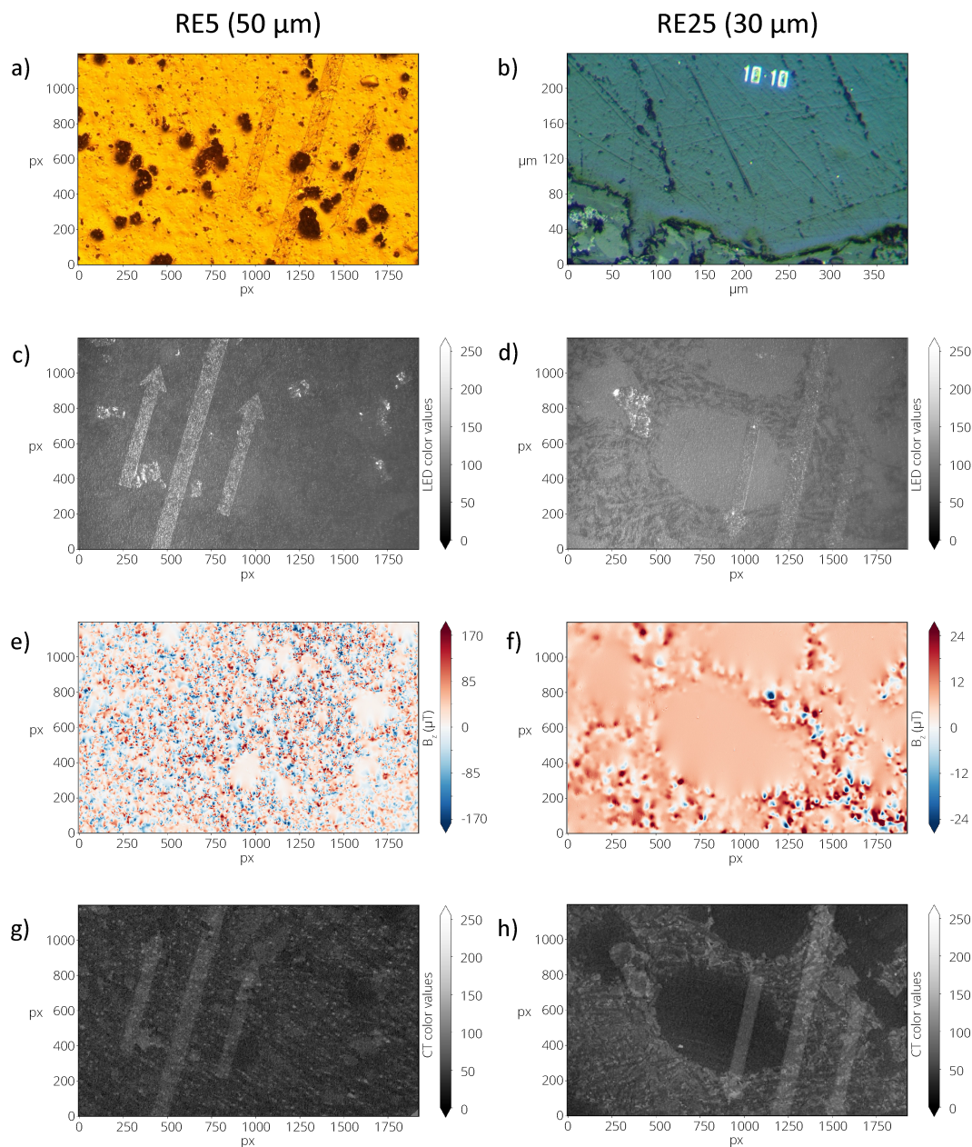
Figure 5. Images of the applied marker structures. One QDM pixel equals 1.20 \mu\text{m} and the field of view equals 2.30 \text{ mm} \times 1.44 \text{ mm} . All images except b) are scaled to figures c) and d). a) is a micrograph of the applied photo resist, already exposed to UV-light. The large marker structures of two arrows and a line are visible in the photo resist on the sample surface. b) SEM image of the smallest applied marker structures on the sample surface, after lift-off. The white dots are 3 \mu\text{m} in size, the white numbers are 20 \mu\text{m} tall. c) and d) are LED micrographs of the applied markers on the sample surface as observed under the QDM. e) and f) are the B_z -maps of the magnetic surface scans measured with the QDM. The marker structures do not fluoresce under laser light, meaning that they do not interfere with the magnetic signal of the sample. g) and h) are the density-based data obtained with the nanoCT scanner. Only the larger marker structures are visible.
