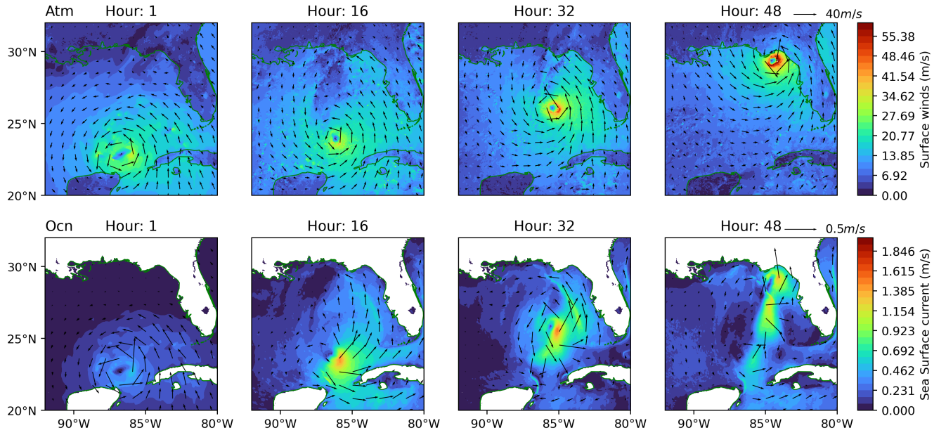
Figure 9. 2D time evolution snapshots of surface winds and sea surface currents for hurricane Helene with an idealized ocean. Black arrows correspond to localized velocity vectors.
