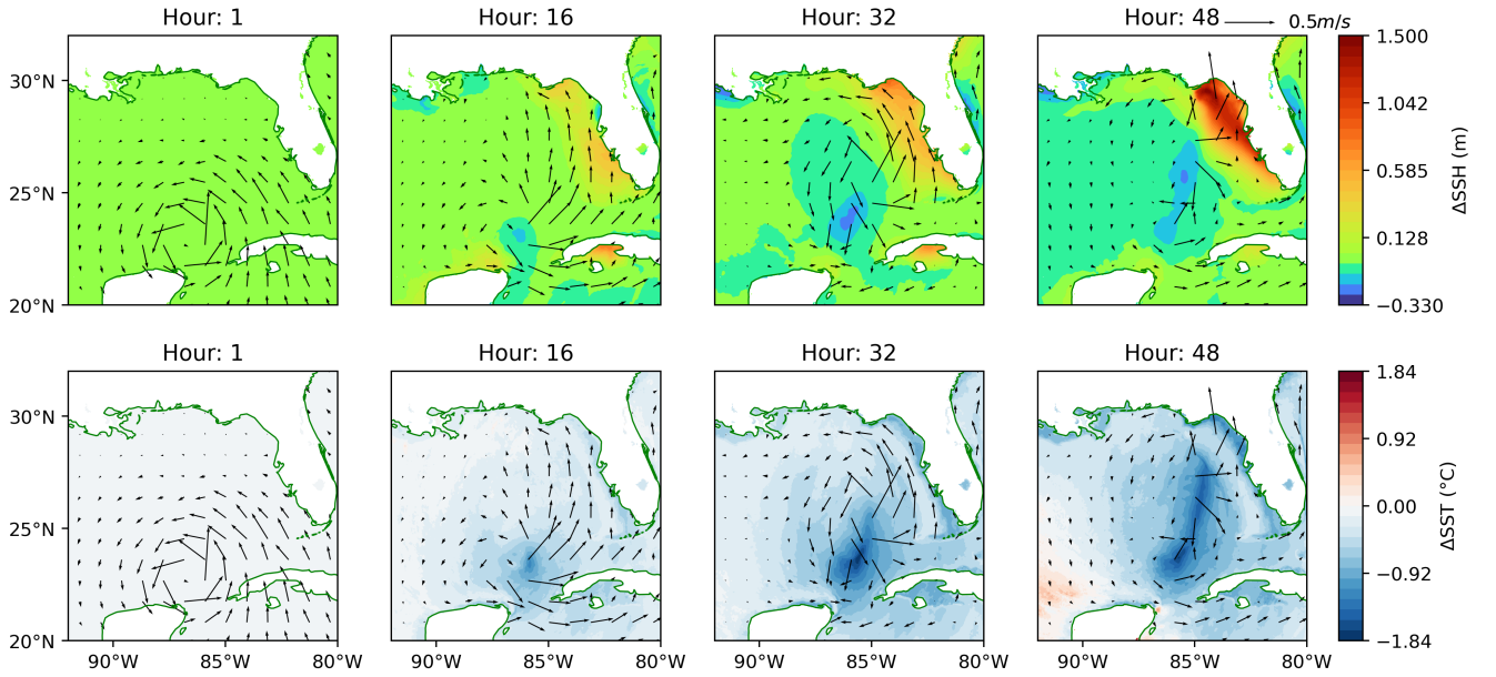
Figure 10. 2D time evolution snapshots of sea surface height (top) and temperature (bottom) compared to their initial values for hurricane Helene with an idealized ocean. Black arrows correspond to localized velocity vectors.
